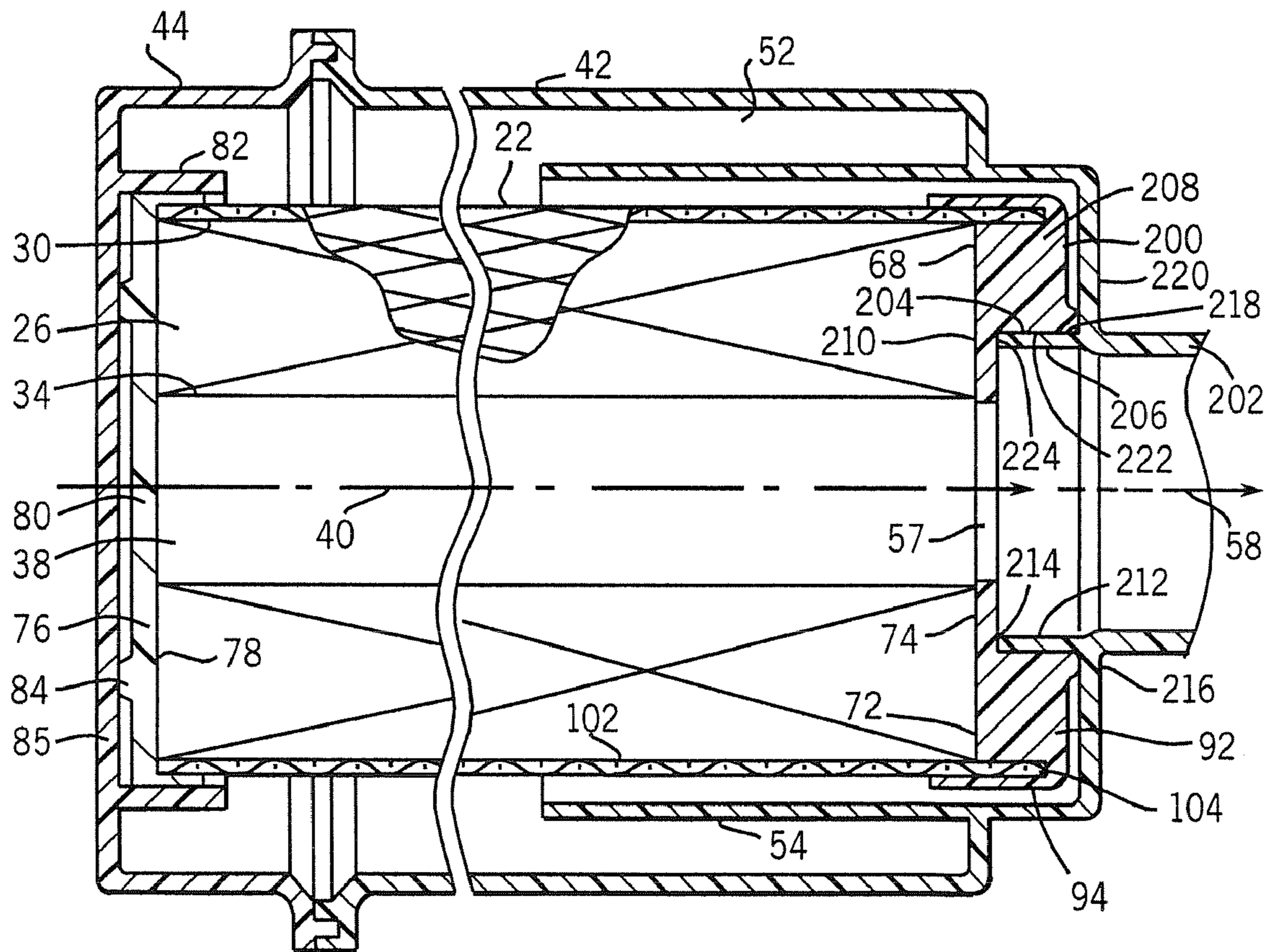
FIG. 7 PRIOR ART
