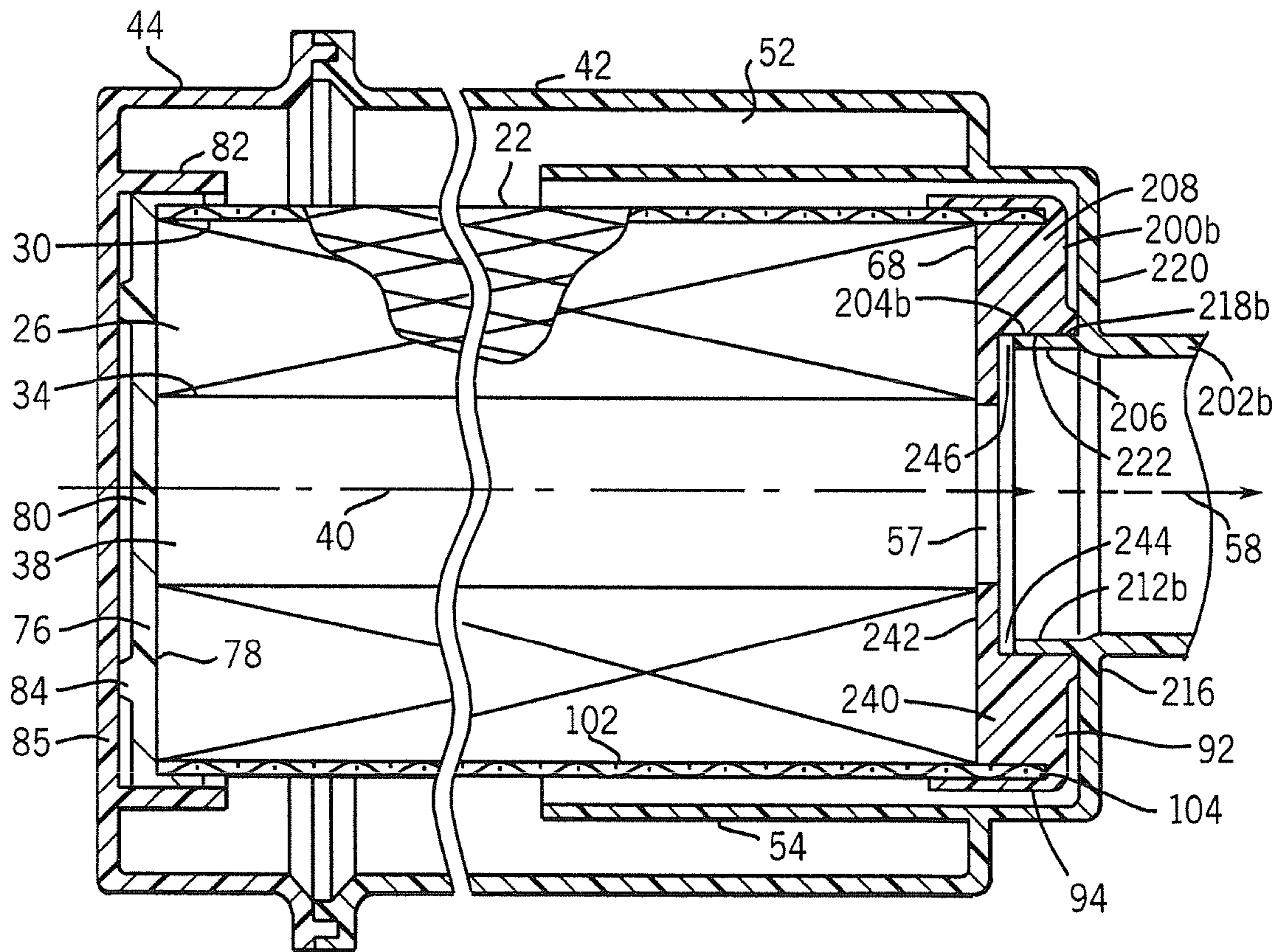
FIG. 12 PRIOR ART
