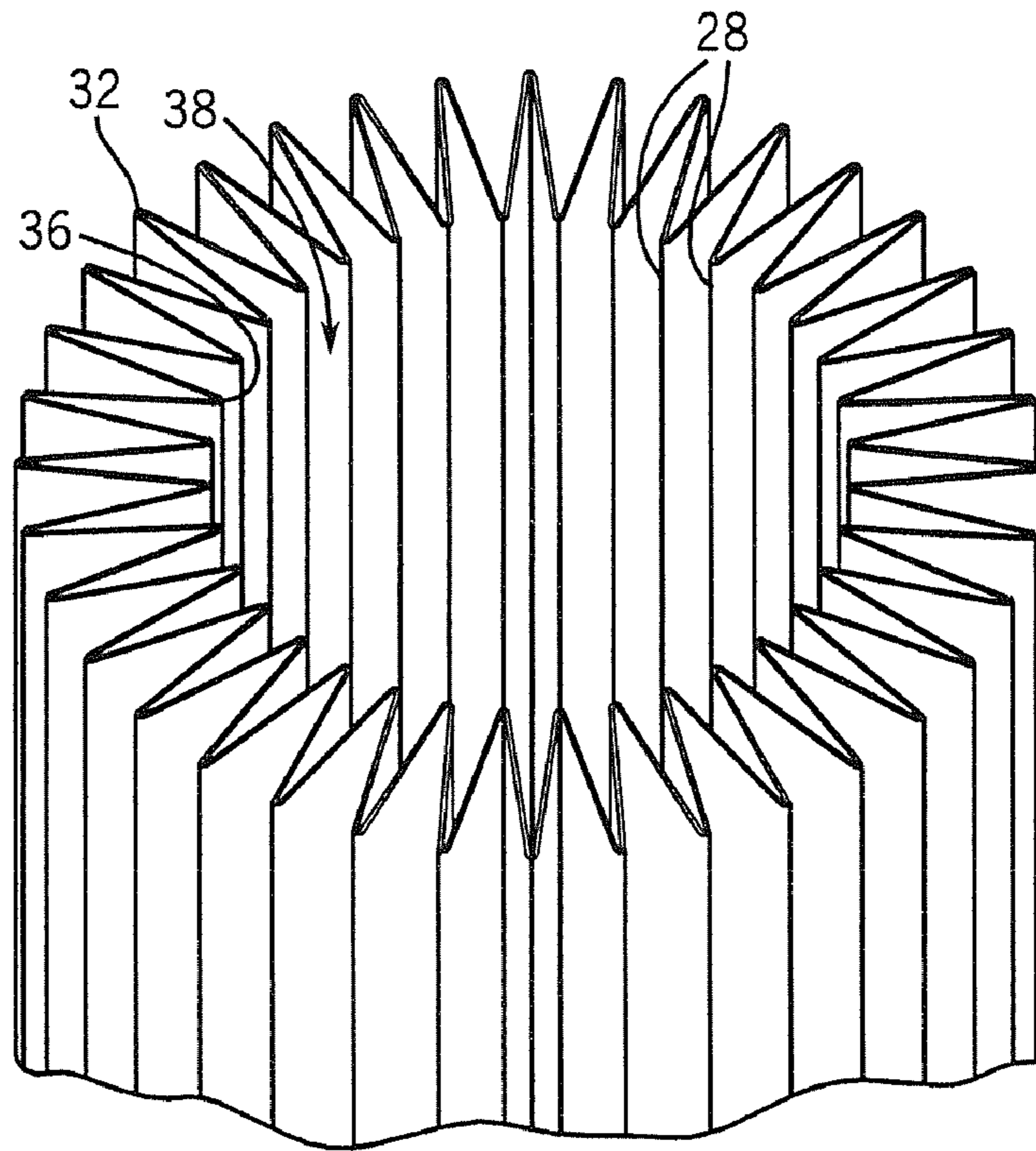
FIG. 8 PRIOR ART
