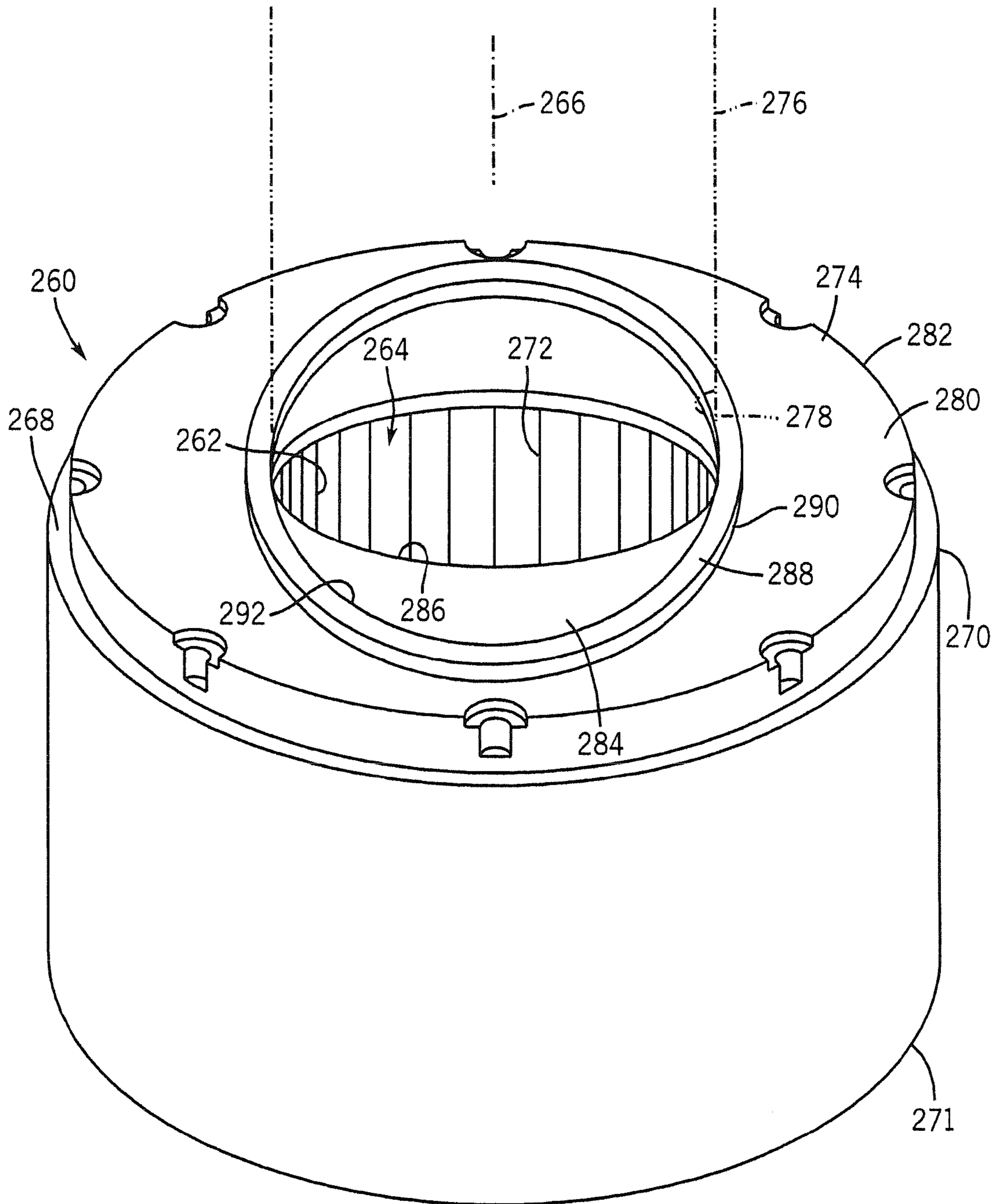
FIG. 14 PRIOR ART
