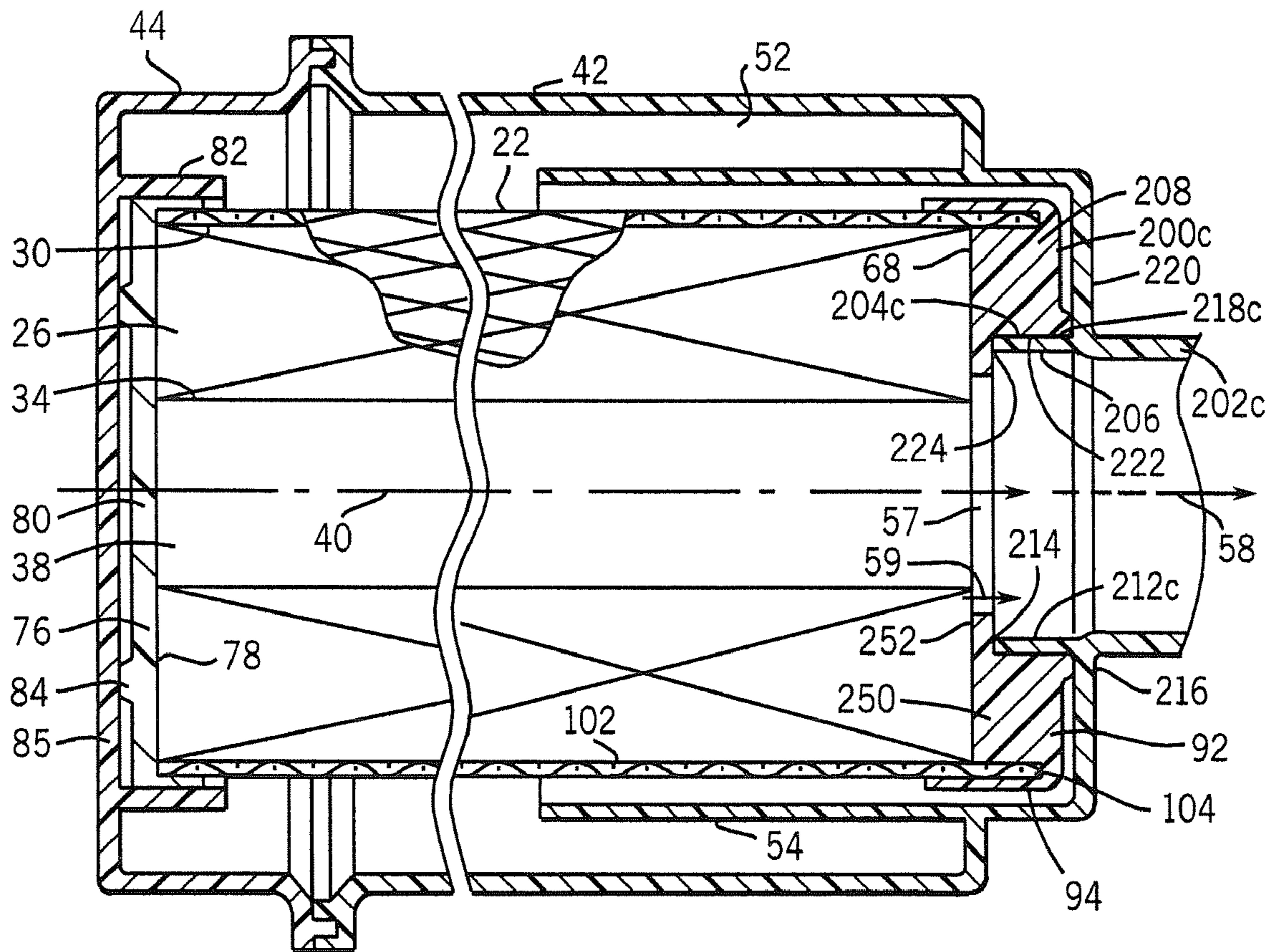
FIG. 13 PRIOR ART
