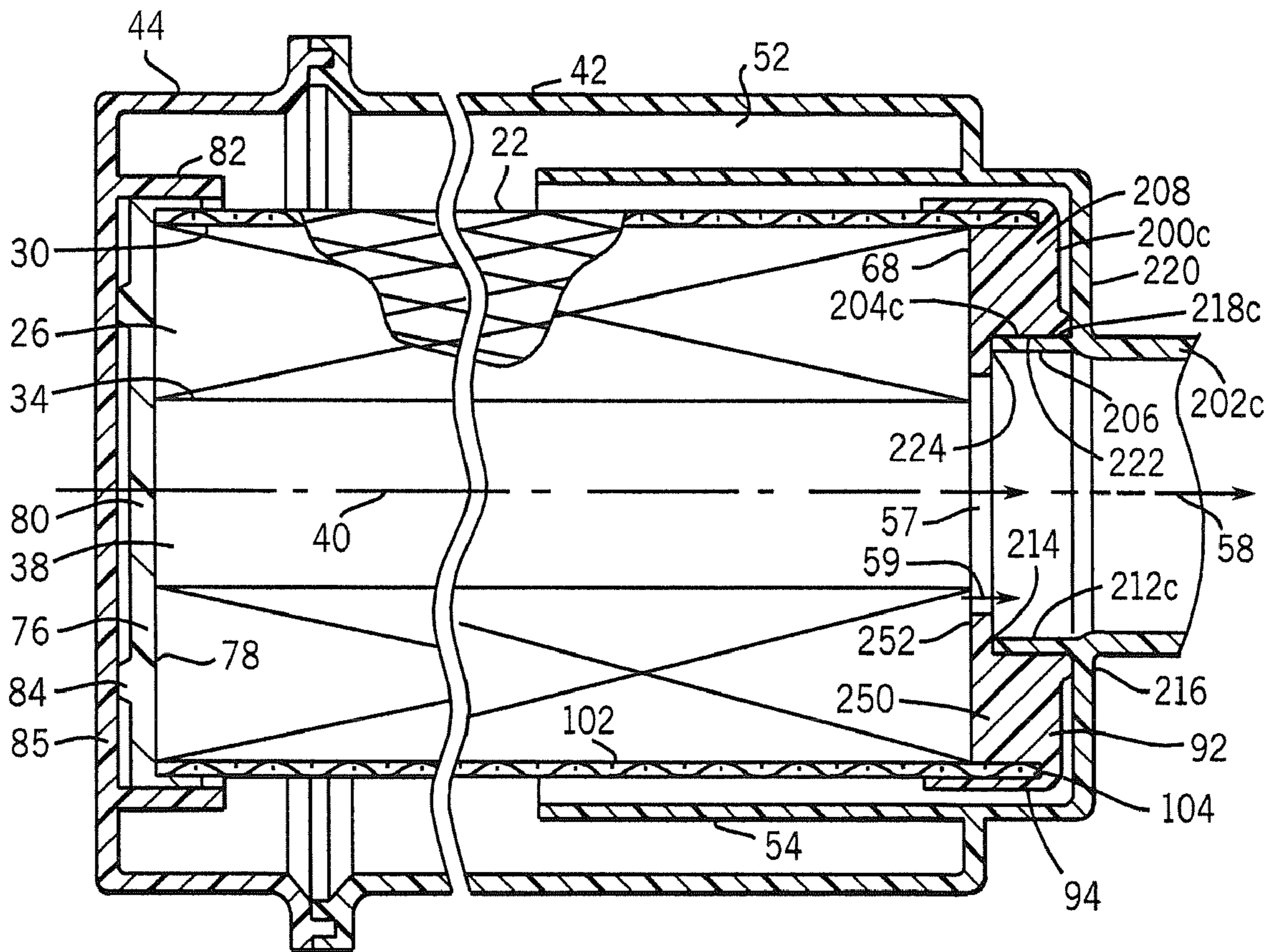
FIG. 13 PRIOR ART
