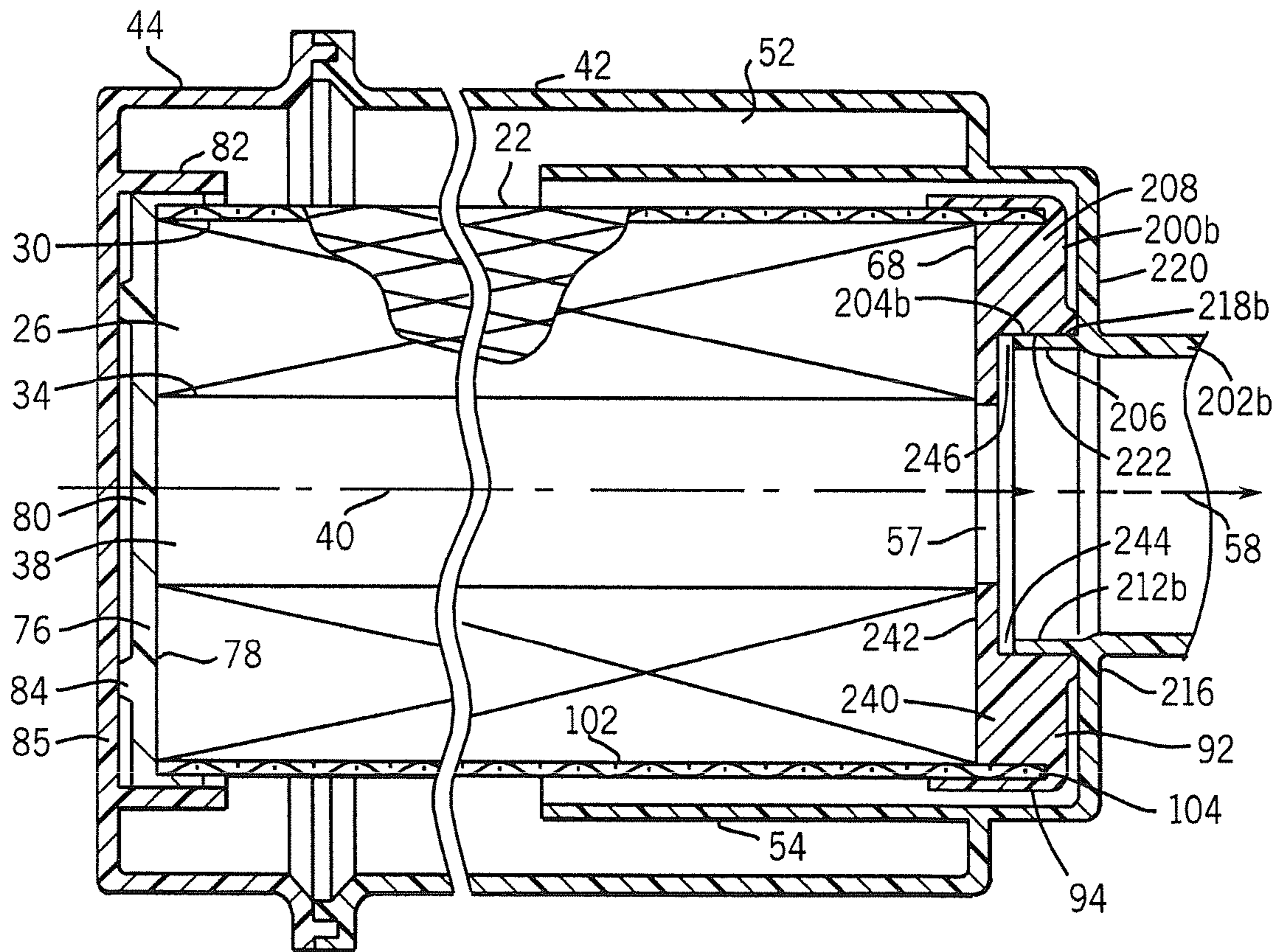
FIG. 12 PRIOR ART
