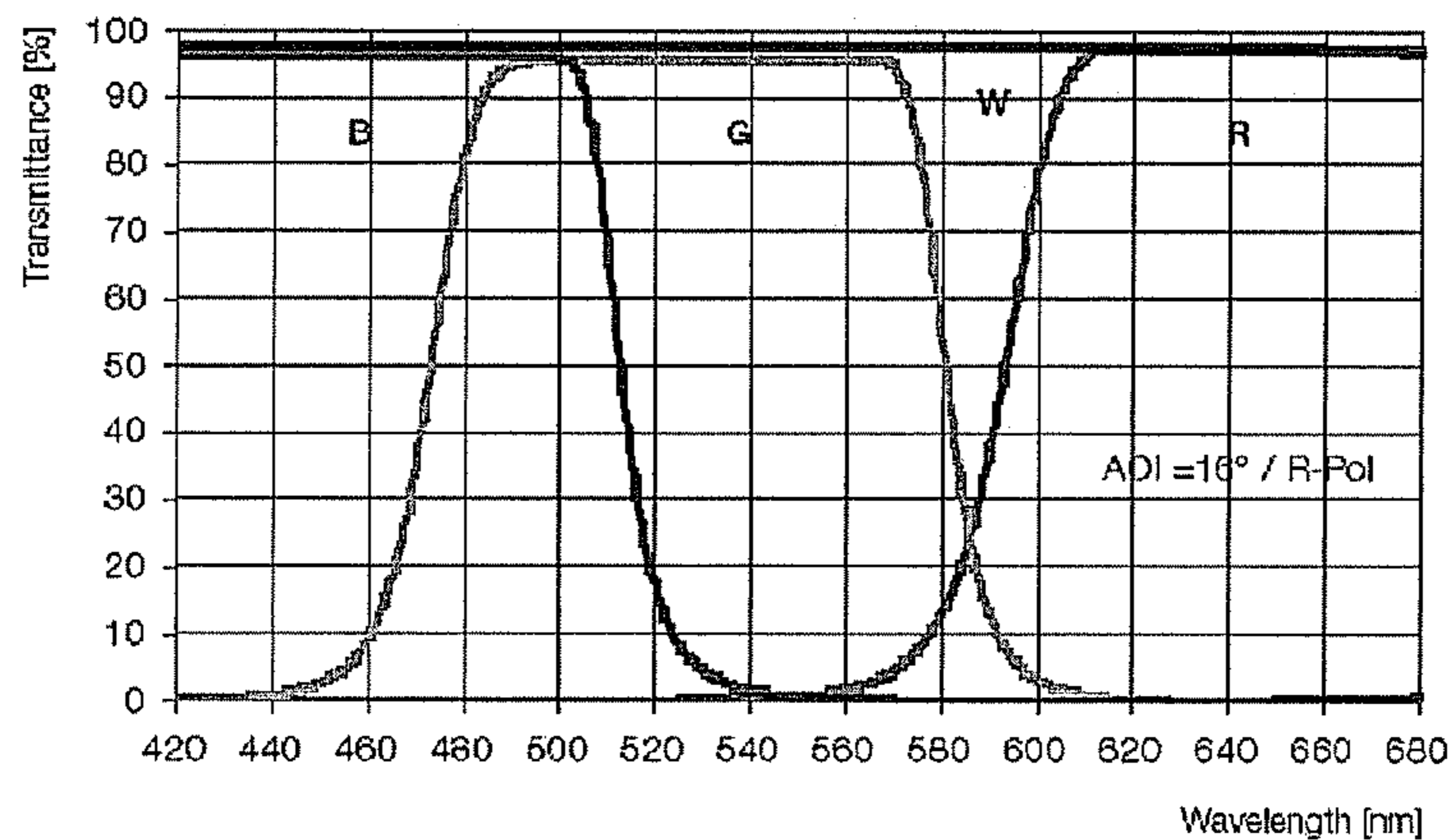
Example for spectral performance of blue/green/red/white filters
