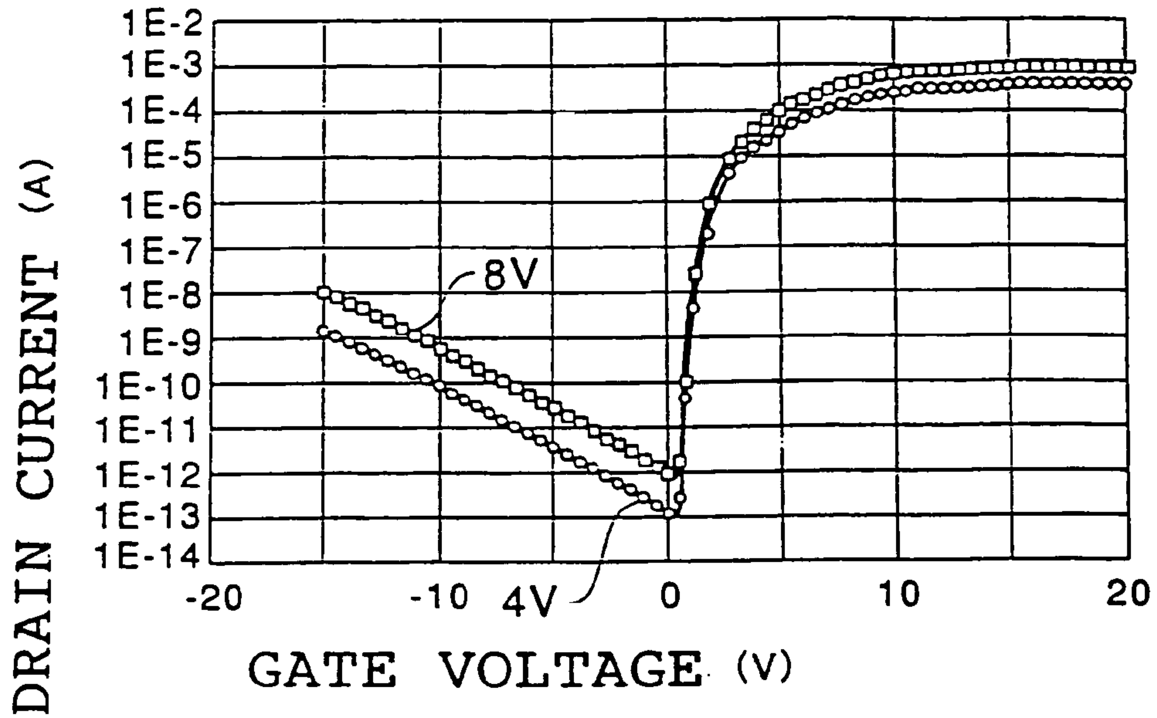
FIG. 11 AMPERE/VOLT CHARACTERISTICS N CHANNEL TYPE TFT
