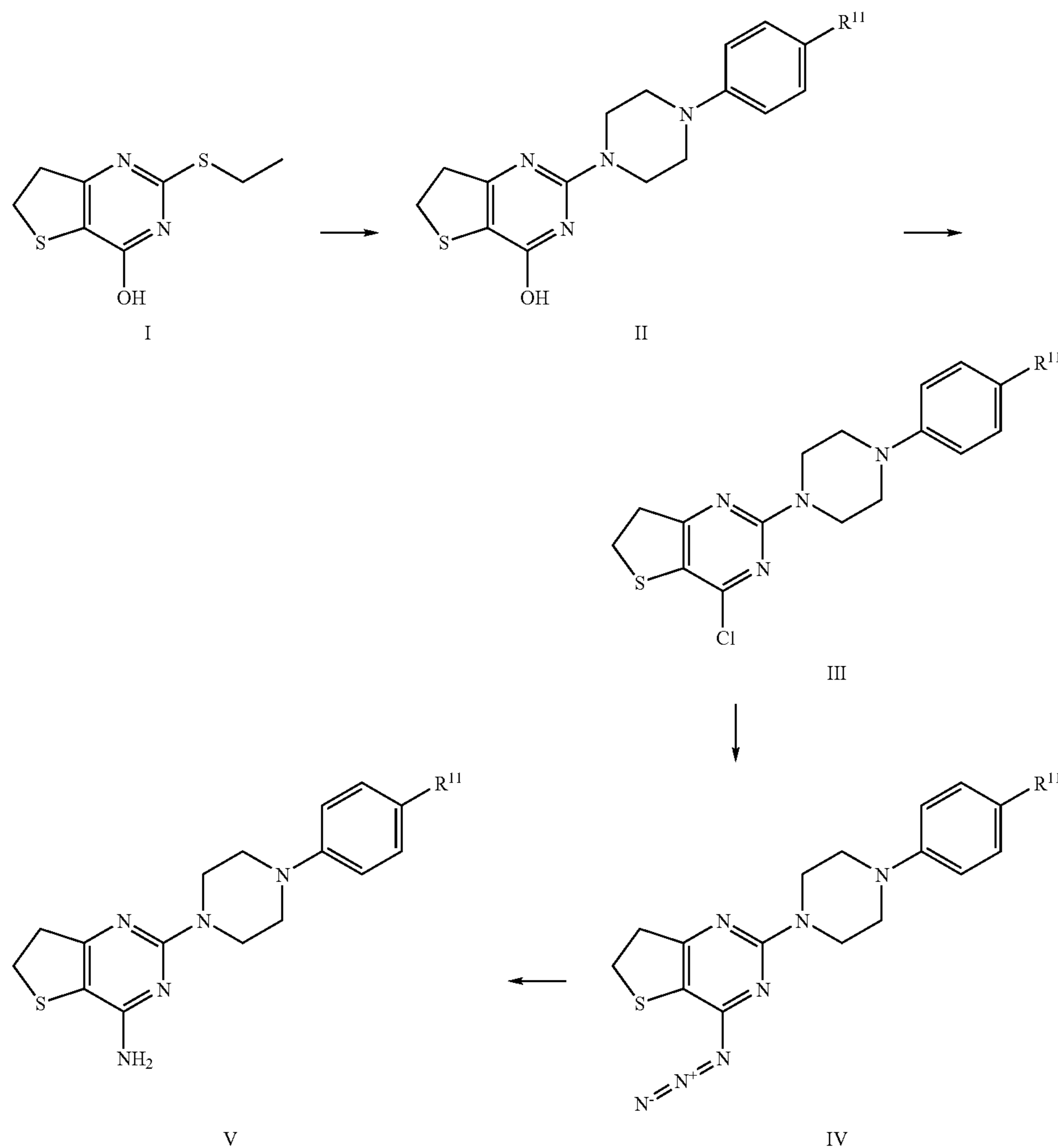
Scheme 13
