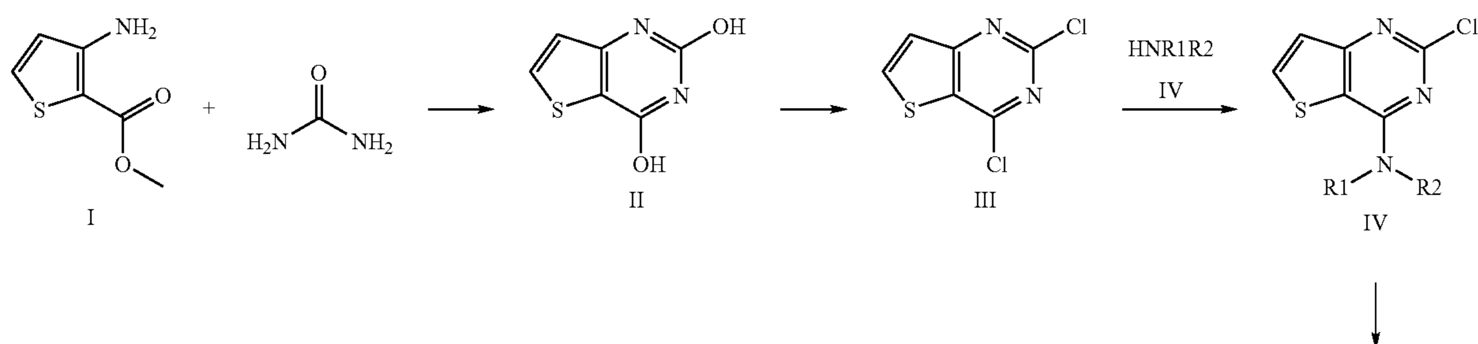
Scheme 14
