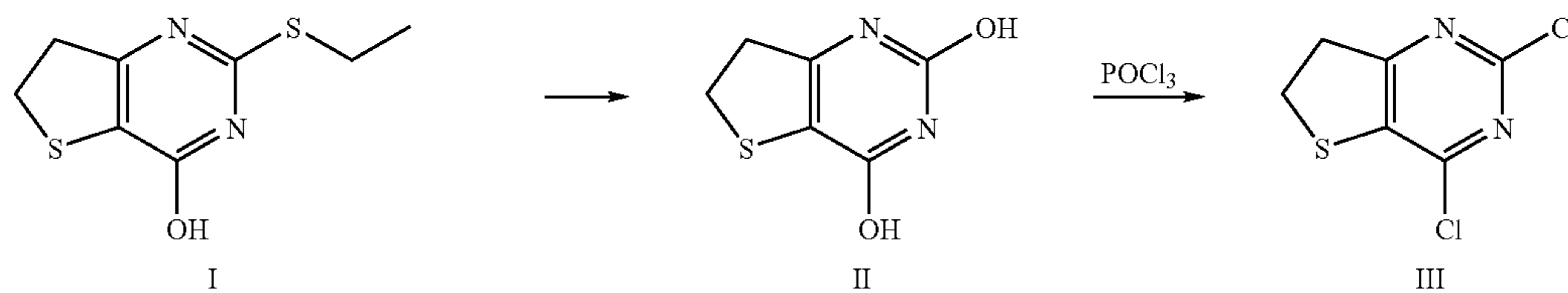
Scheme 10
