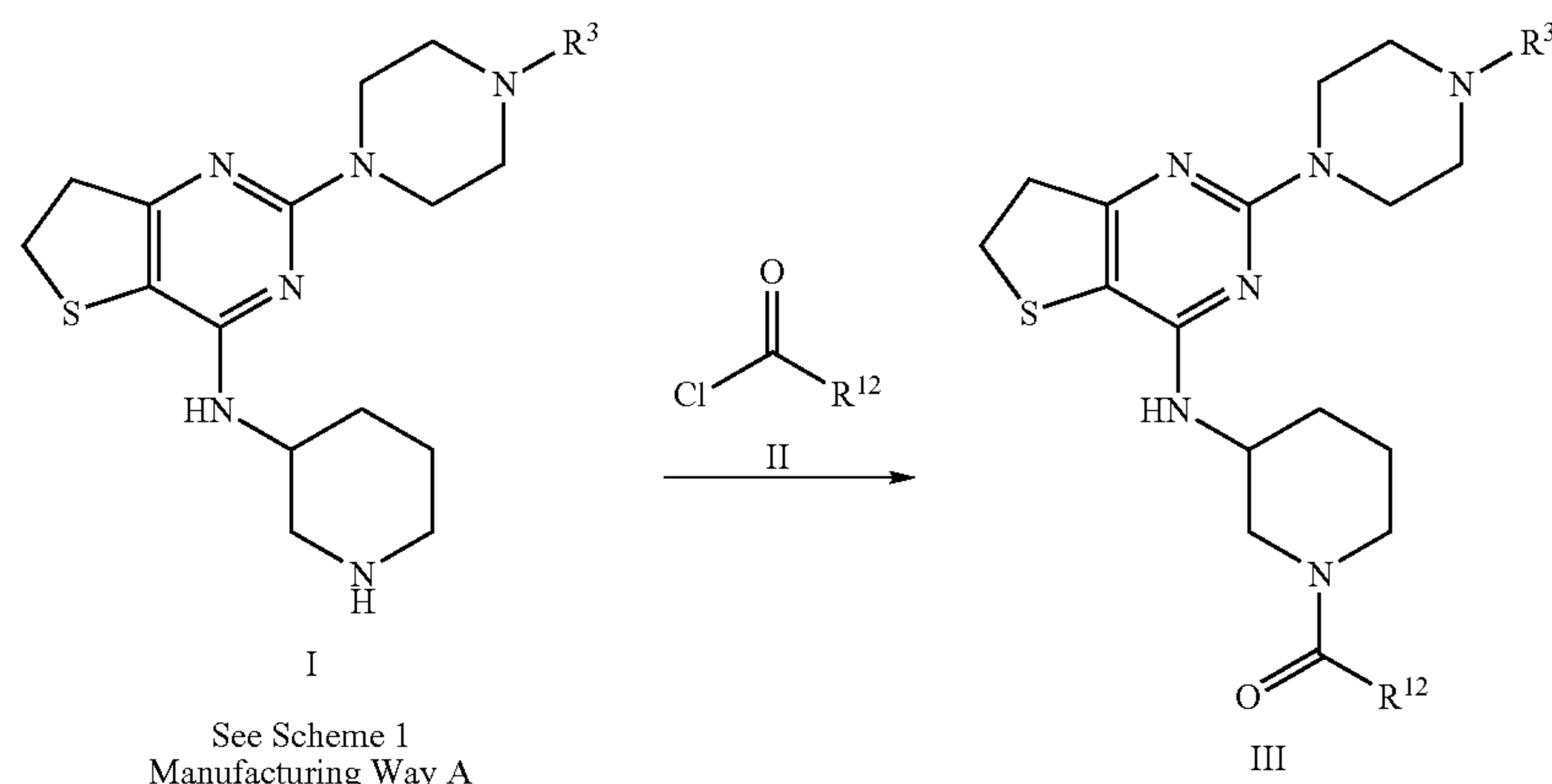
Scheme 11
