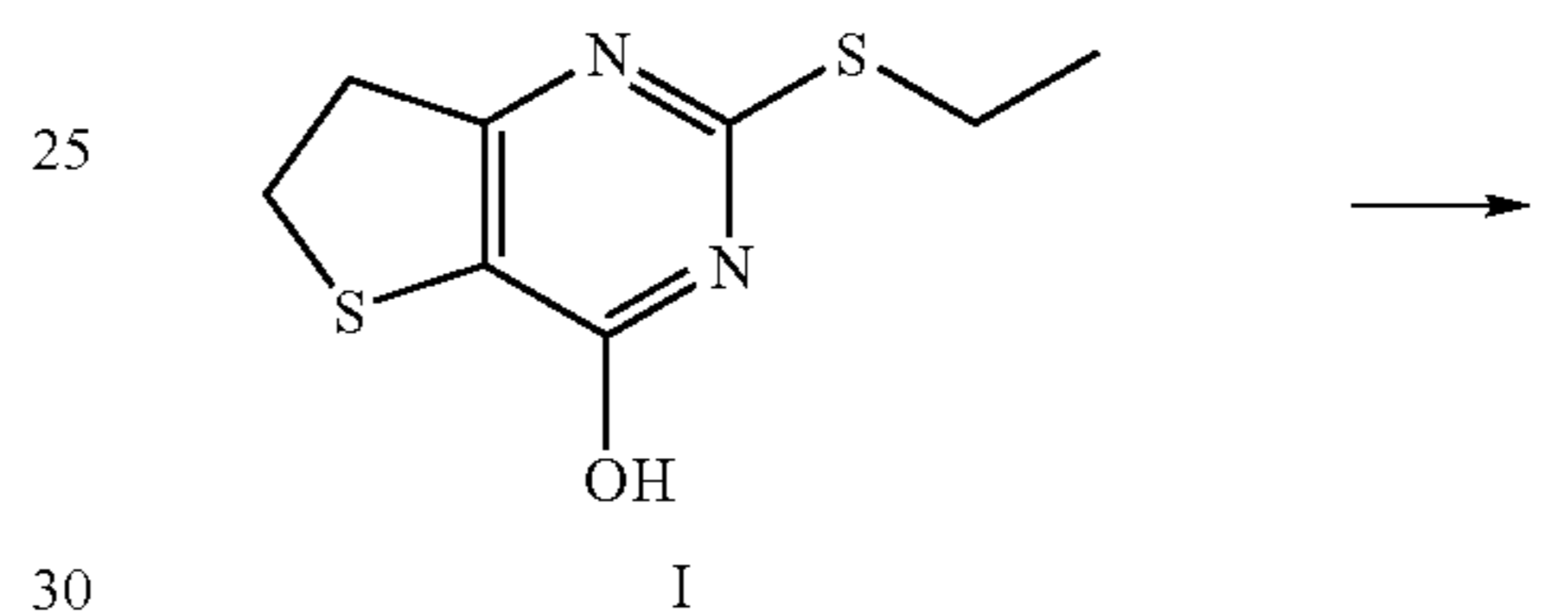
Scheme 6
