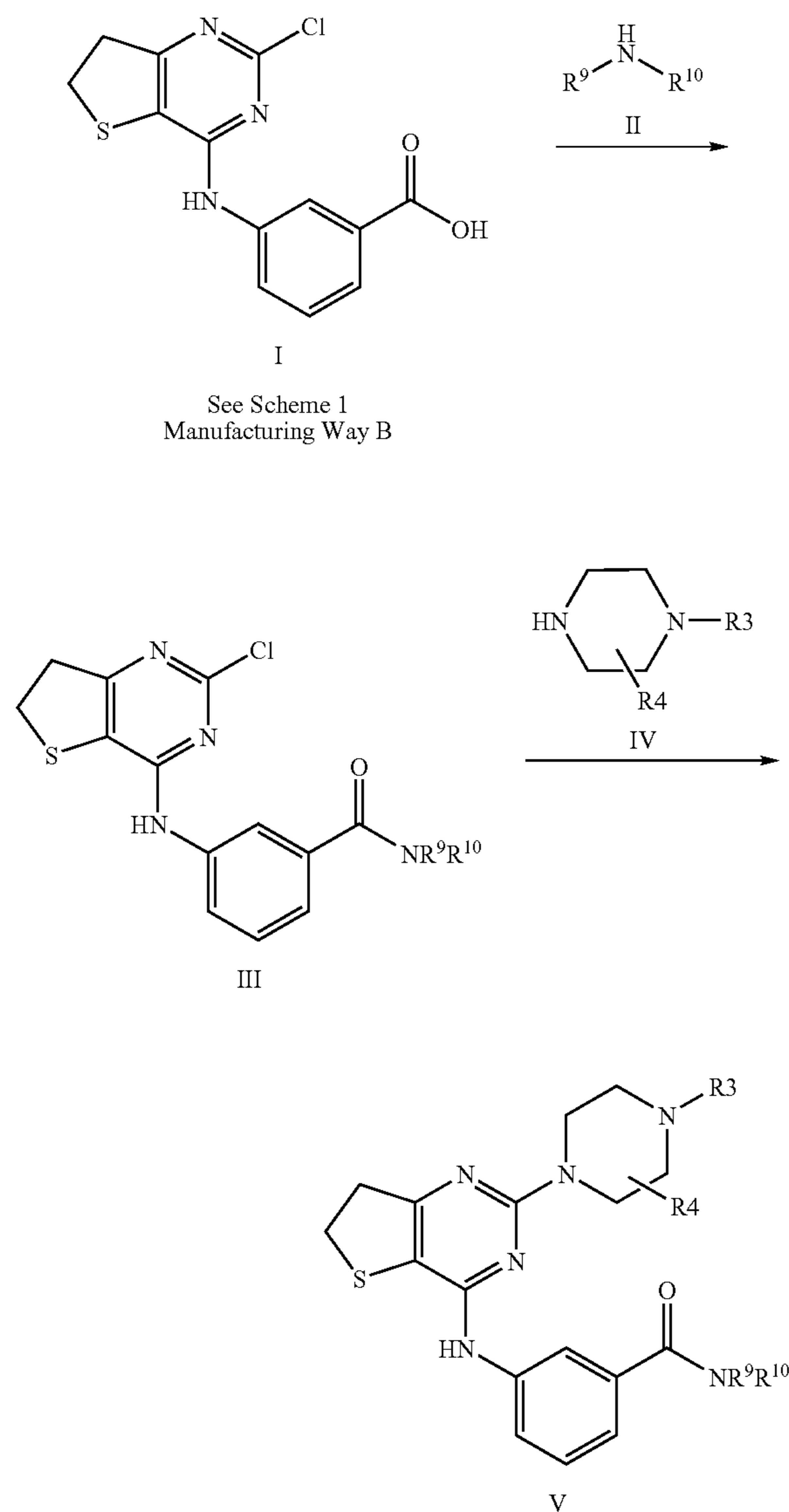
Scheme 12
