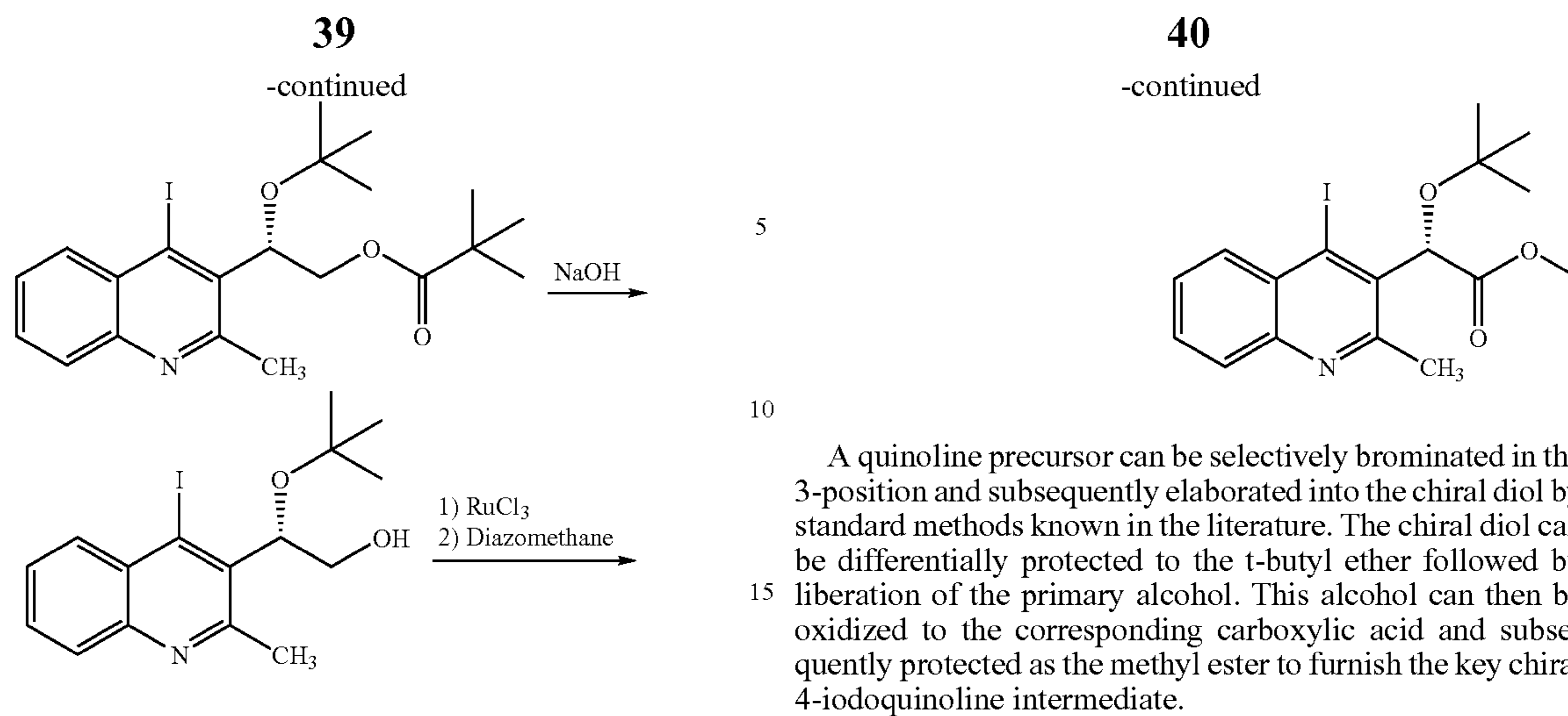
Scheme 4: Alternate synthesis of quinoline scaffold
