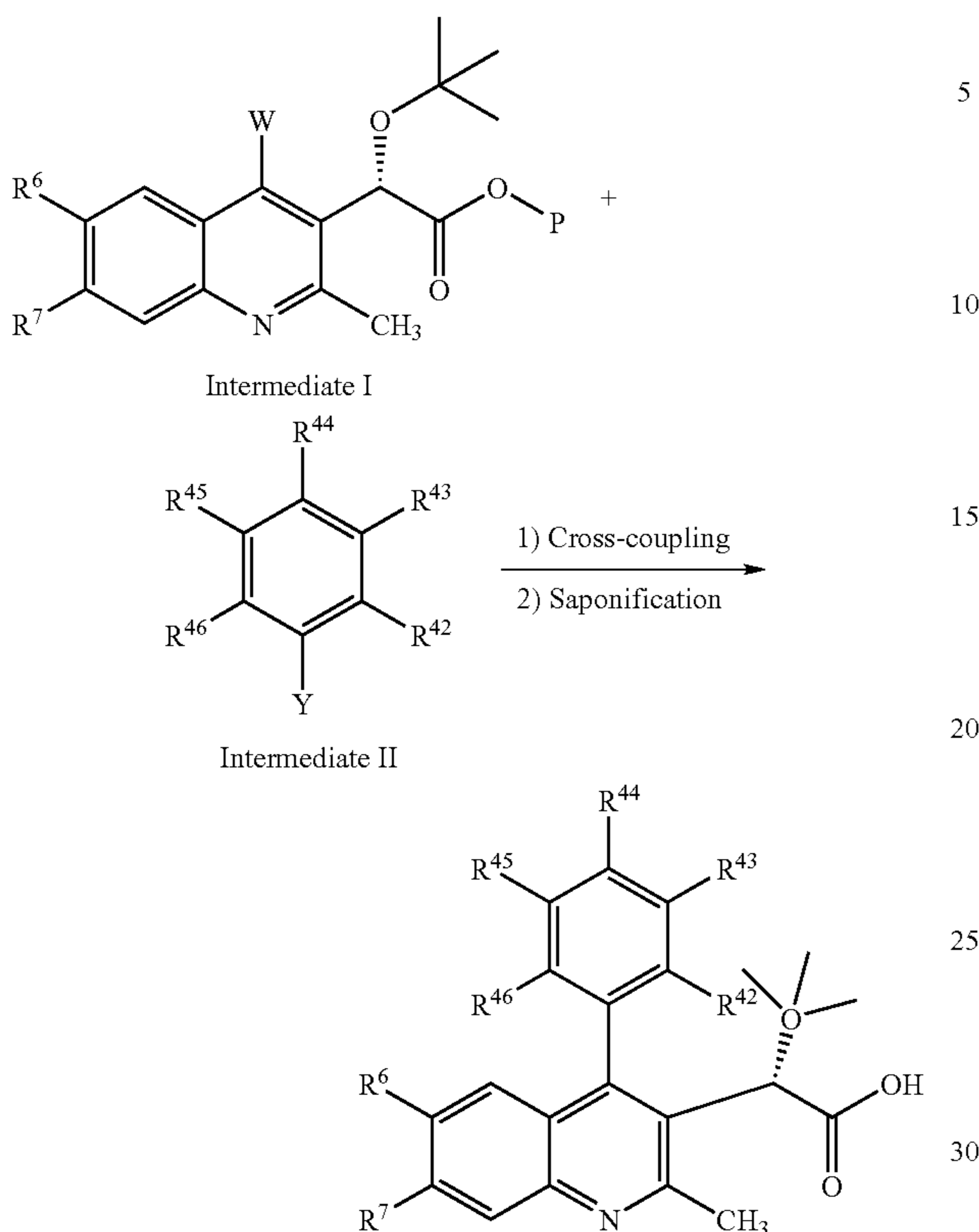
Scheme 1: Assembly of inhibitors
