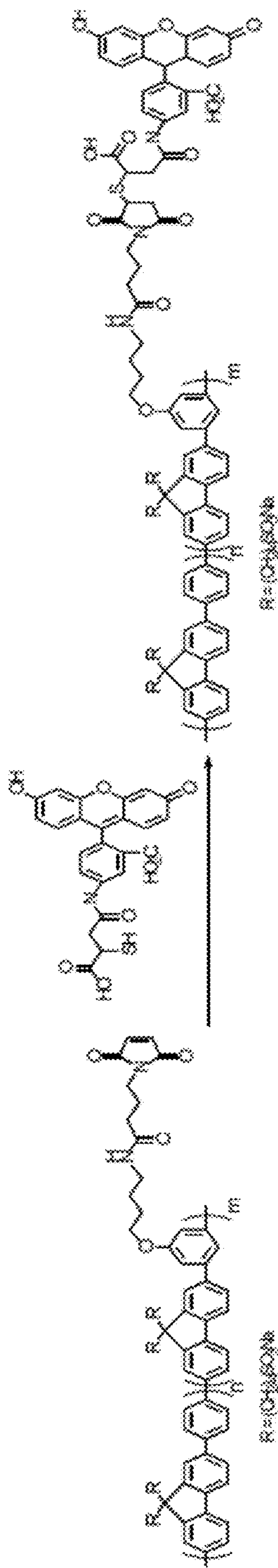
Maleimide-functionalized polymer
