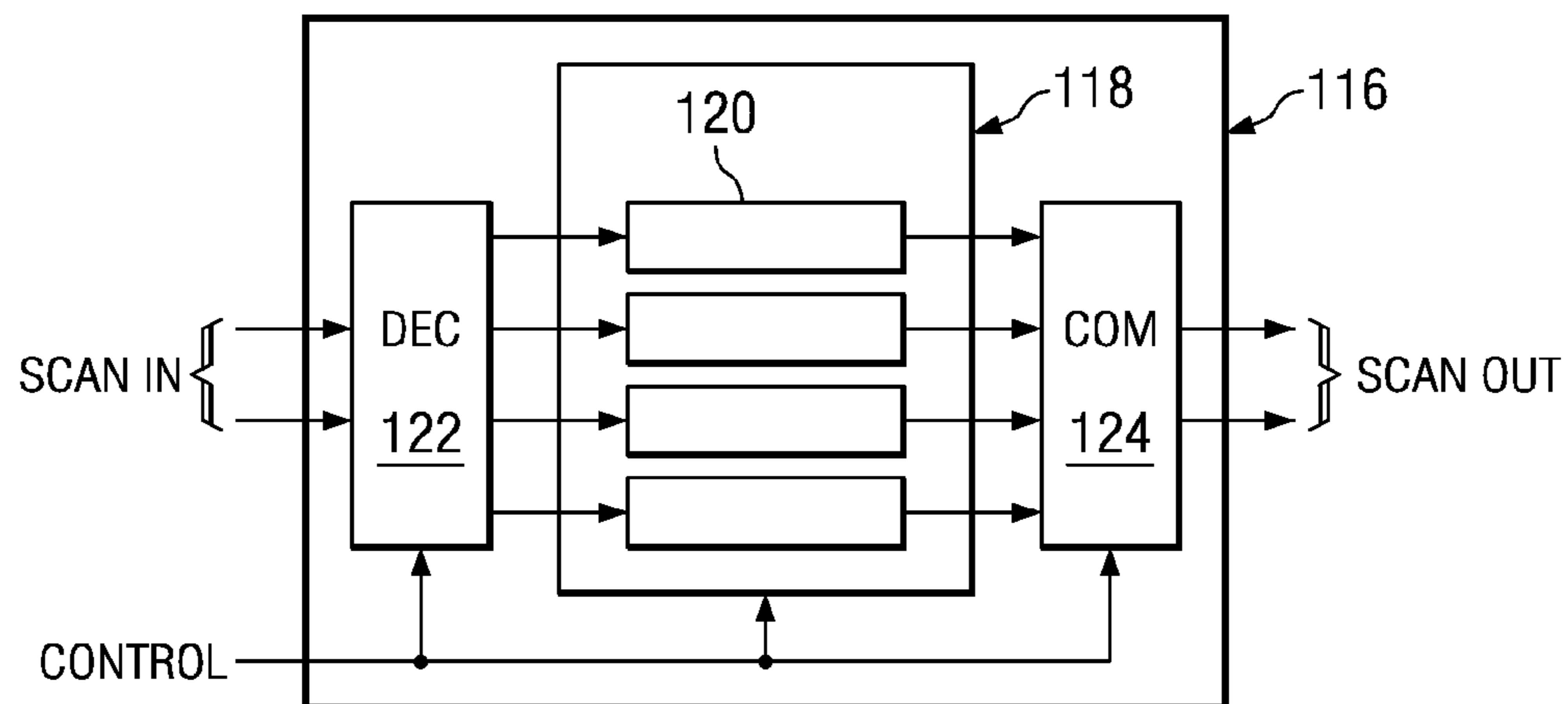
FIG. 1C (PRIOR ART)
