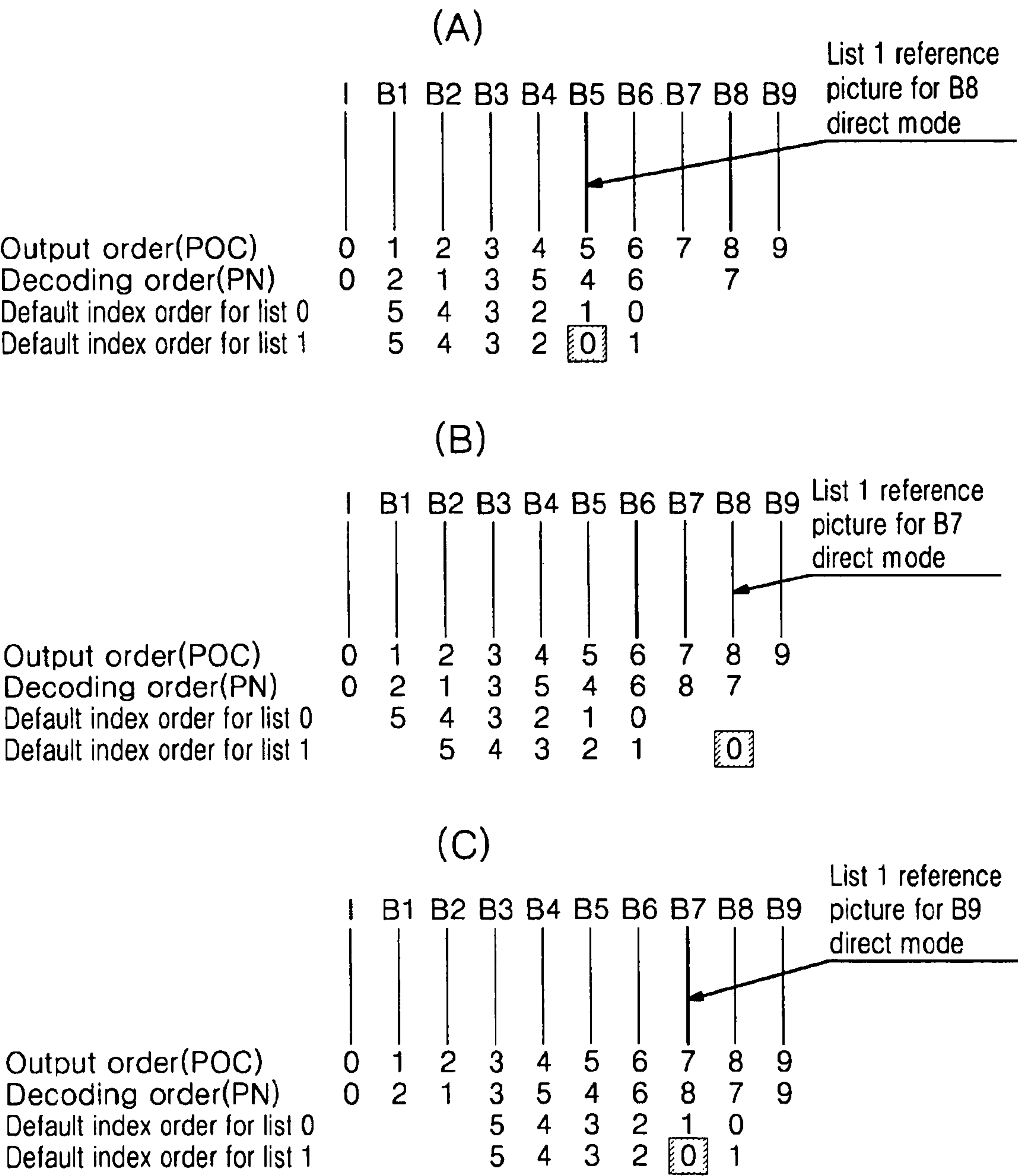
FIG. 2 (Related Art)
