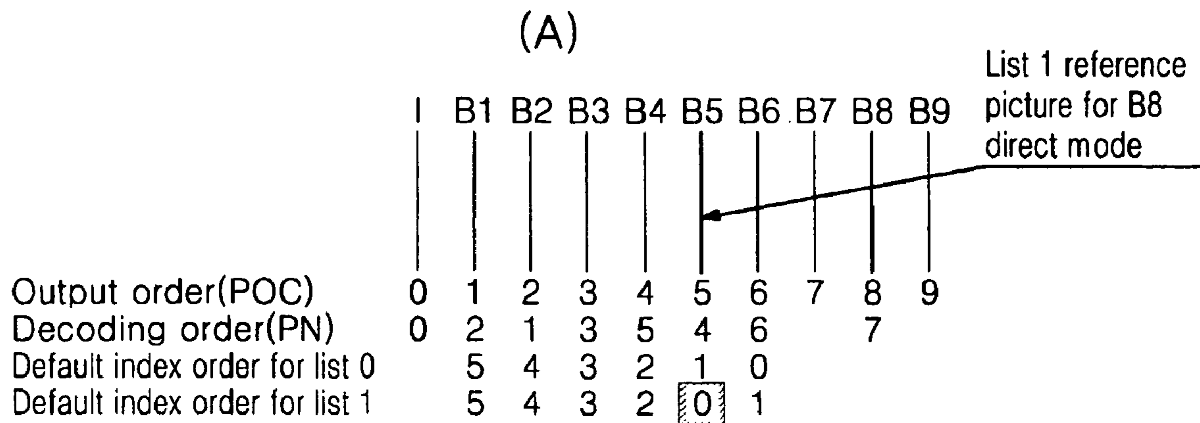
FIG. 2 (Related Art)
