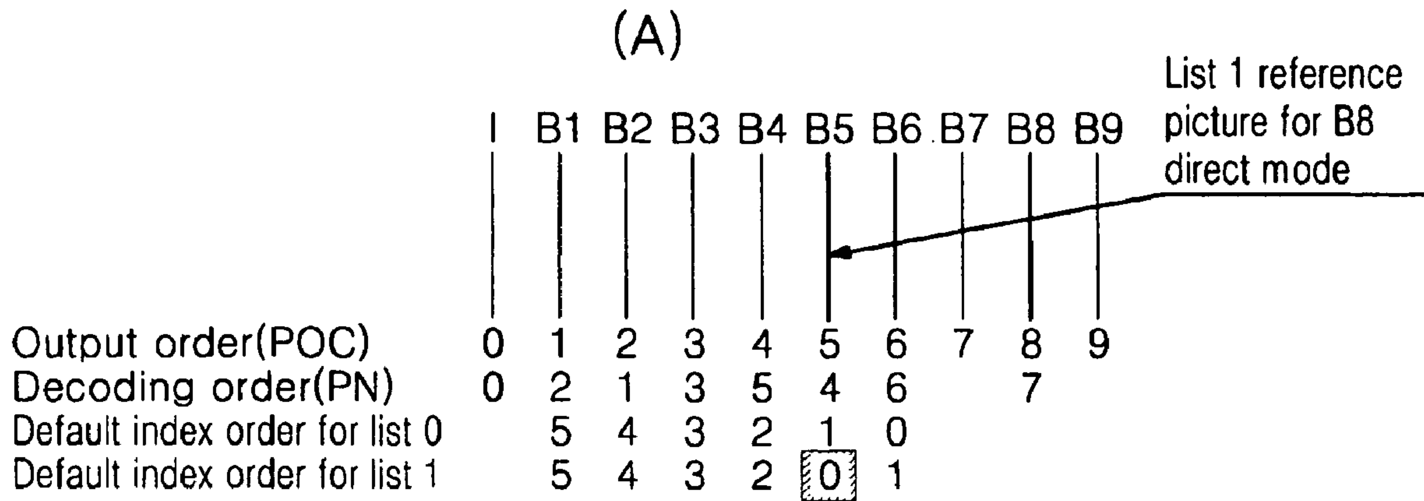
FIG. 2 (Related Art)
