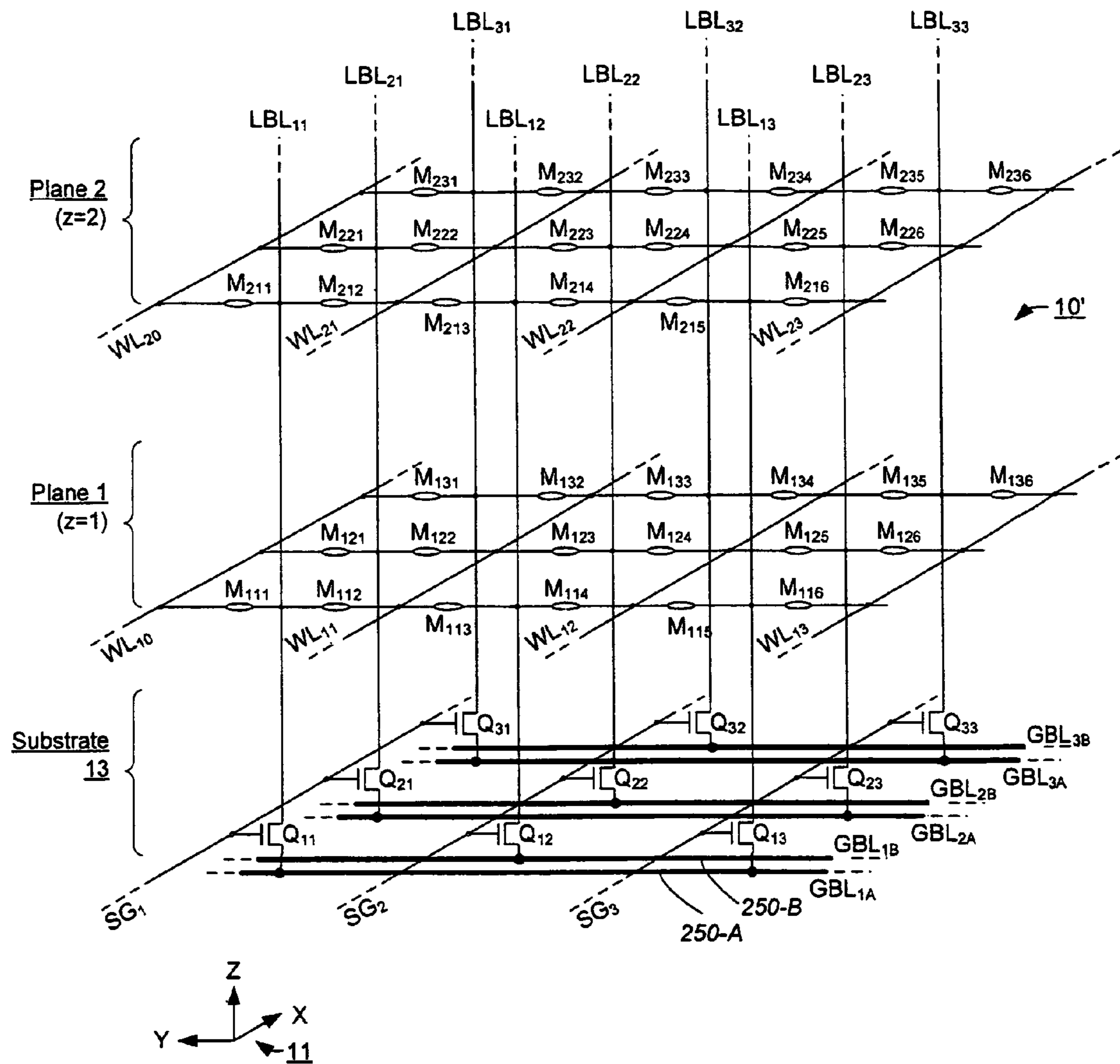
Double-Global-Bit-line Structure
