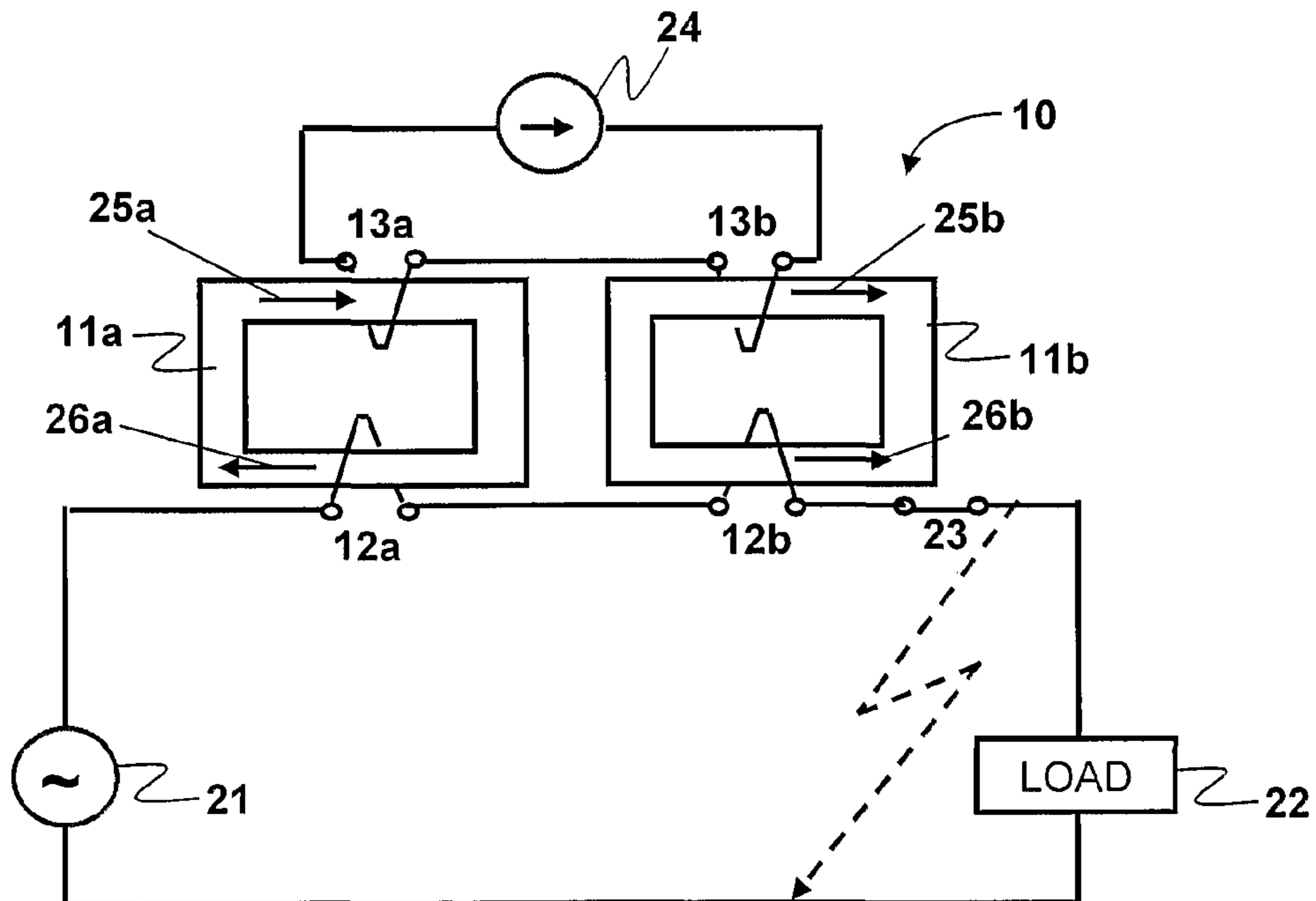
FIG. 1 (PRIOR ART)
