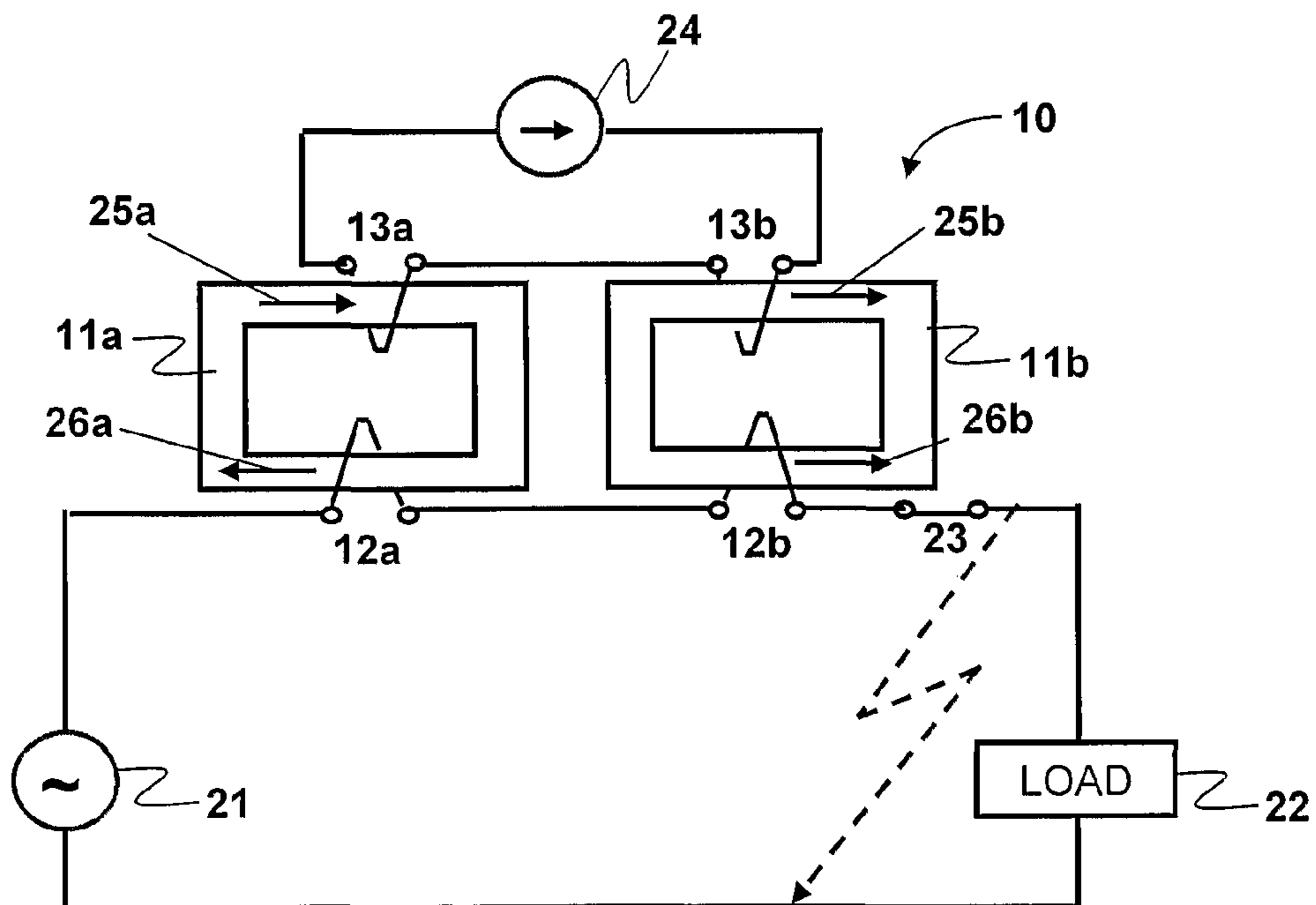
FIG. 1 (PRIOR ART)
