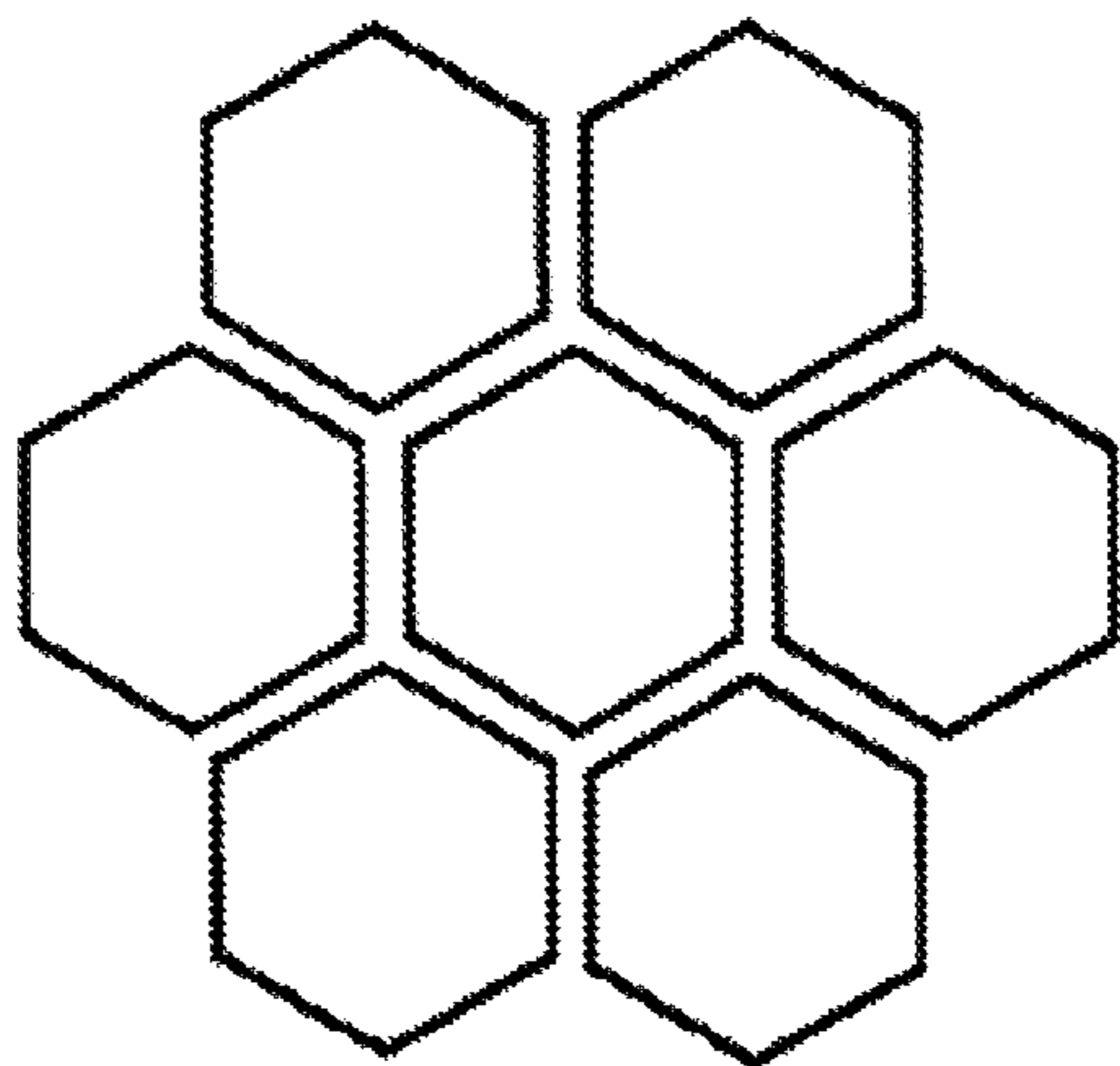
API structure
