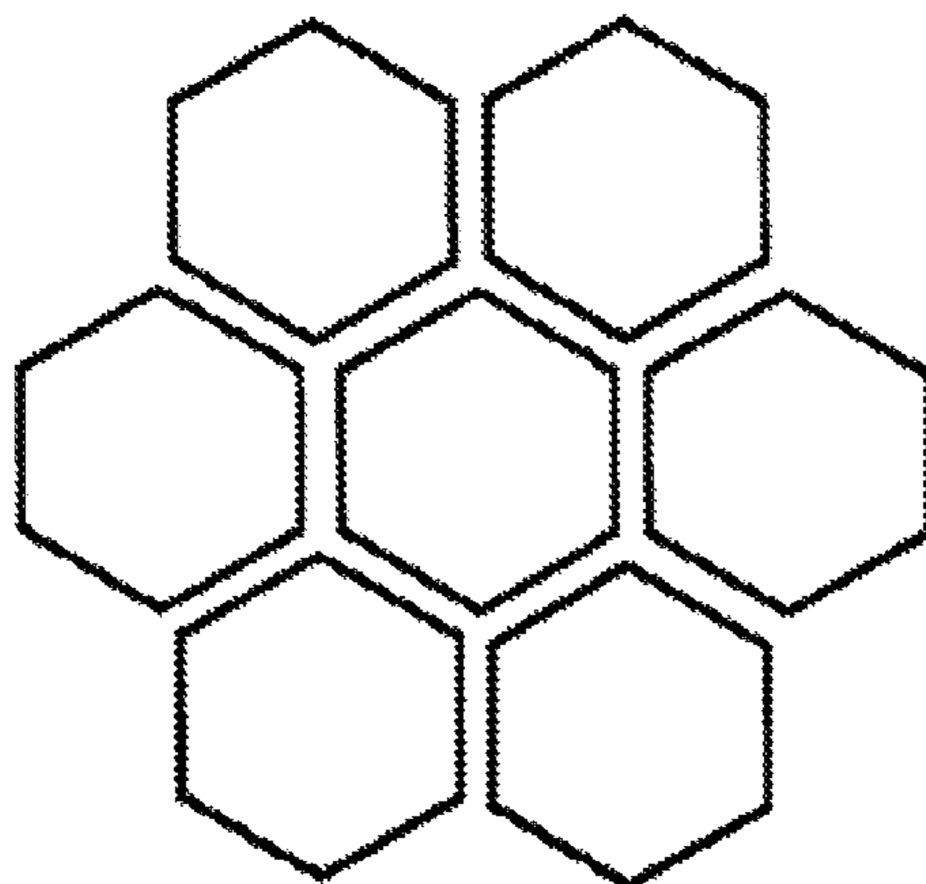
API structure
