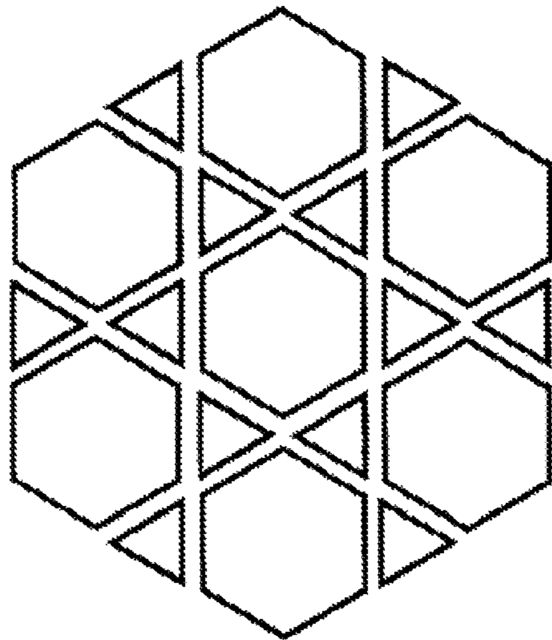
1:2 API:guest co-crystal
