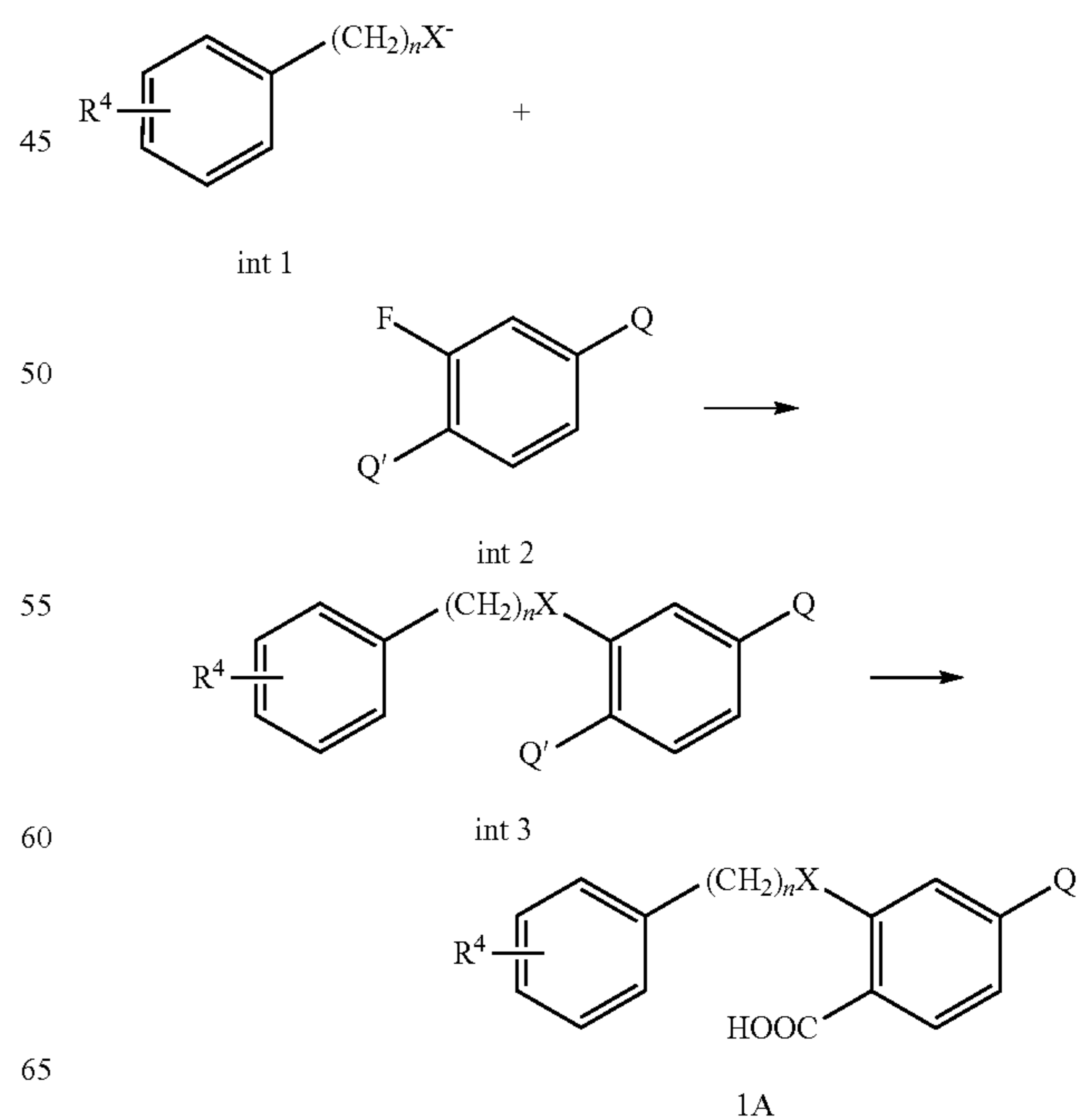
Scheme 1, Stage 1
