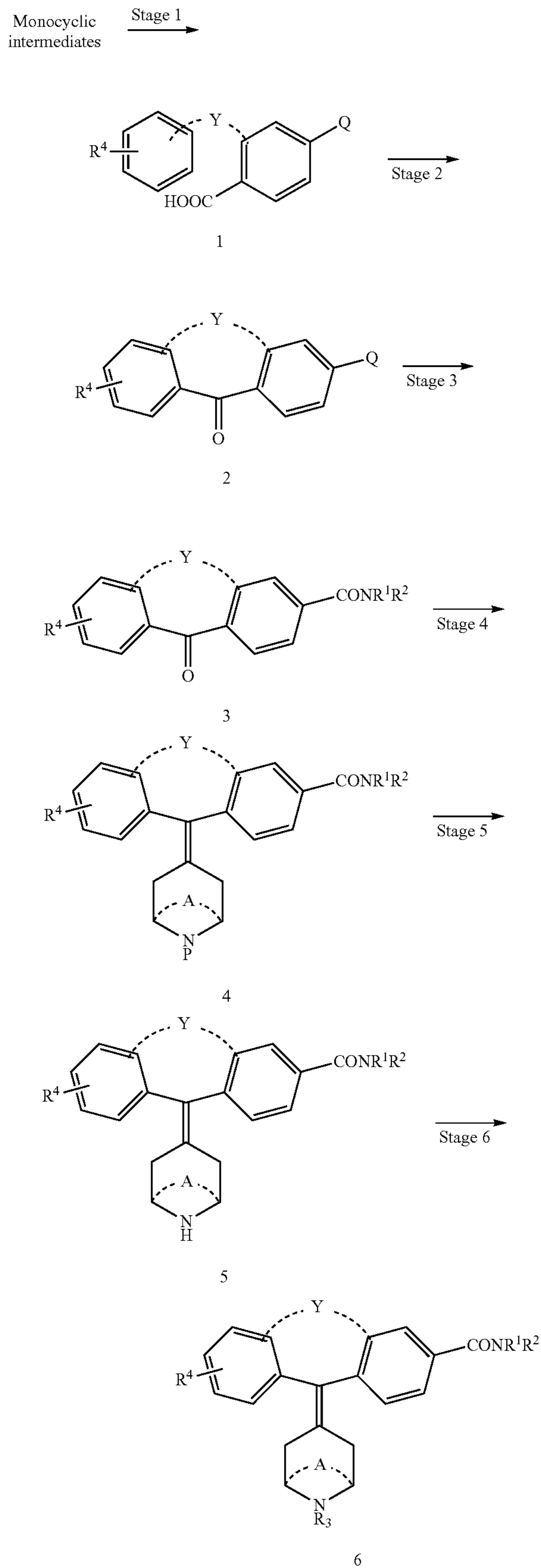
Scheme 1
