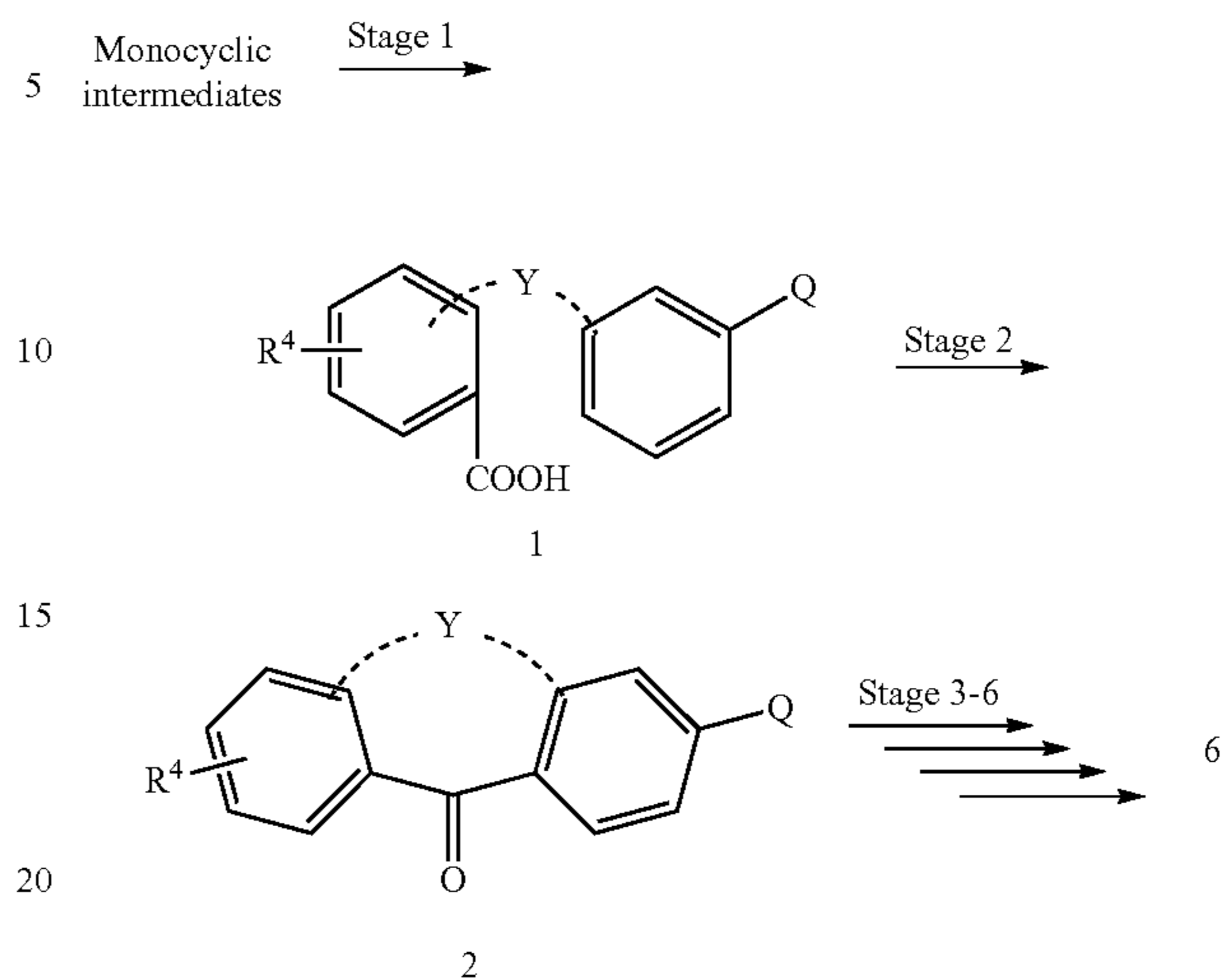
Scheme 2
