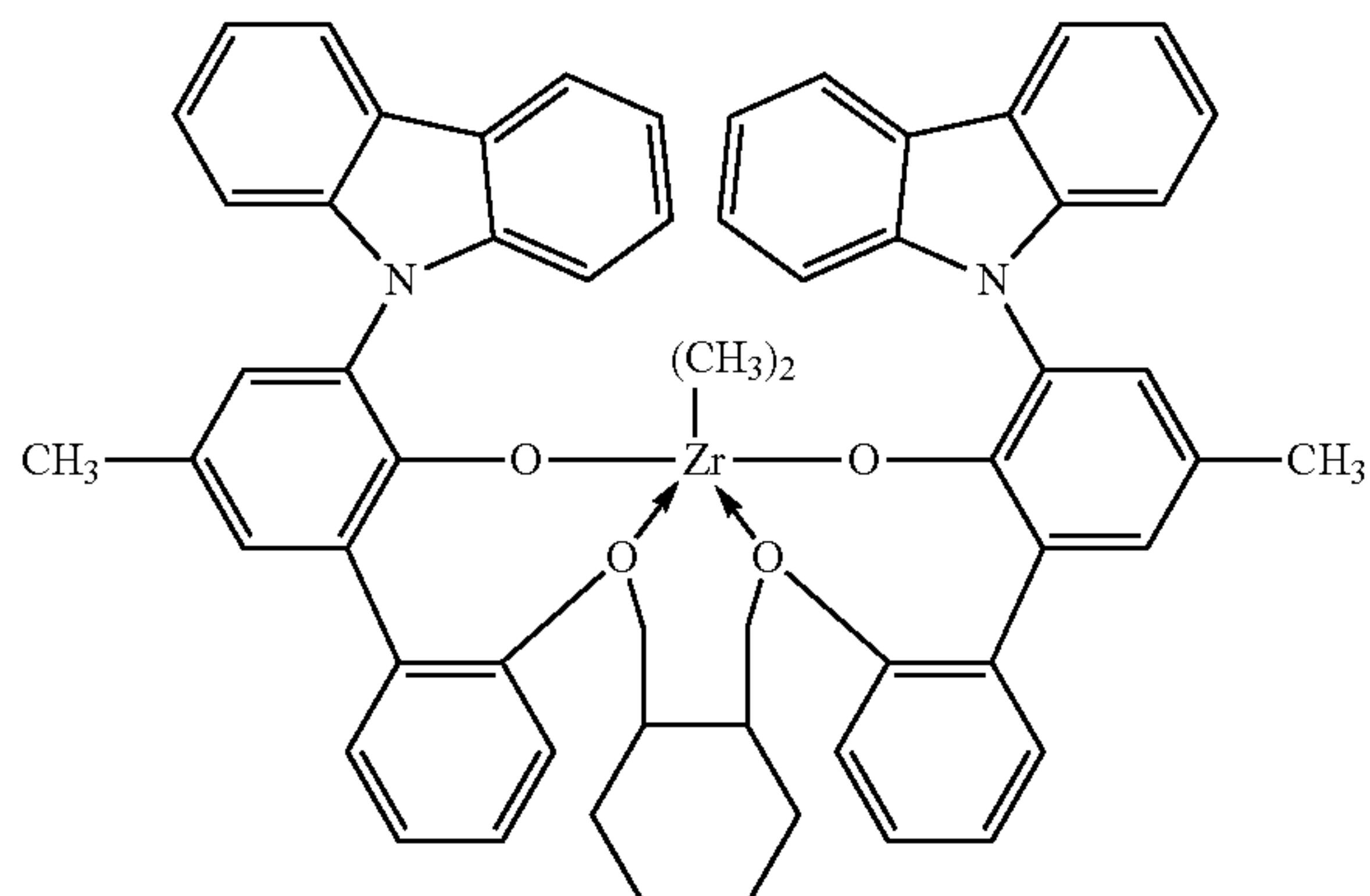
bis((2-oxoyl-3-(dibenzo-1H-pyrrole-1-yl)-5-(methyl)phenyl)-2-phenoxy)-trans-1,2-cyclohexanediylzirconium (IV) dimethyl
