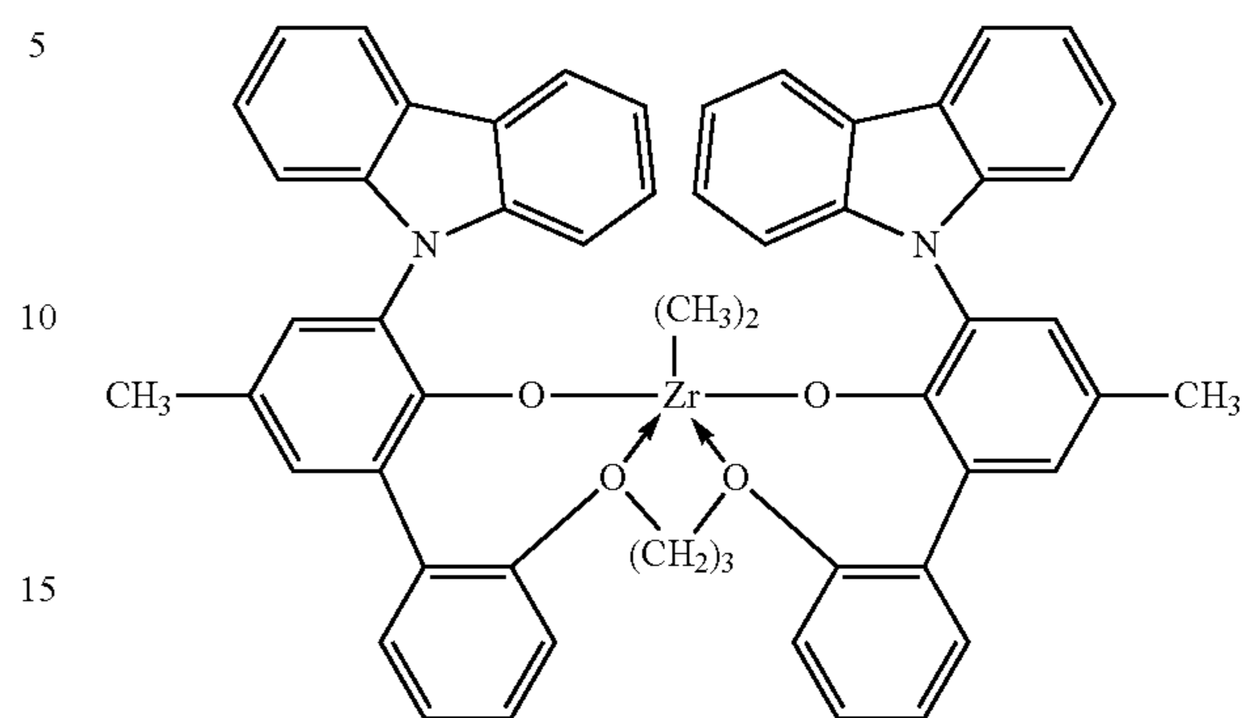
bis((2-oxoyl-3-(dibenzo-1H-pyrrole-1-yl)-5-(methyl)phenyl)-2-phenoxy)-1,3-propanediyl zirconium (IV) dimethyl
