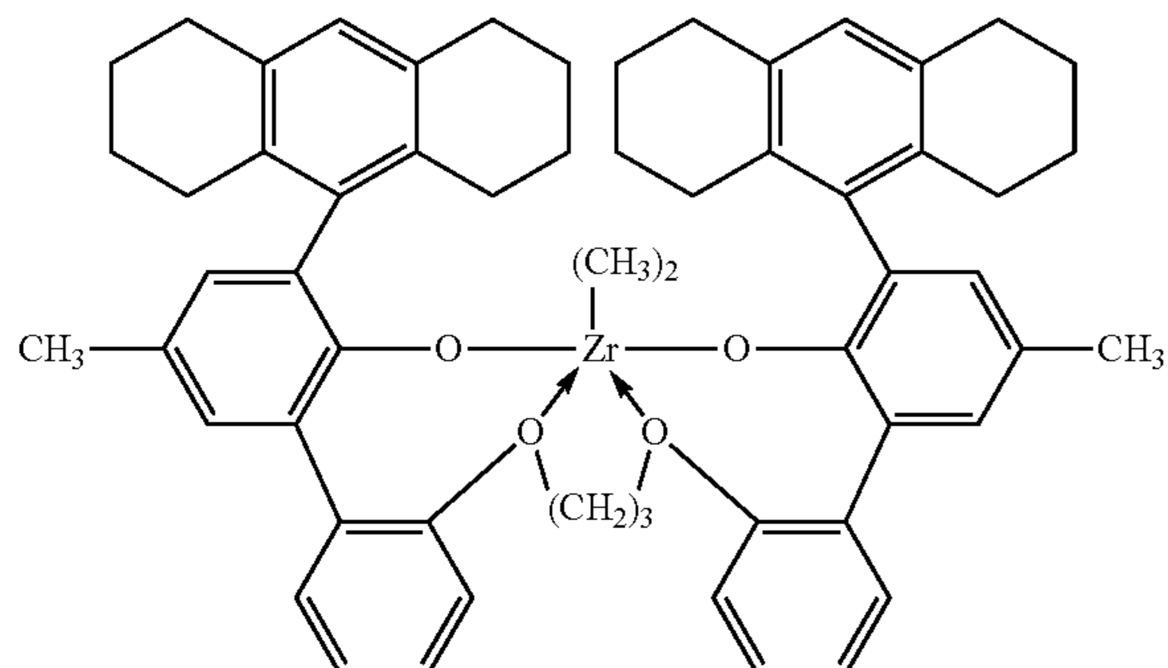
bis((2-oxoyl-3-(1,2,3,4,6,7,8,9-octahydro-anthracen-5-yl)-5-(methyl)phenyl)-2-phenoxy)-1,3-propanediyl zirconium (IV) dimethyl
