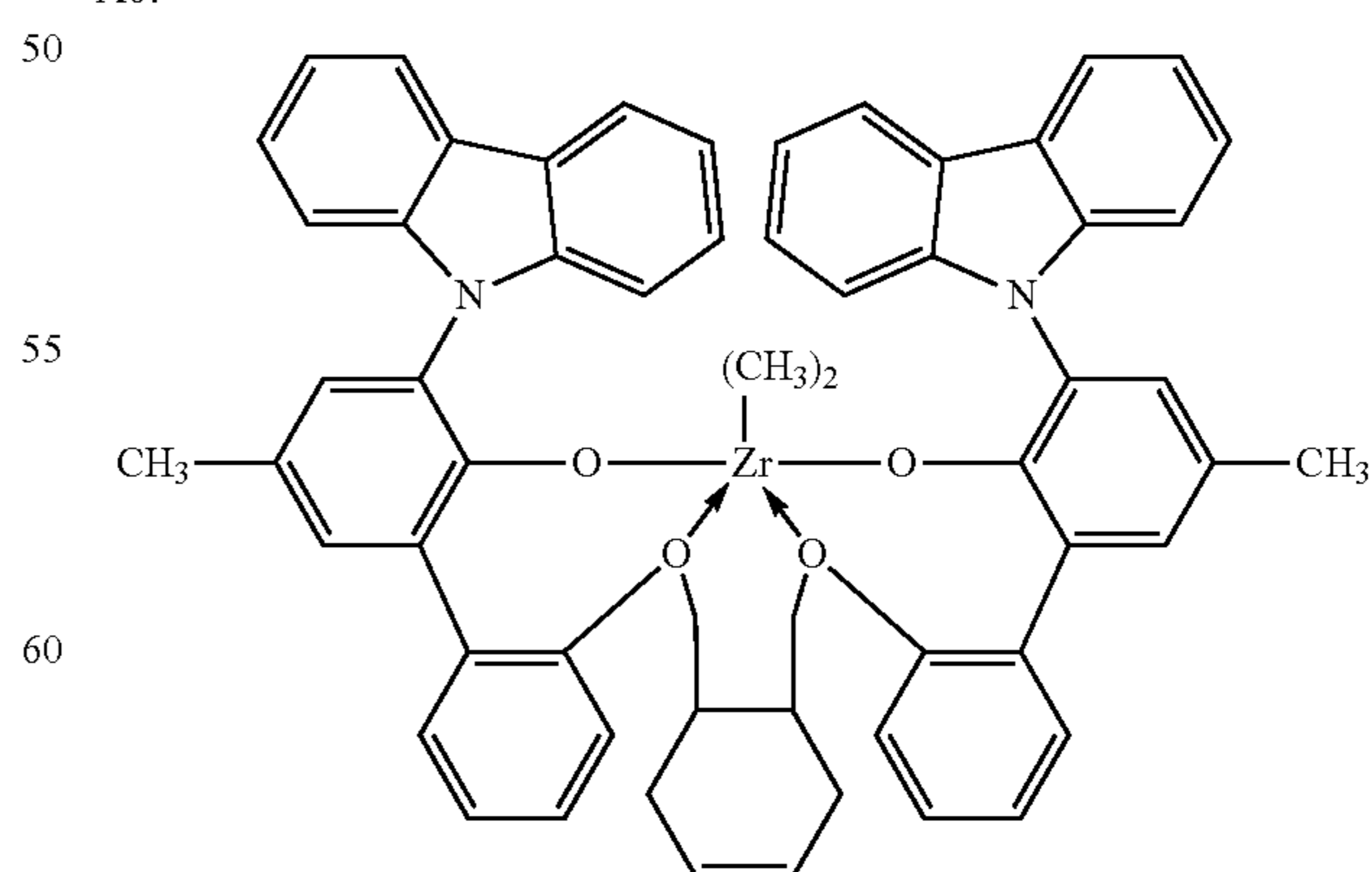
bis((2-oxoyl-3-(dibenzo-1H-pyrrole-1-yl)-5-(methyl)phenyl)-2-phenoxy)-cis-4,5-cyclohexenediyl zirconium (IV) dimethyl
