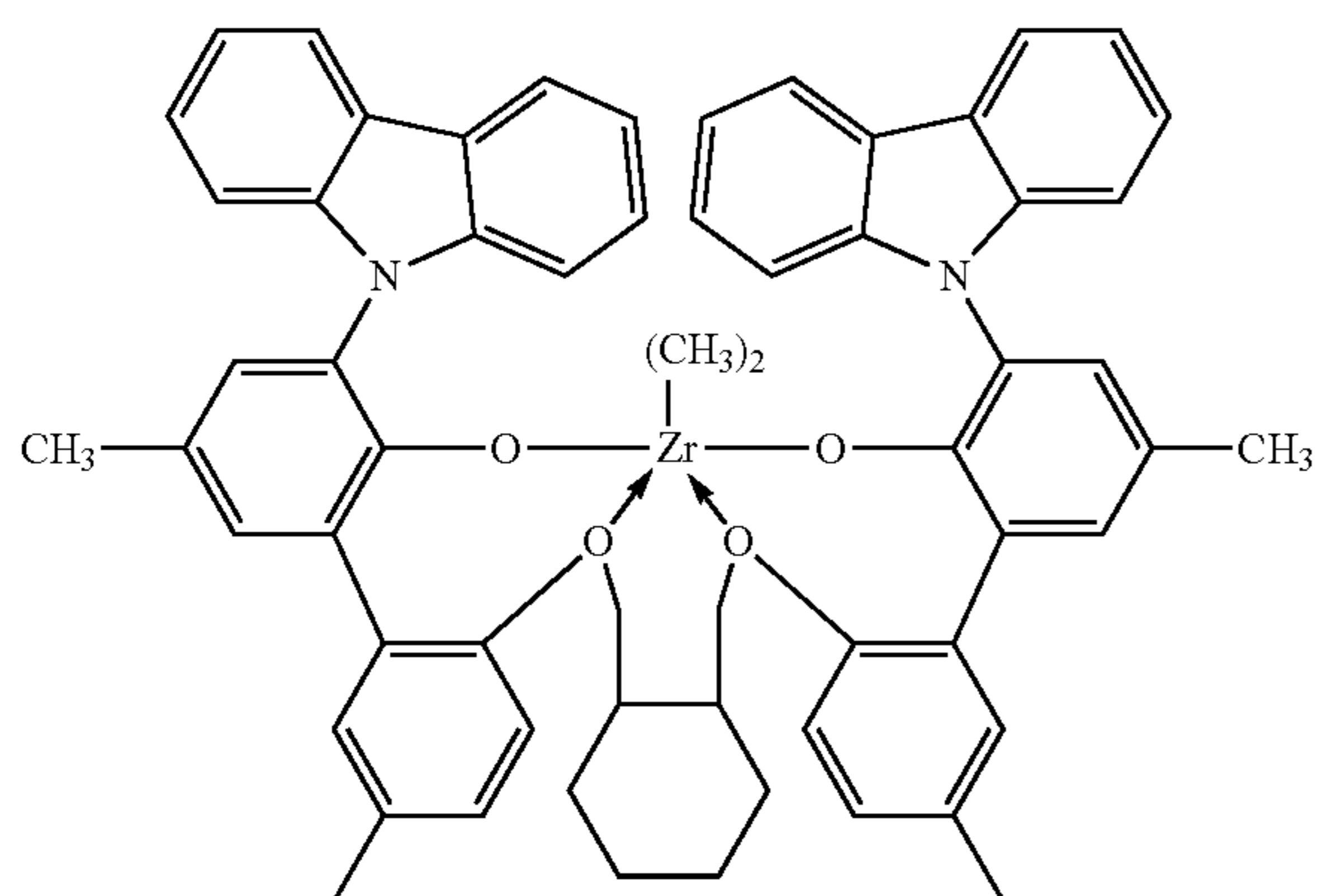
bis((2-oxoyl-3-(dibenzo-1H-pyrrole-1-yl)-5-(methyl)phenyl)-(4-methyl-2-phenoxyethyl))-trans 1,2-cyclohexanezirconium (IV) dimethyl
