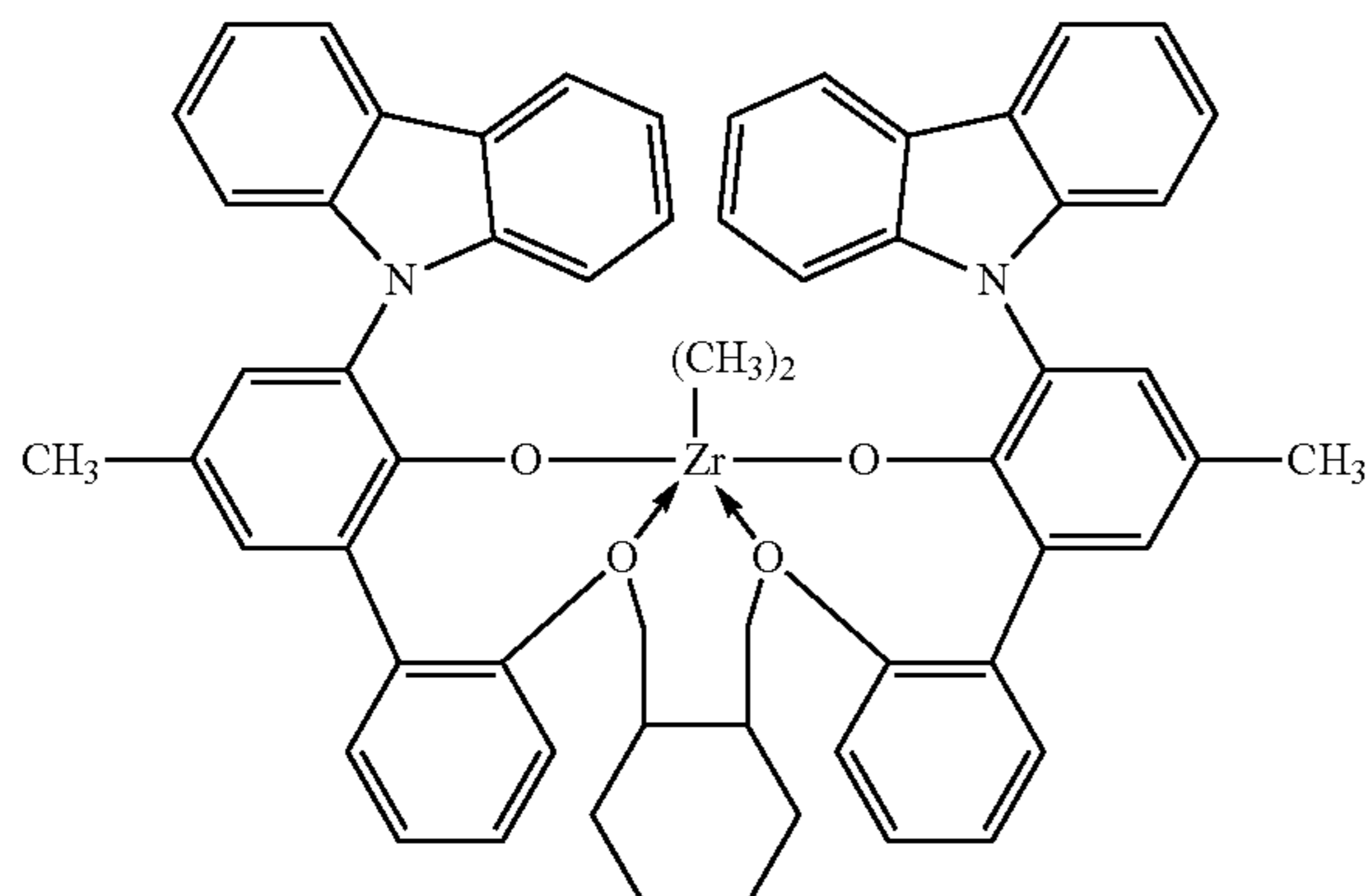
bis((2-oxoyl-3-(dibenzo-1H-pyrrole-1-yl)-5-(methyl)phenyl)-2-phenoxy)-1,2-cyclohexanediylzirconium (IV) dimethyl
