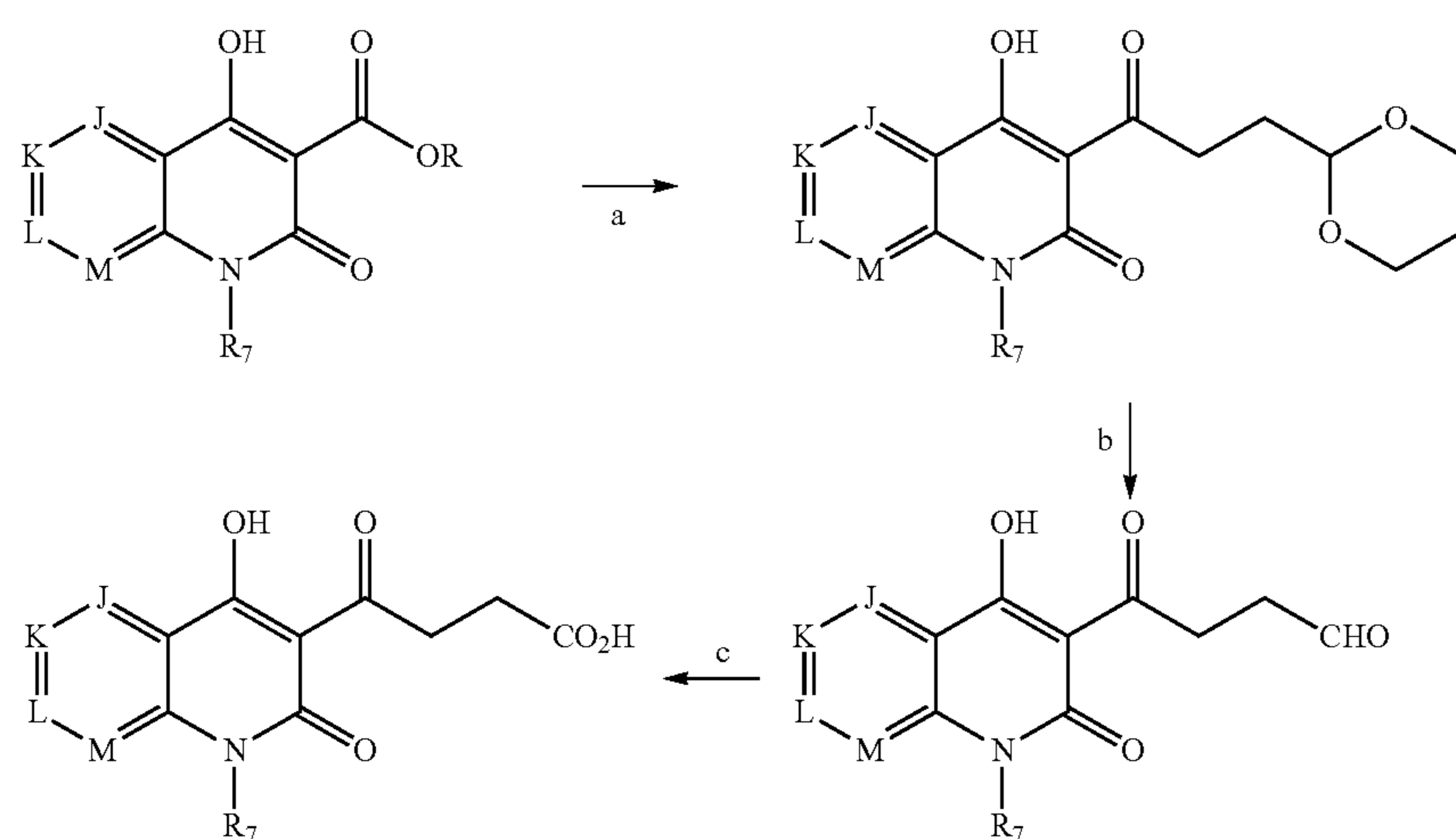
Scheme 2
