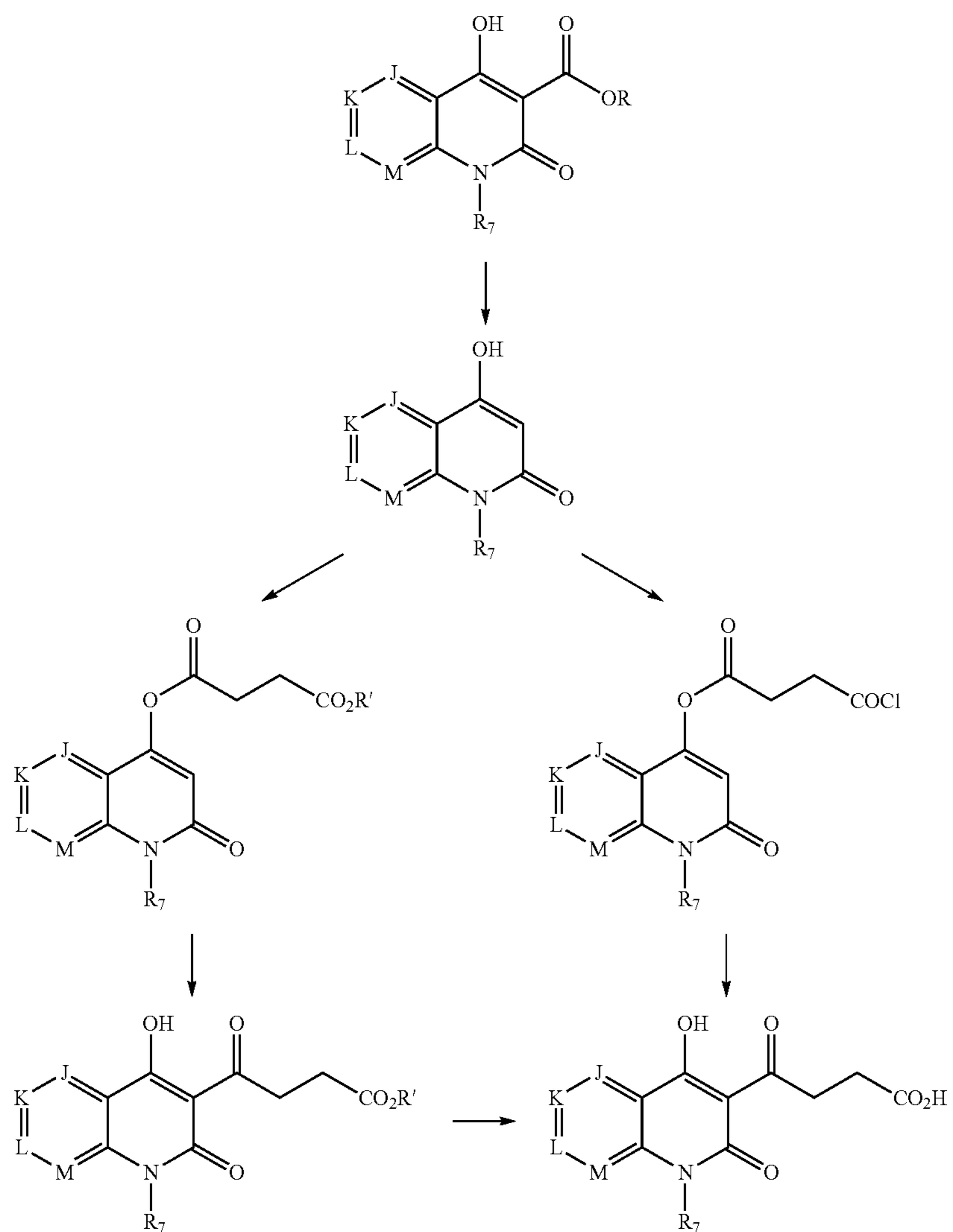
Scheme 1
