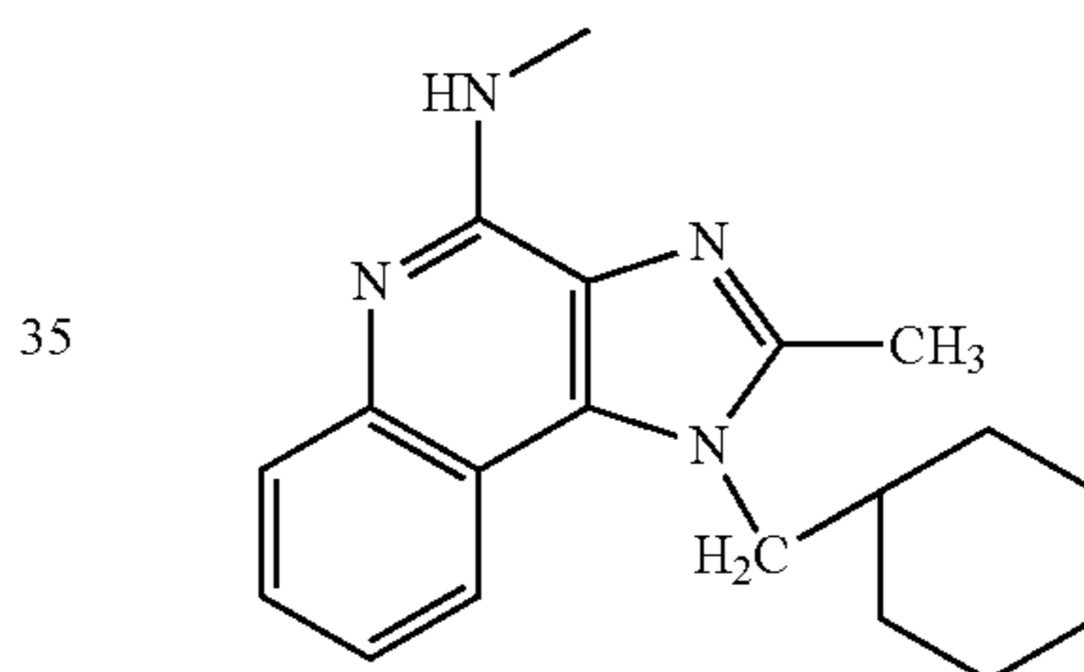
Structure F-10
