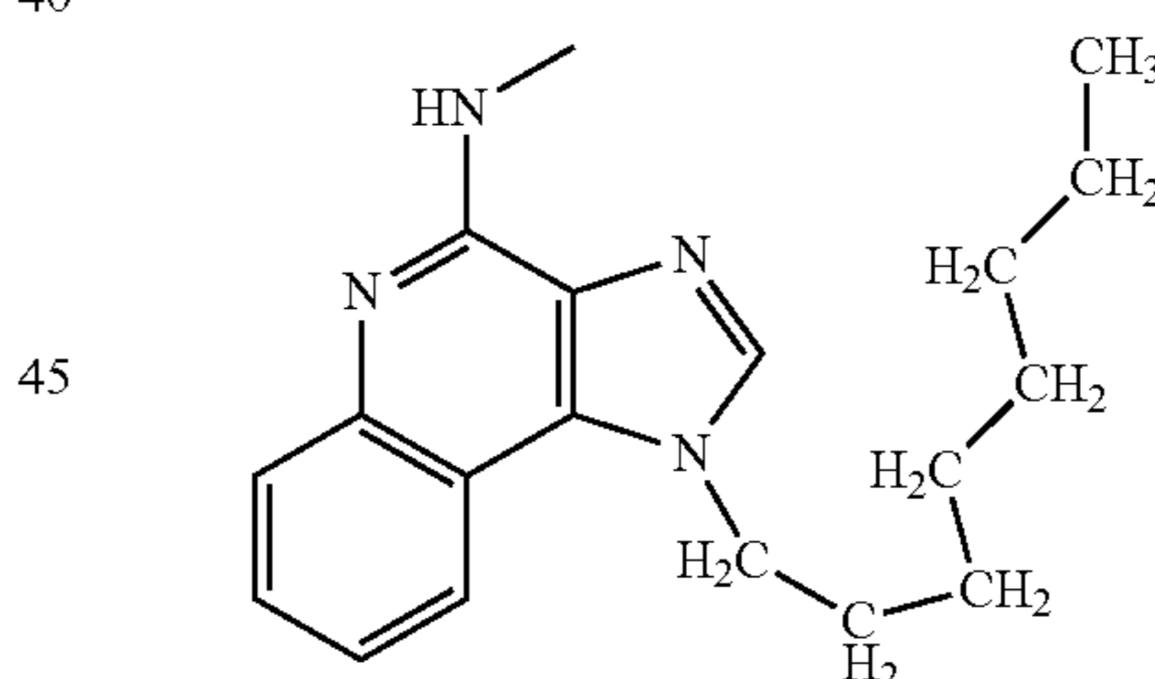
Structure F-11
