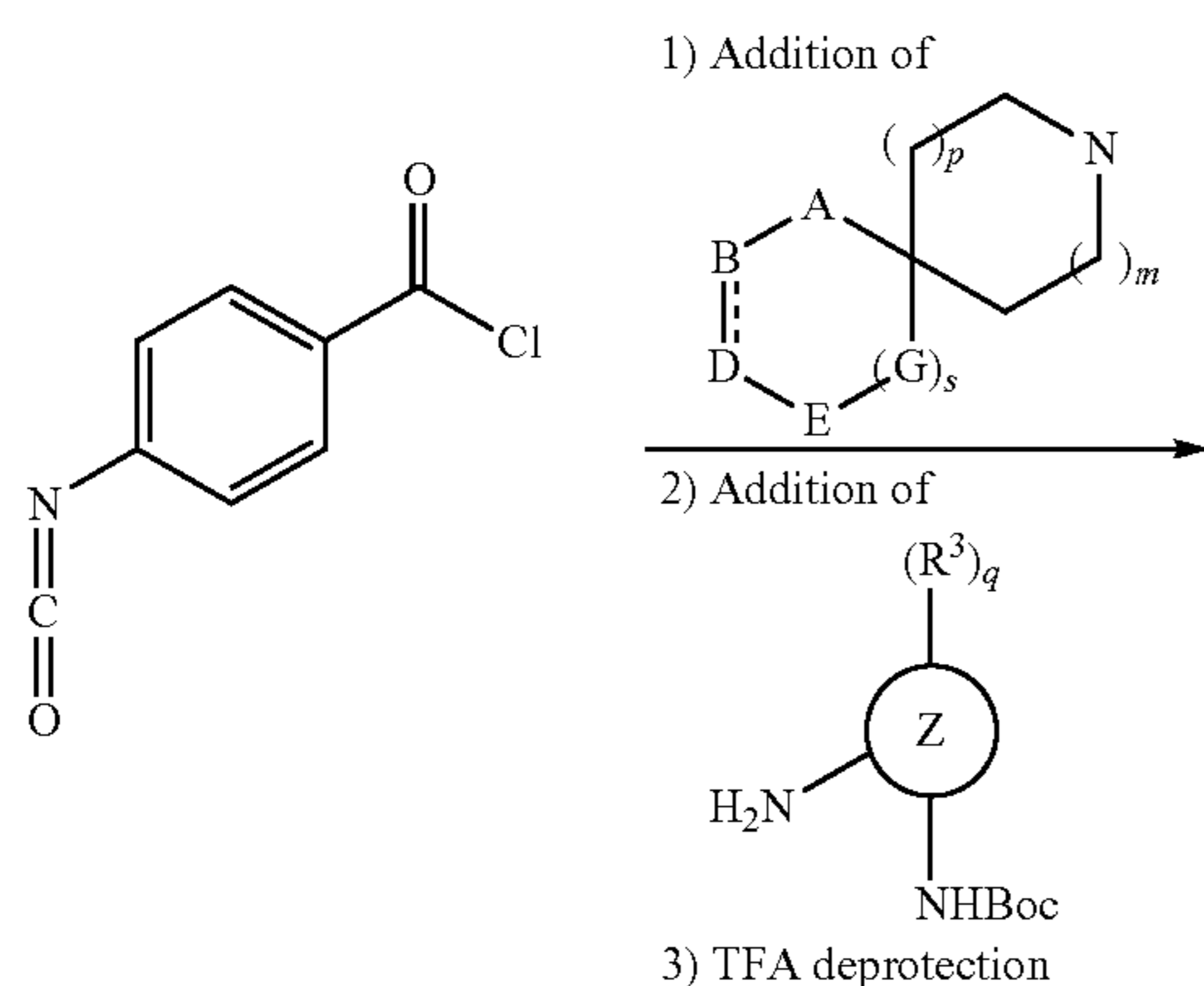
SCHEME 8
