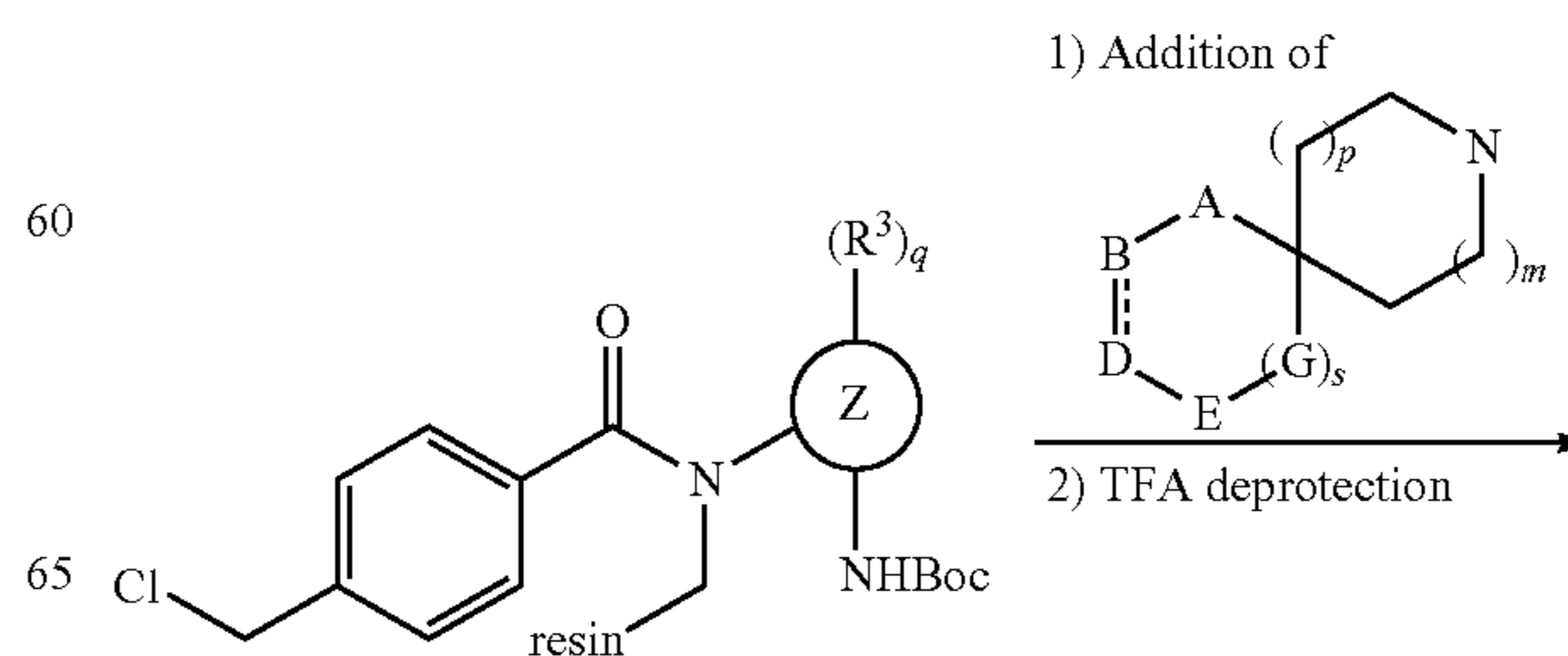
SCHEME 6
