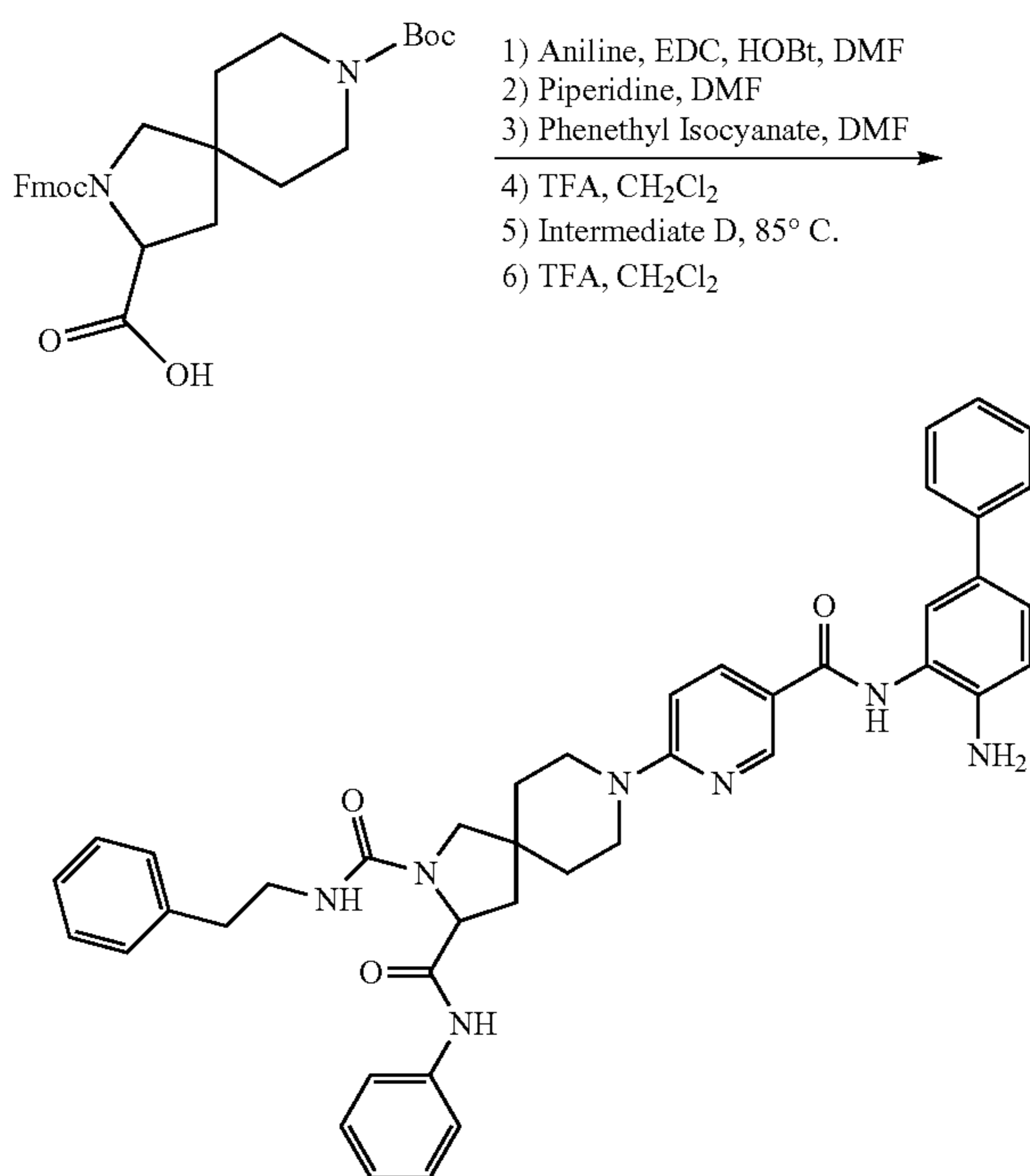
8-(5-[[[(4-Aminobiphenyl-3-yl)amino]carbonyl]pyridin-2-yl]-N 3 -phenyl-N 2 -(2-phenylethyl)-2,8-diazaspiro[4.5]decane-2,3-dicarboxamide
