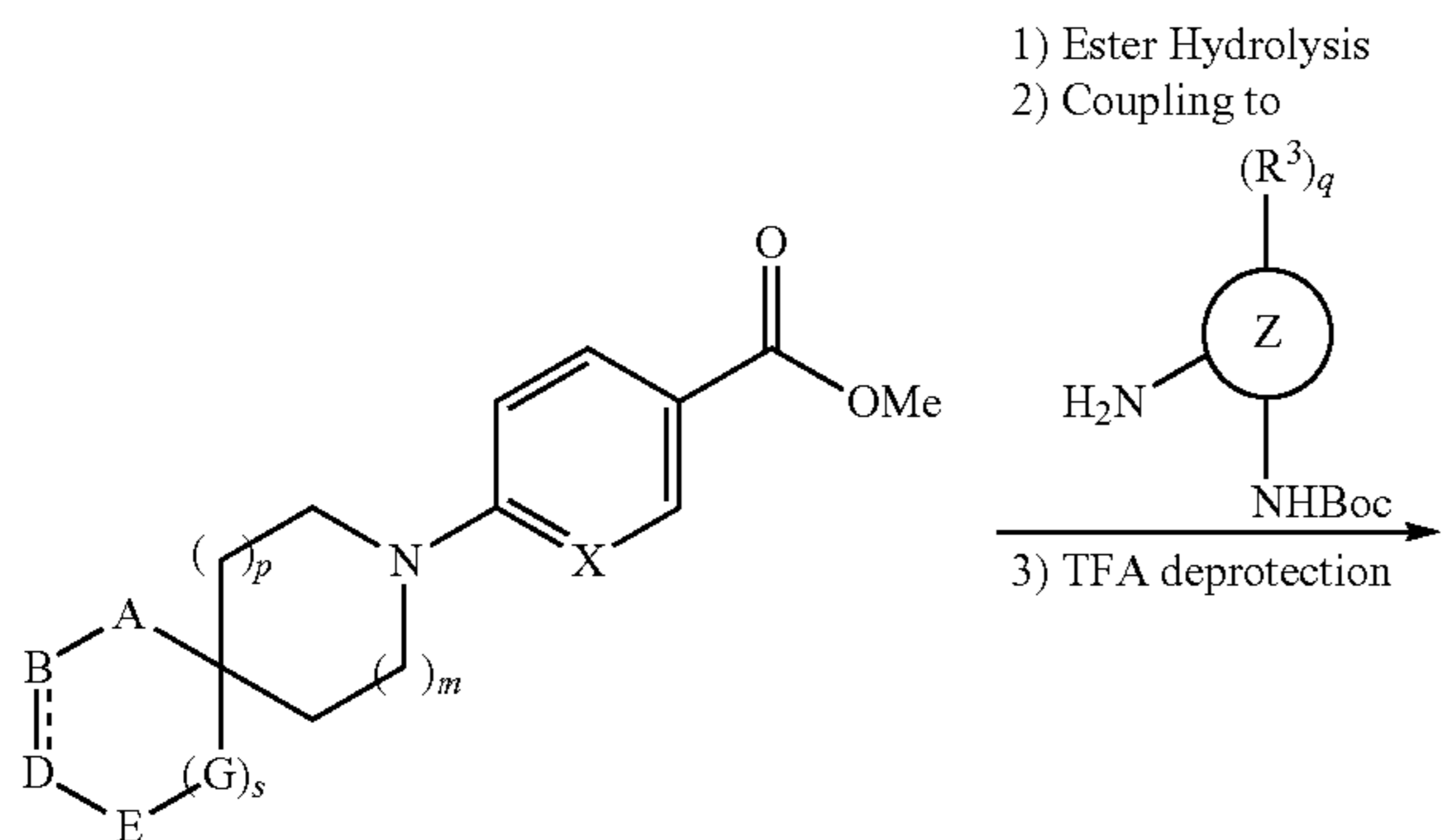
SCHEME 3
