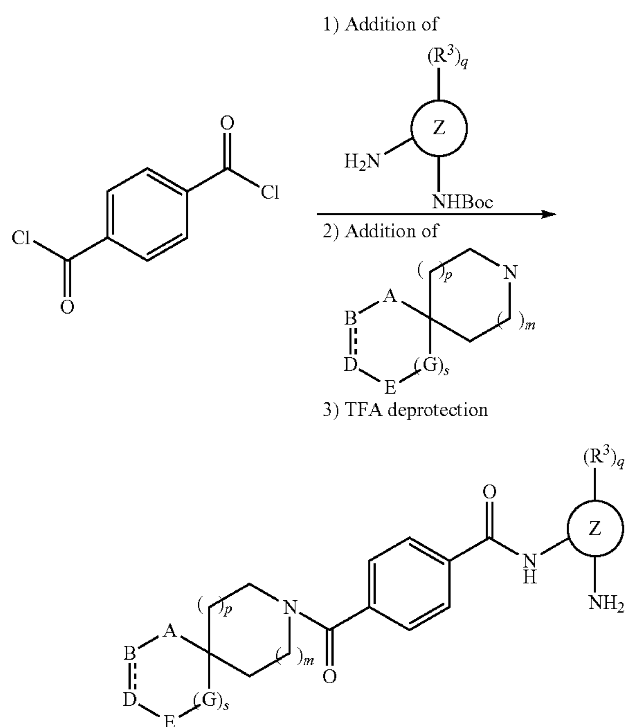
SCHEME 7
