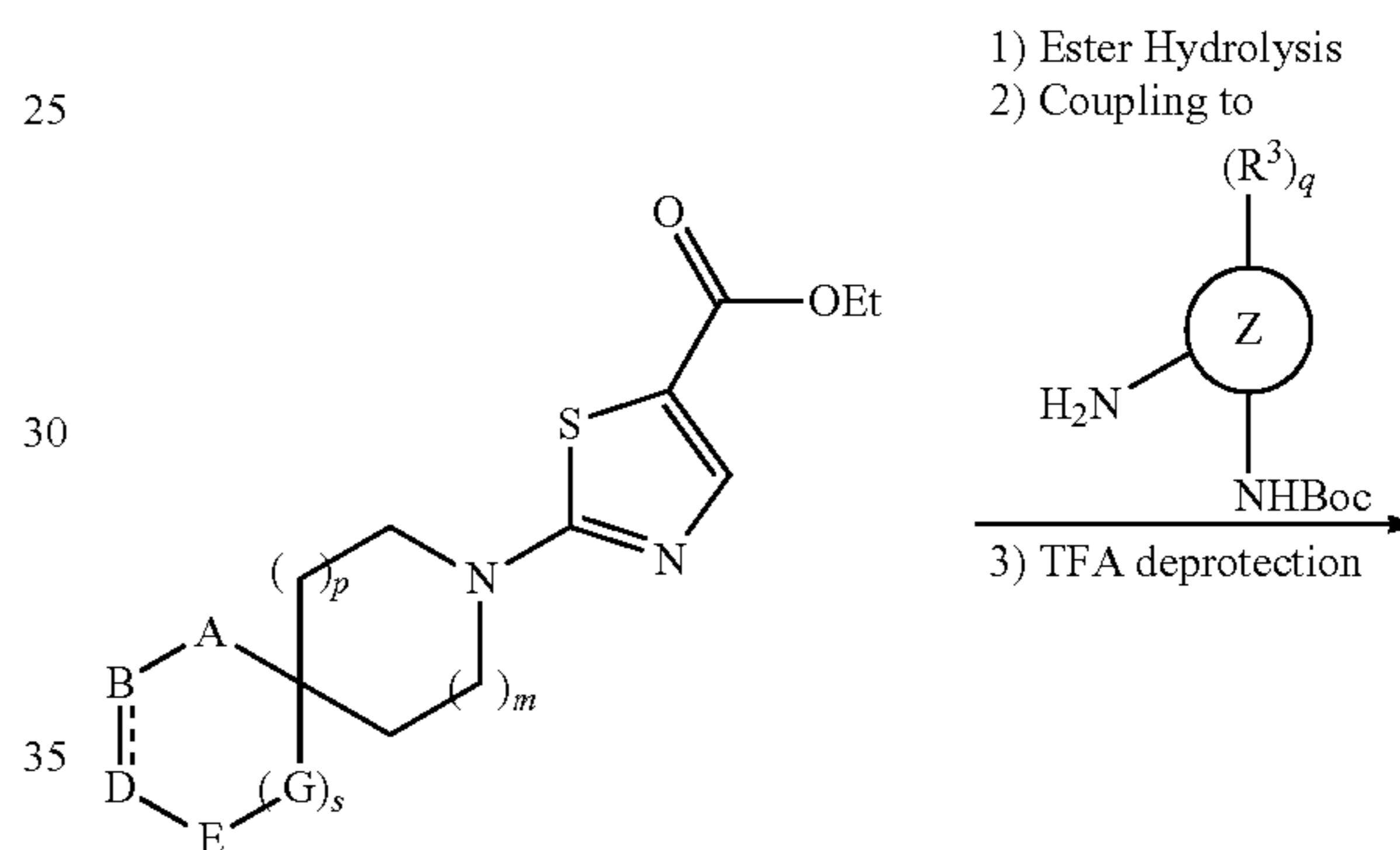
SCHEME 5
