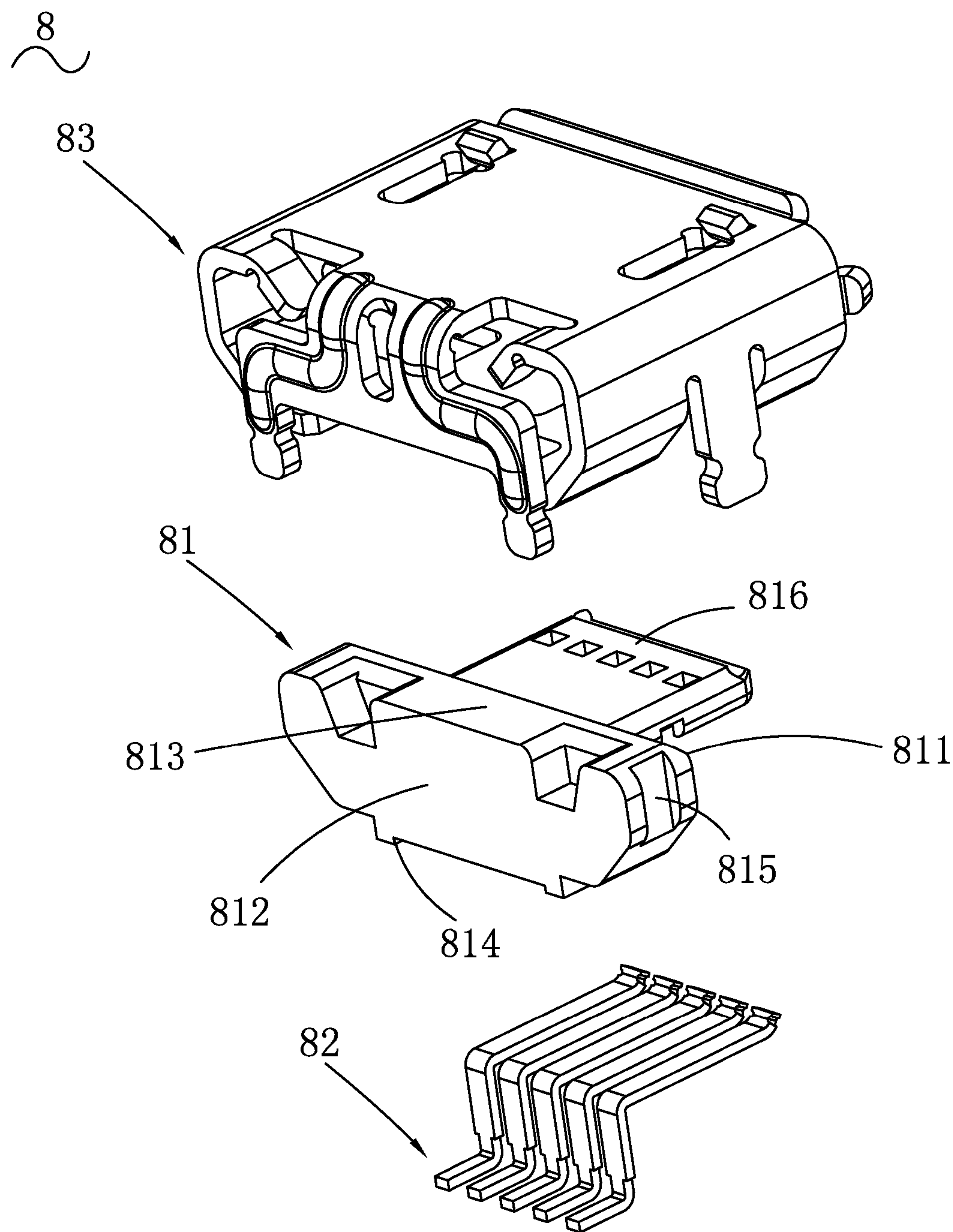
FIG. 8 (PRIOR ART)
