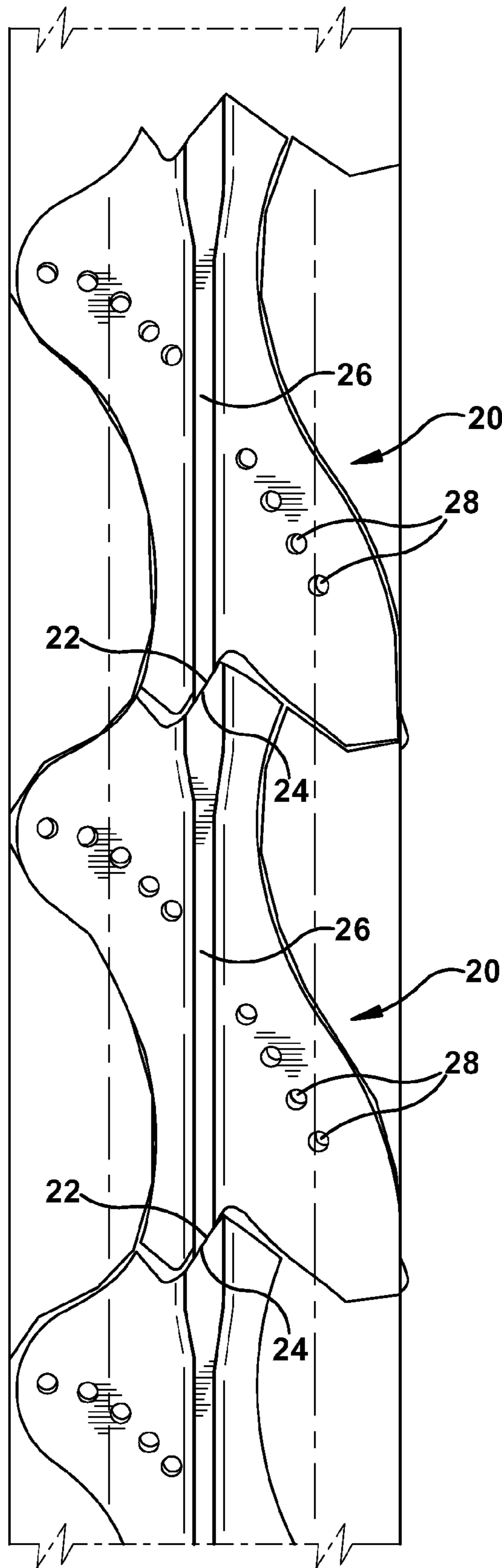
FIG. 2 PRIOR ART
