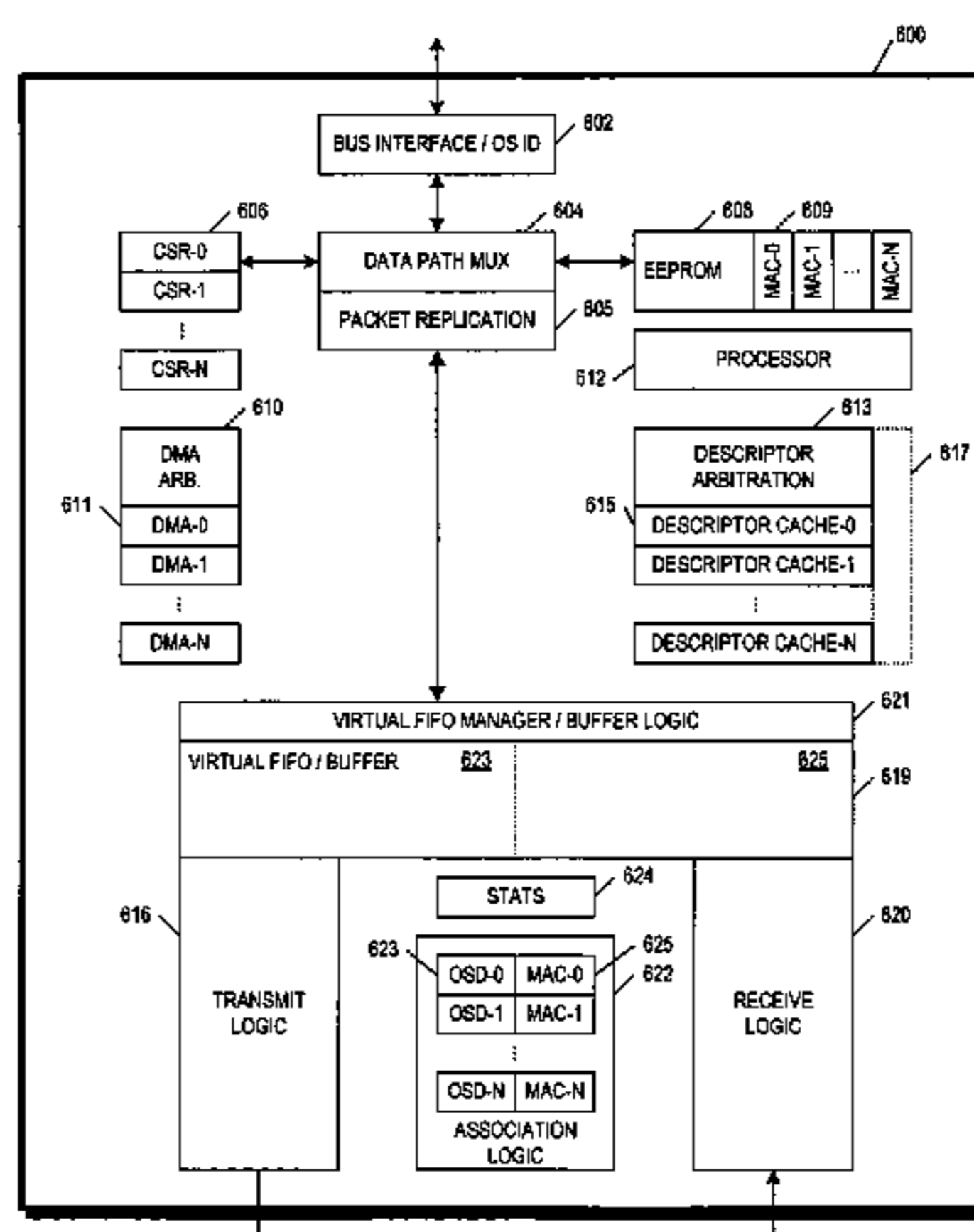
BLOCK DIAGRAM OF SHARED NETWORK INTERFACE CONTROLLER
