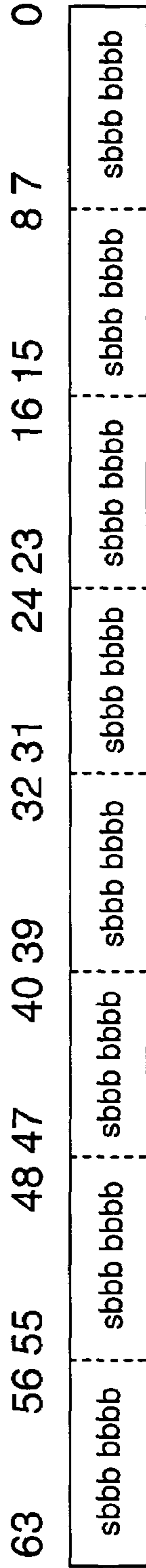
Signed packed byte in-register representation 511 FIG. 5a
