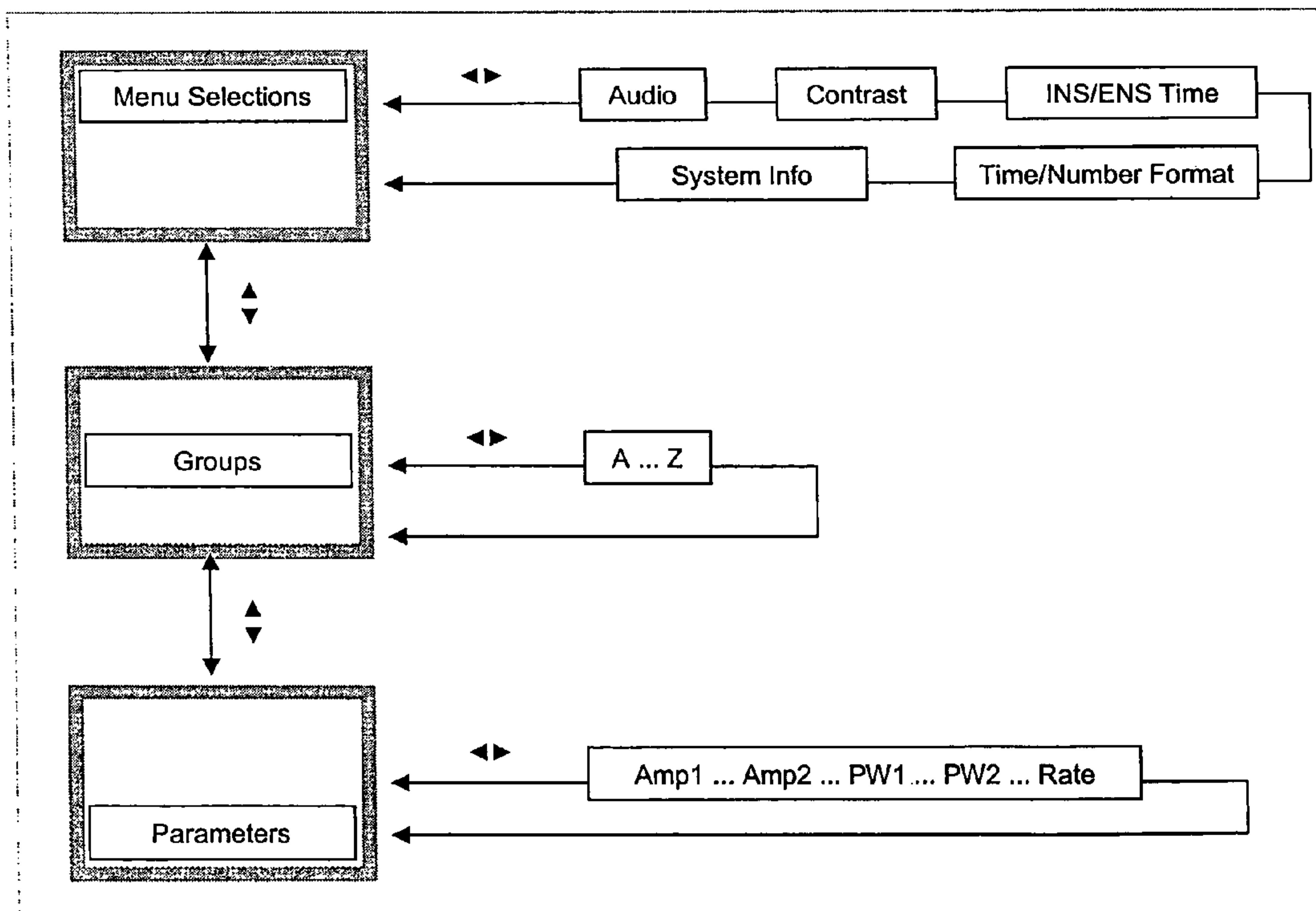
Figure 4 Operation Flow
