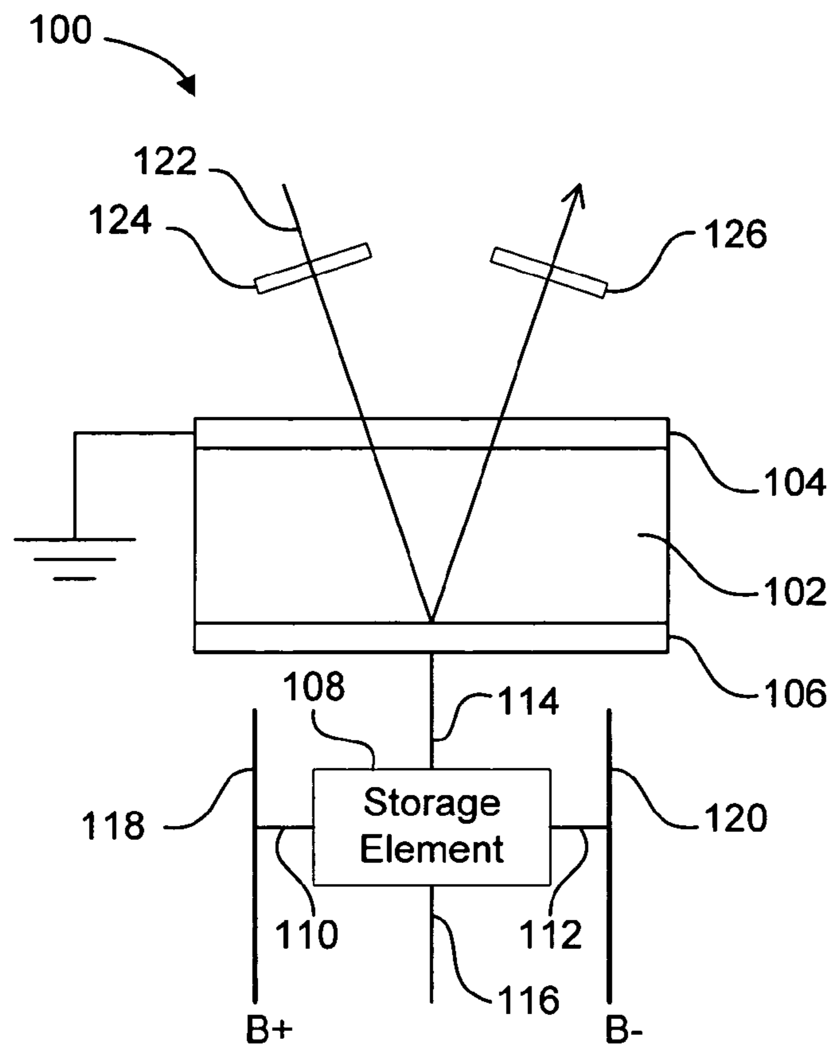
FIG. 1 Prior Art
