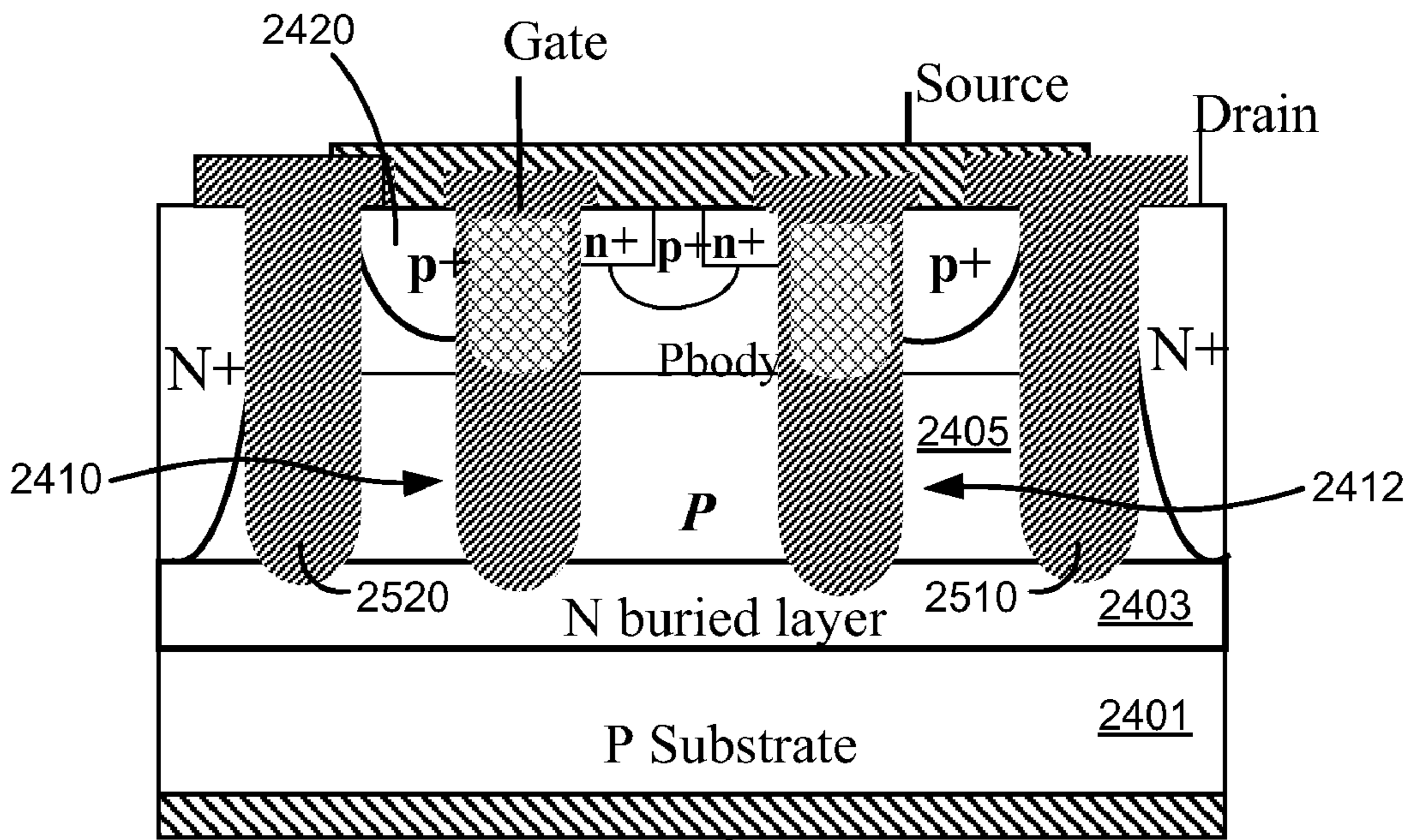
Substrate FIG. 25
