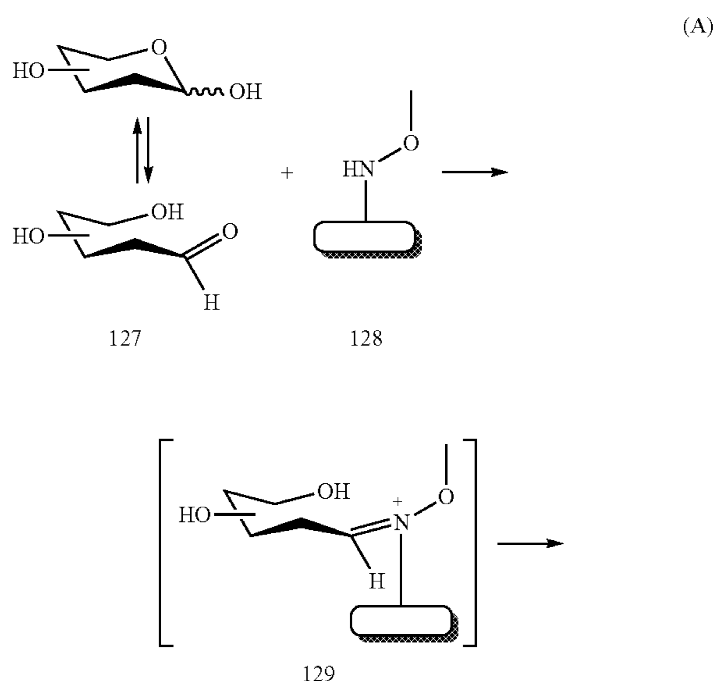
Scheme 1
