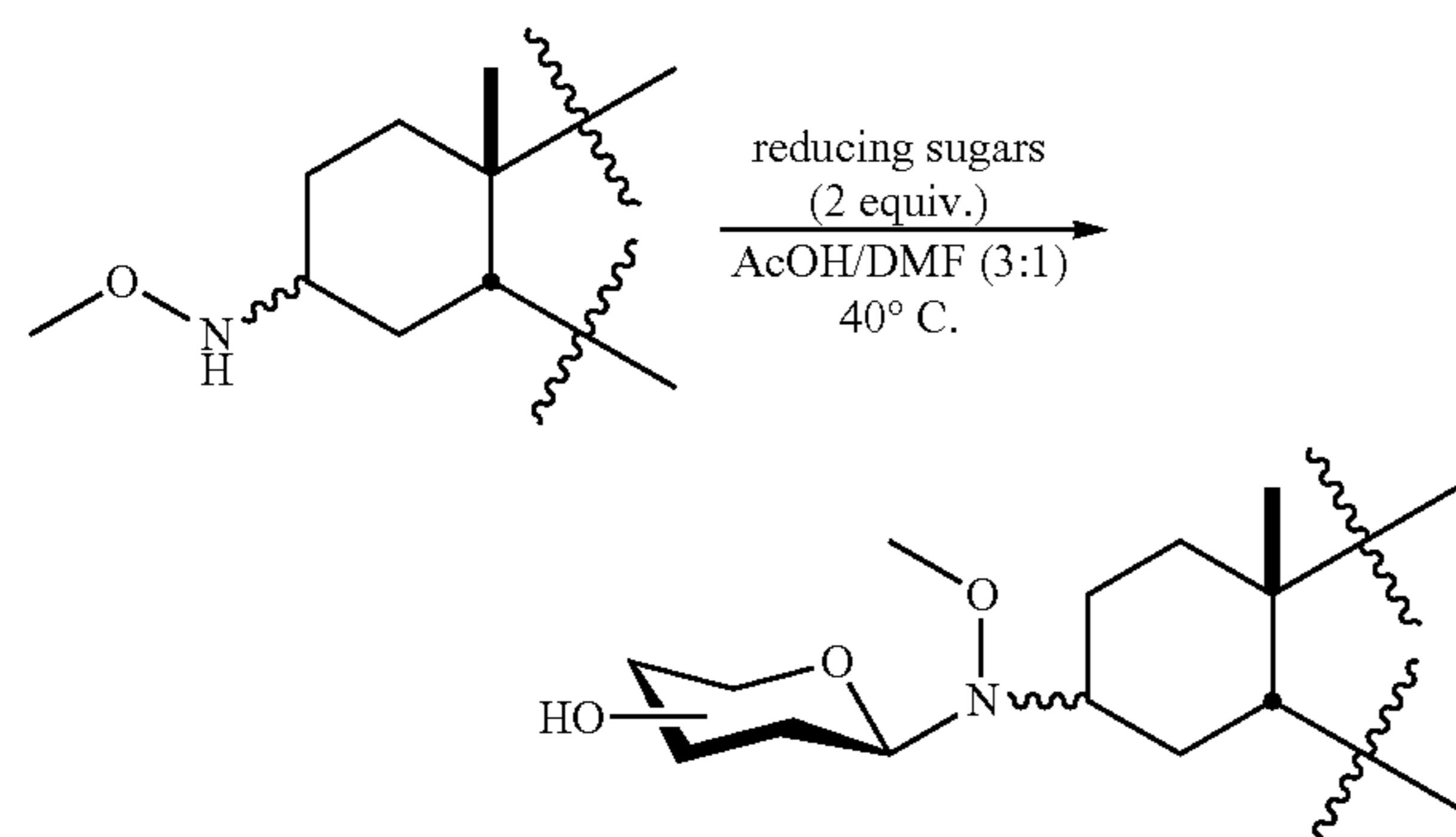
Scheme 6
