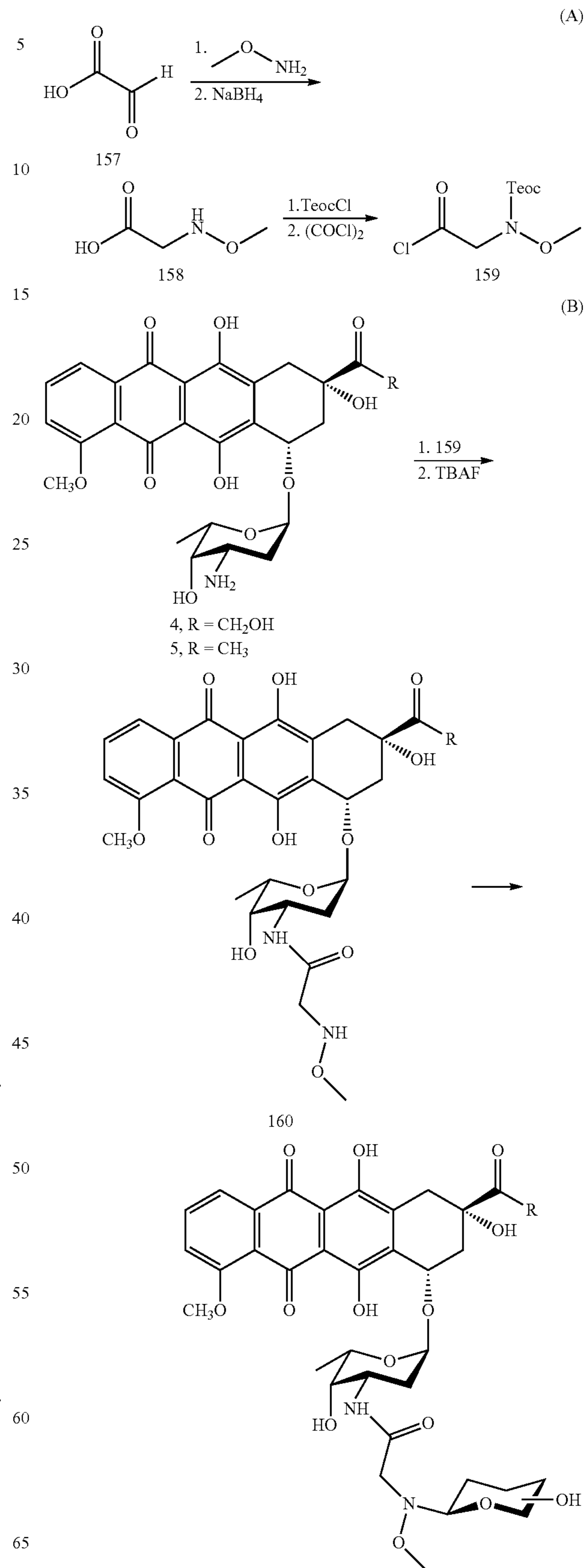
Scheme 5
