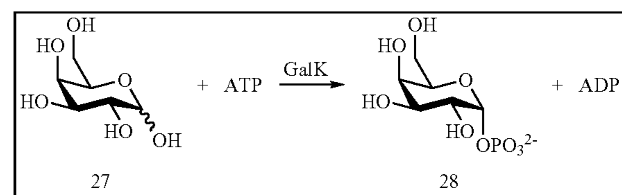
Scheme 2
