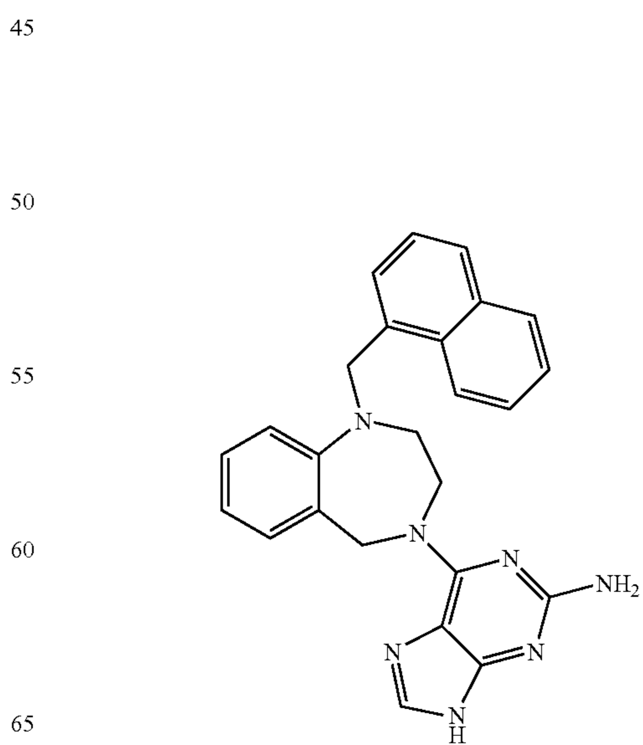
Compound 17
