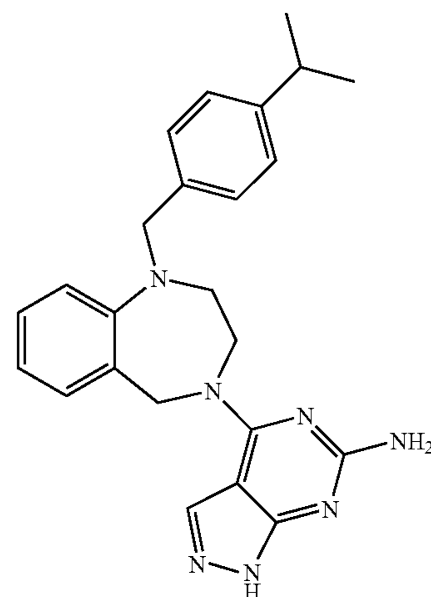
Compound 4
