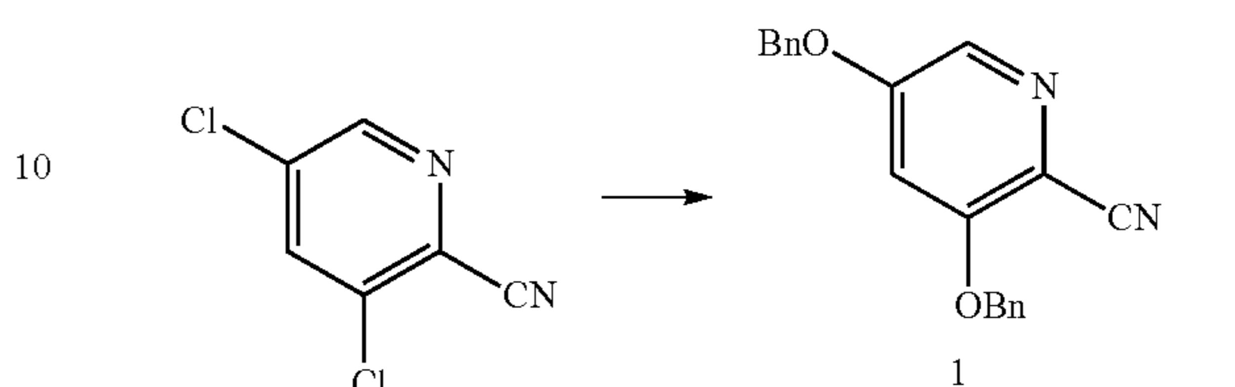
Scheme I
