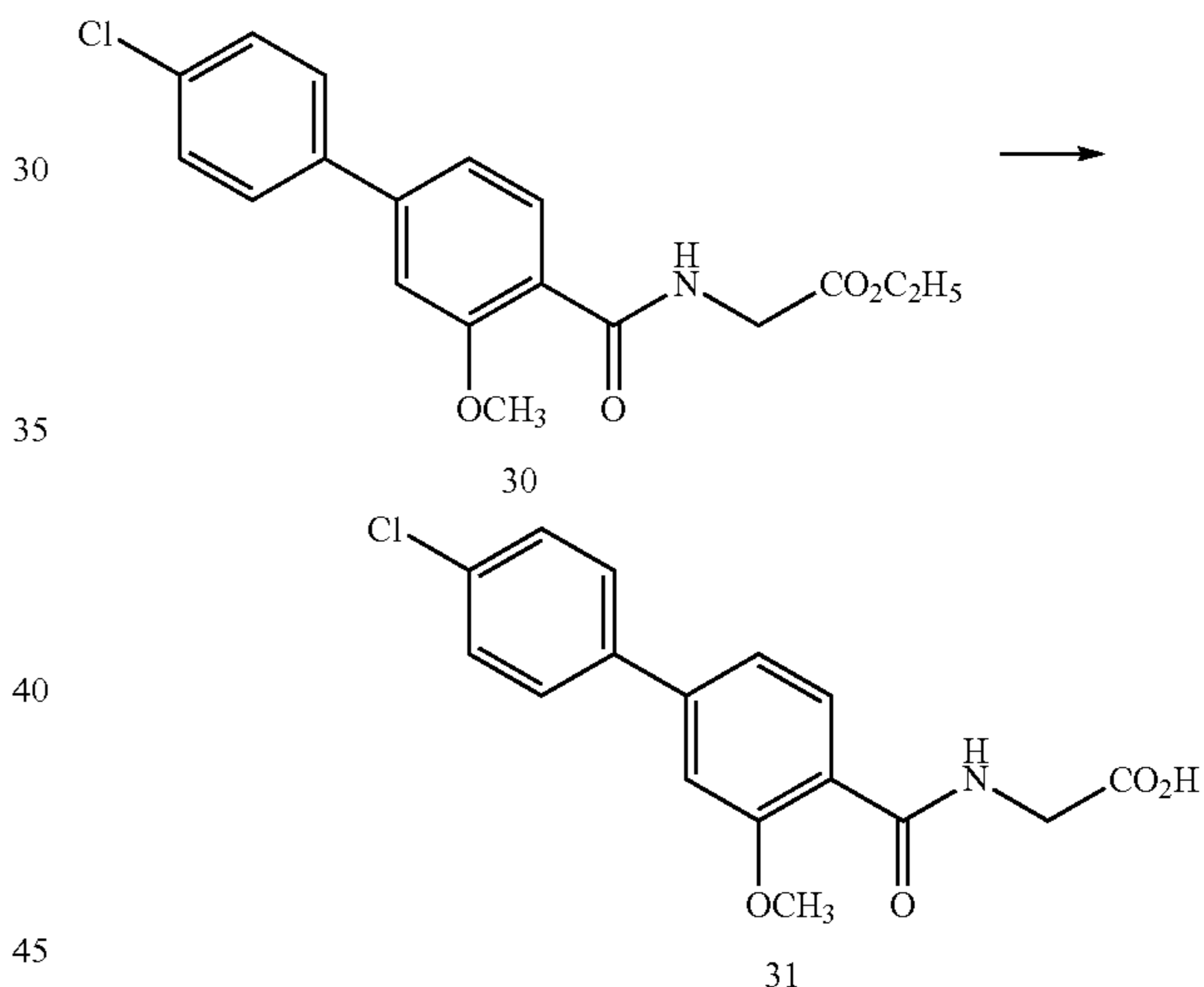
Scheme XVIII
