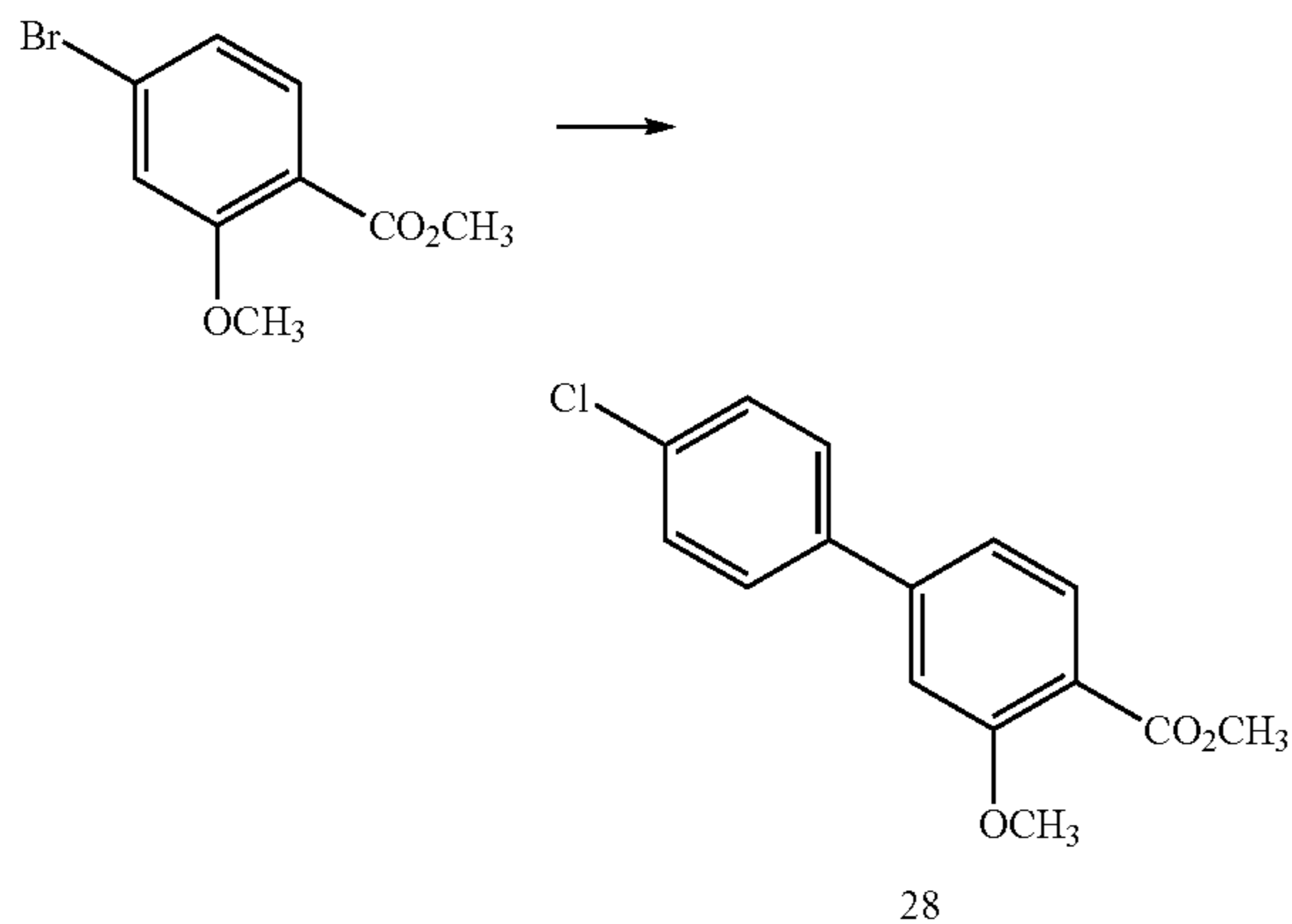
Scheme XVII
