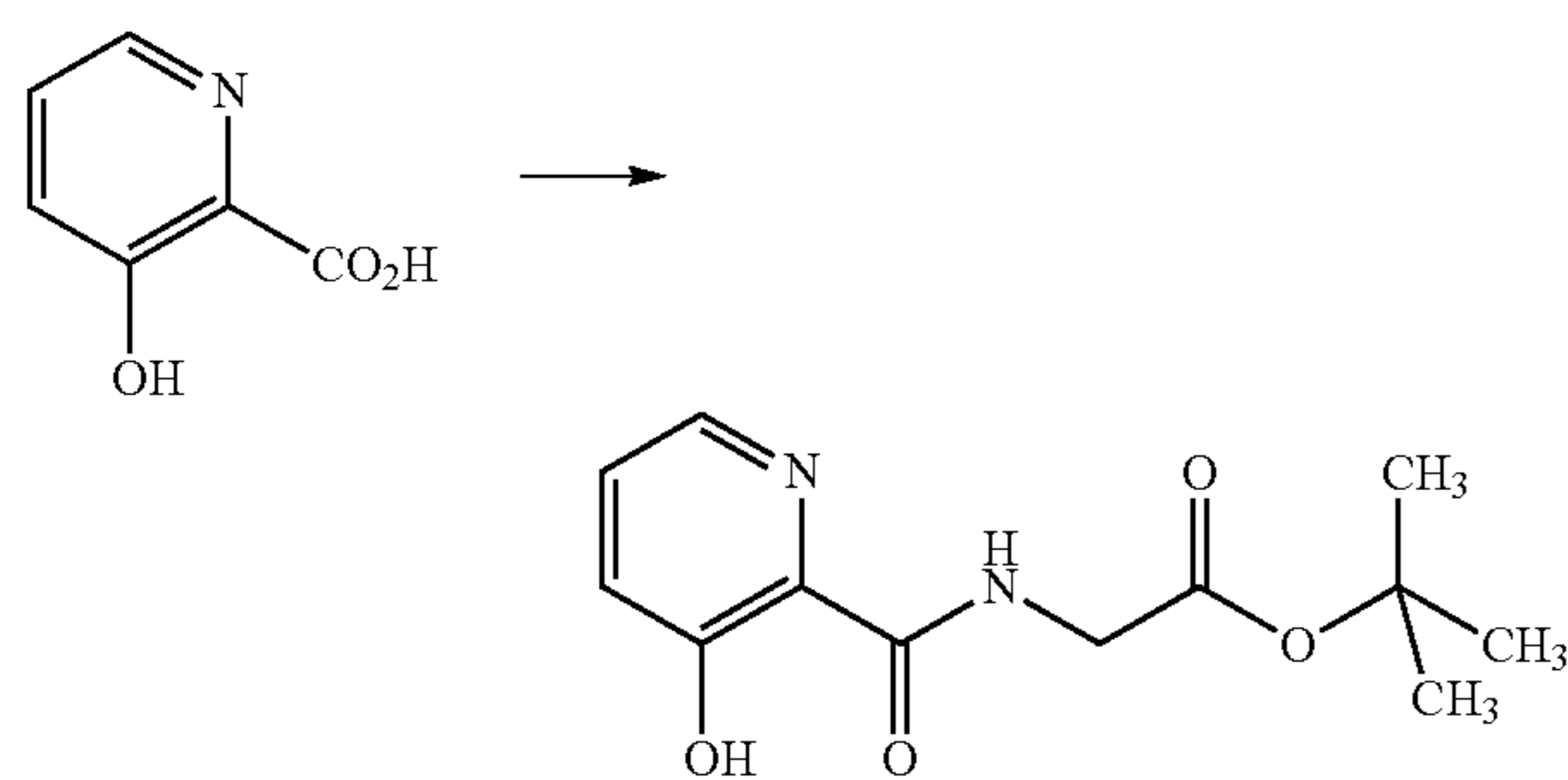
Scheme XVI
