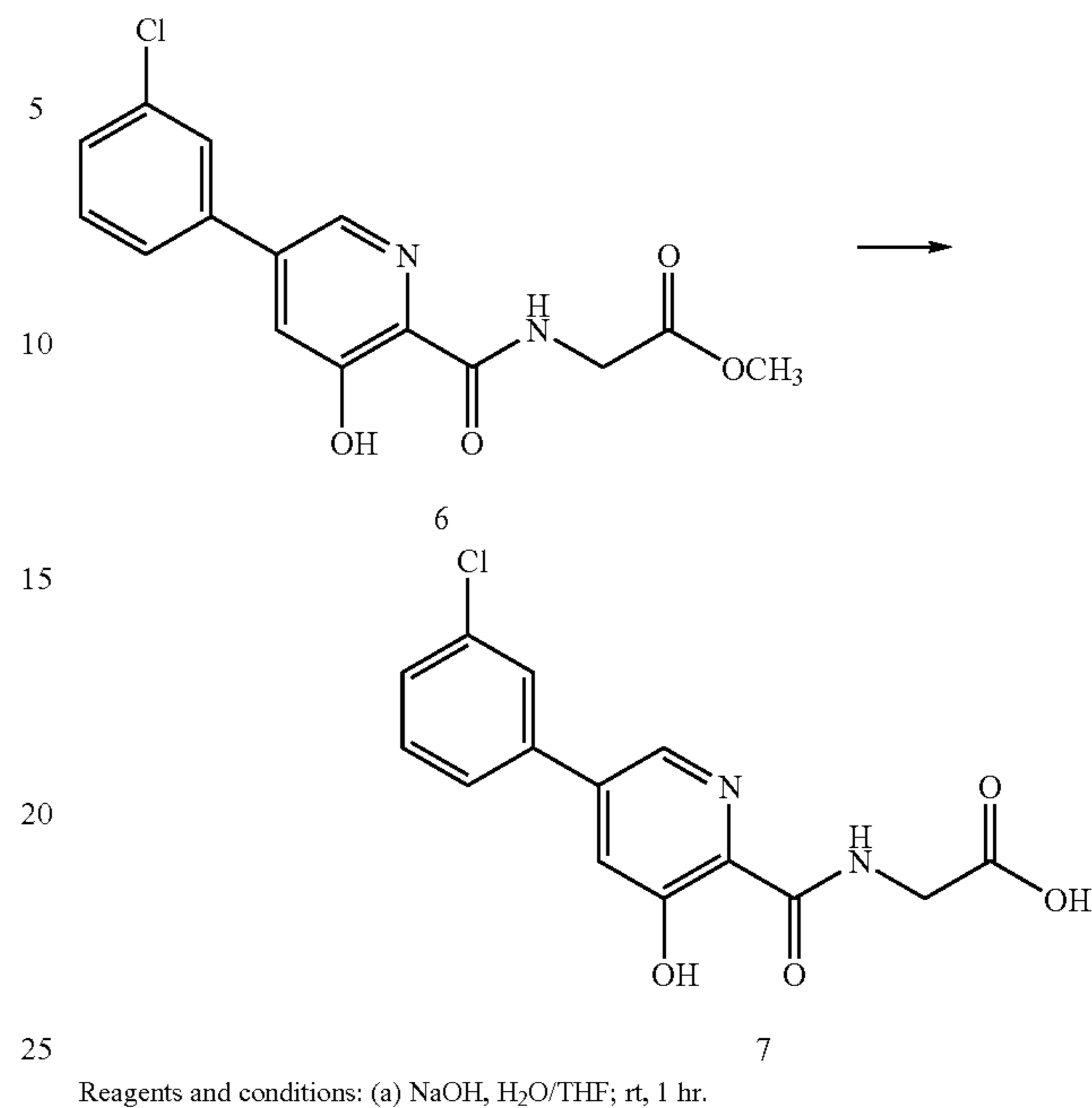
Scheme II
