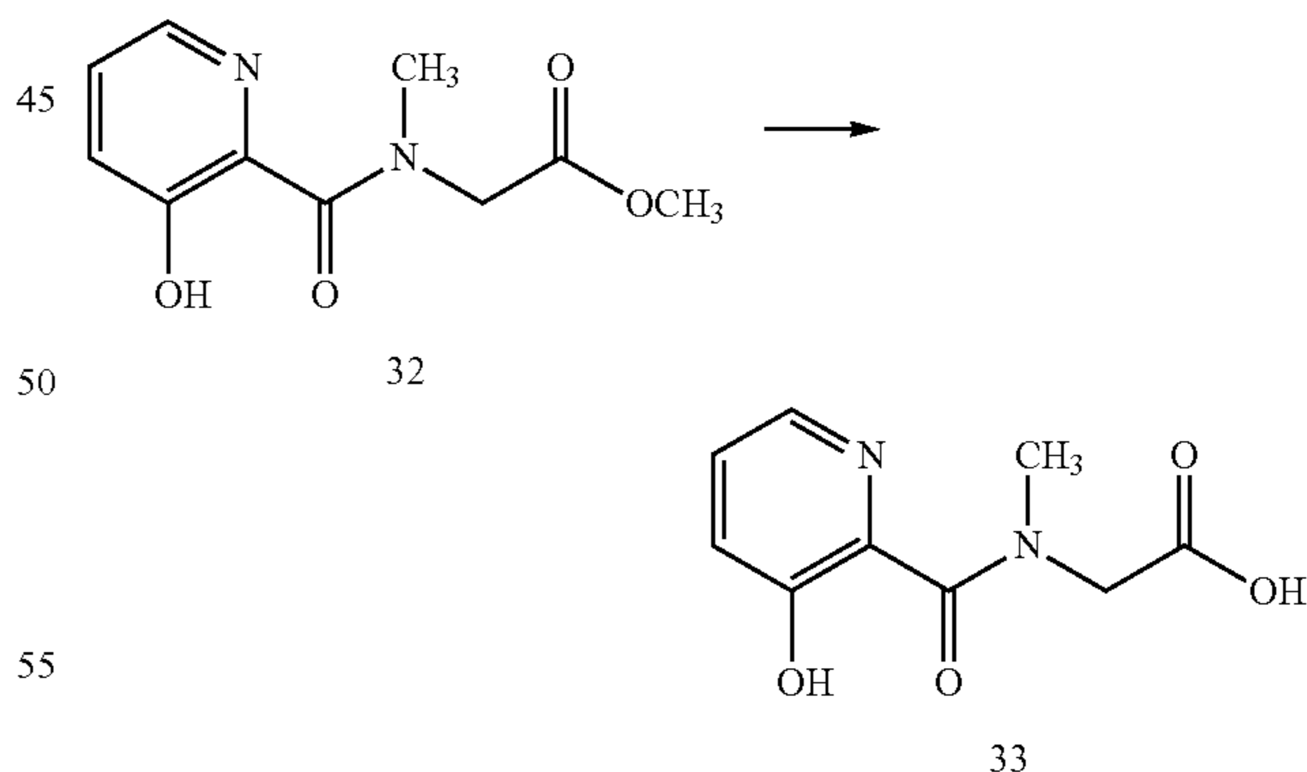
Scheme XX
