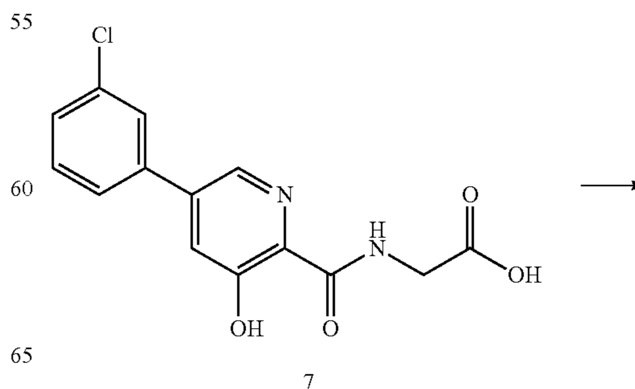
Scheme VII
