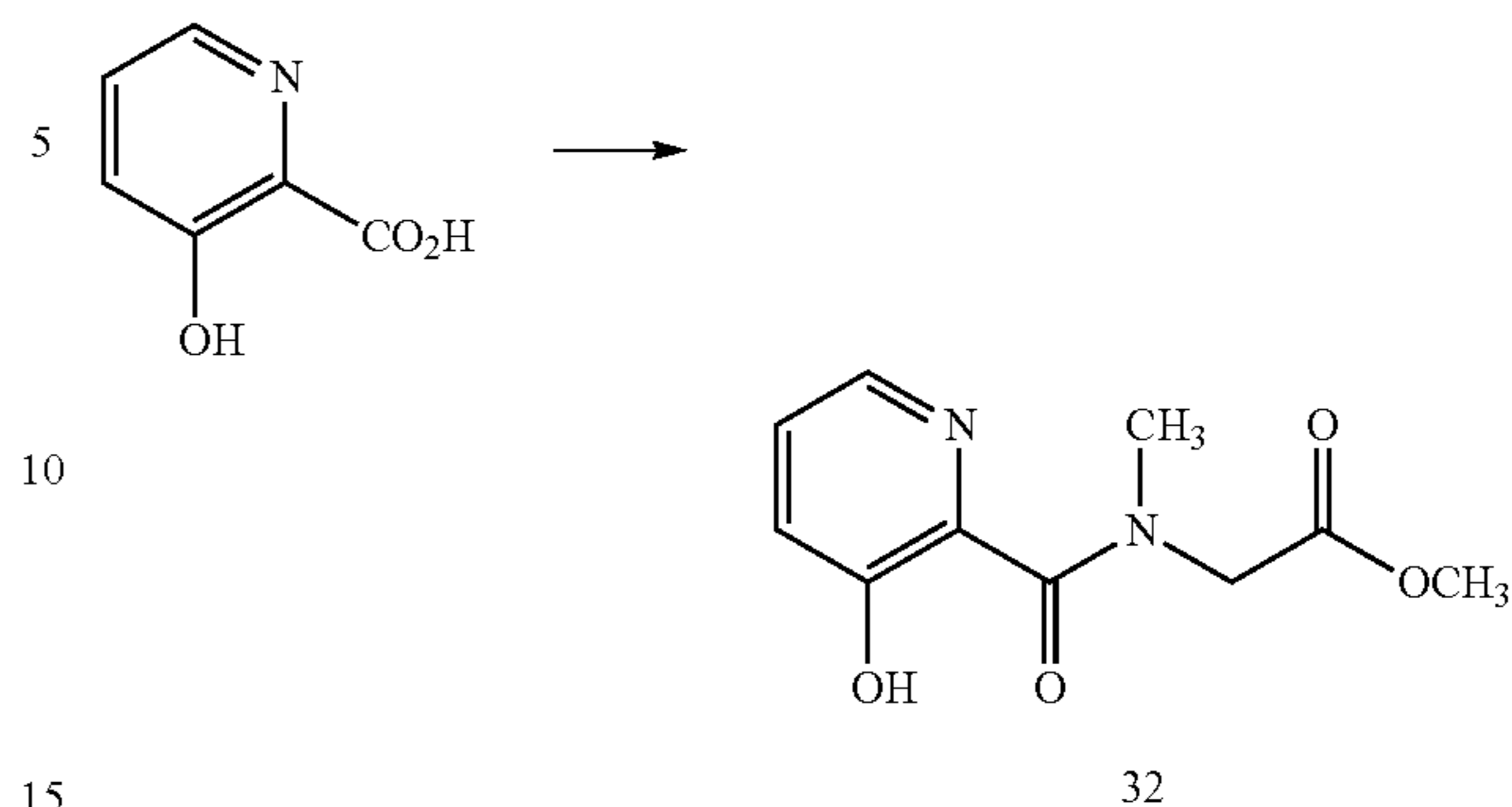
Scheme XIX
