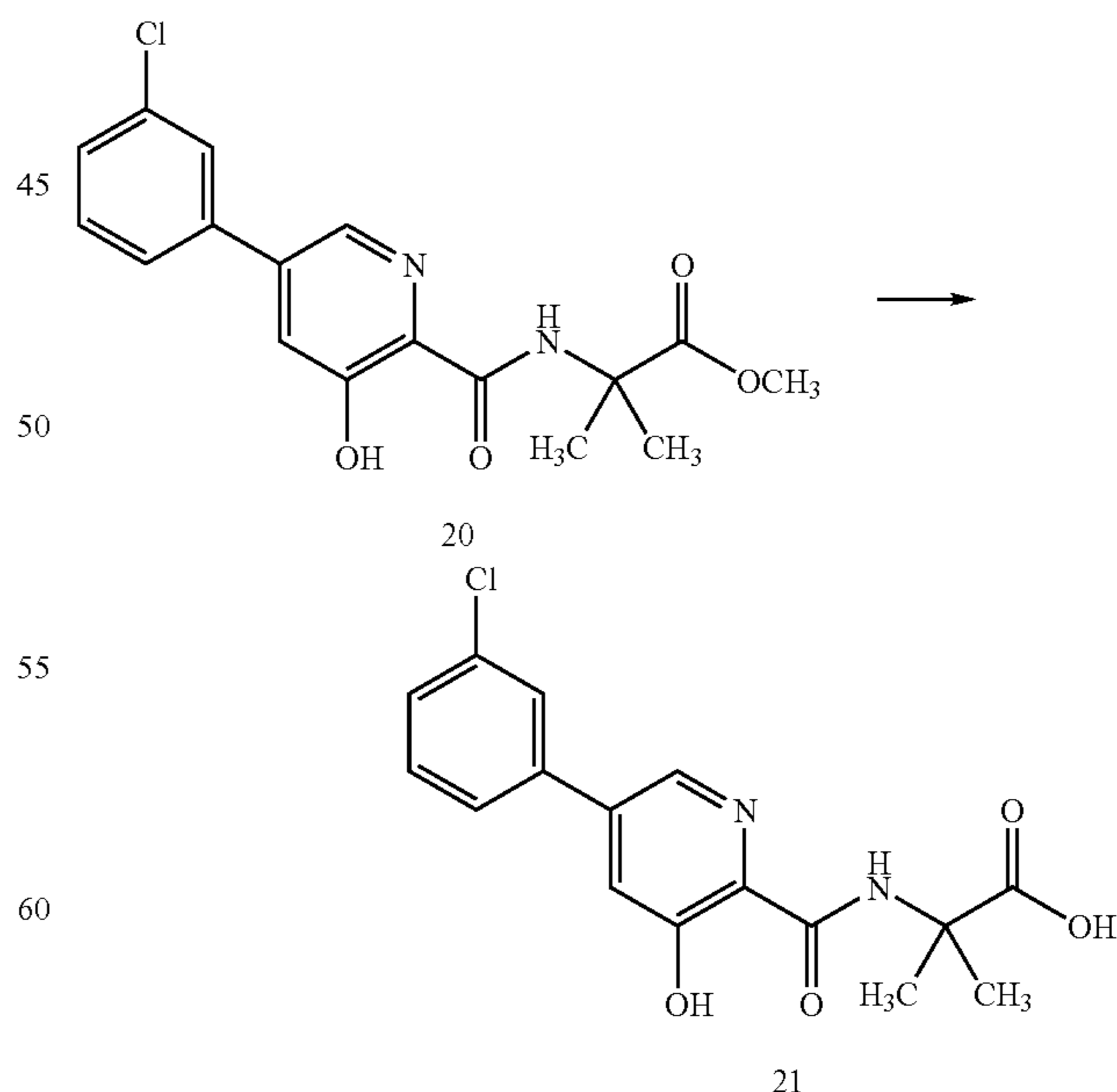
Scheme X
