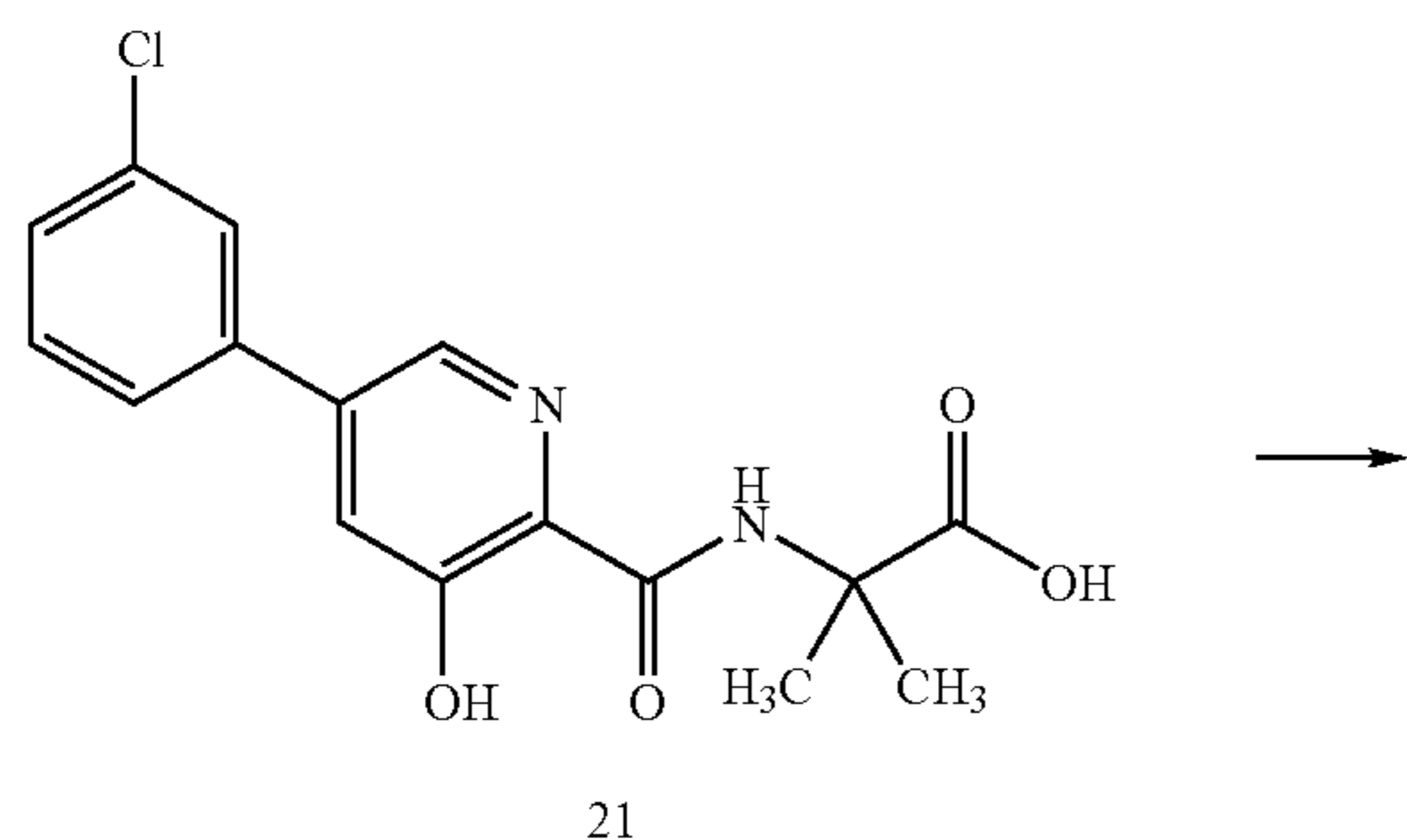
Scheme XI
