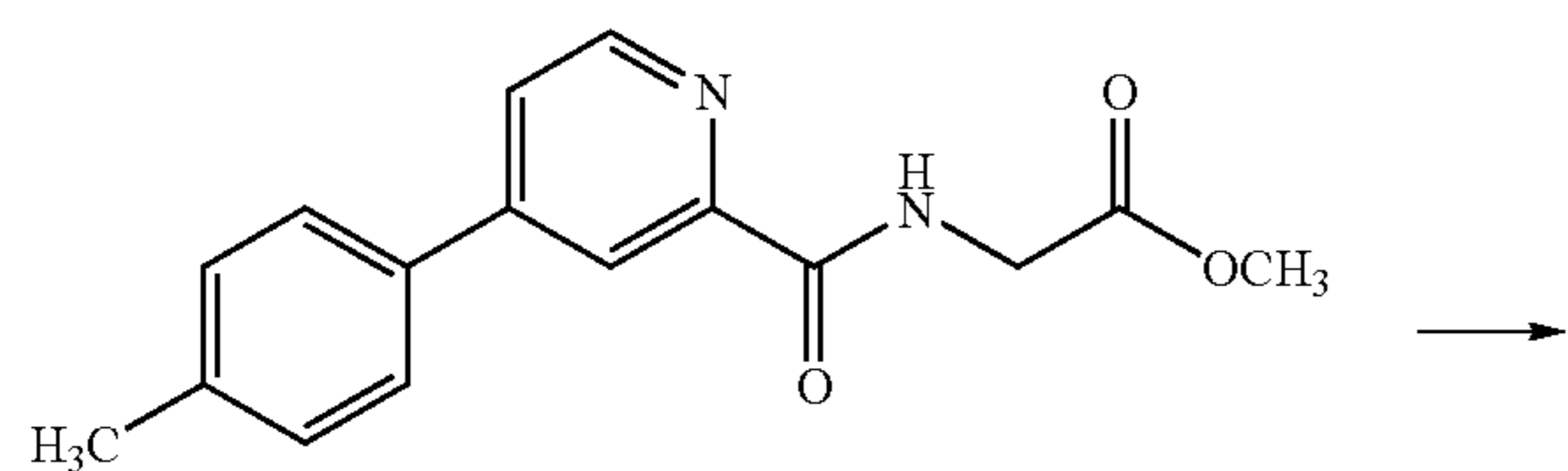
Scheme XIII
