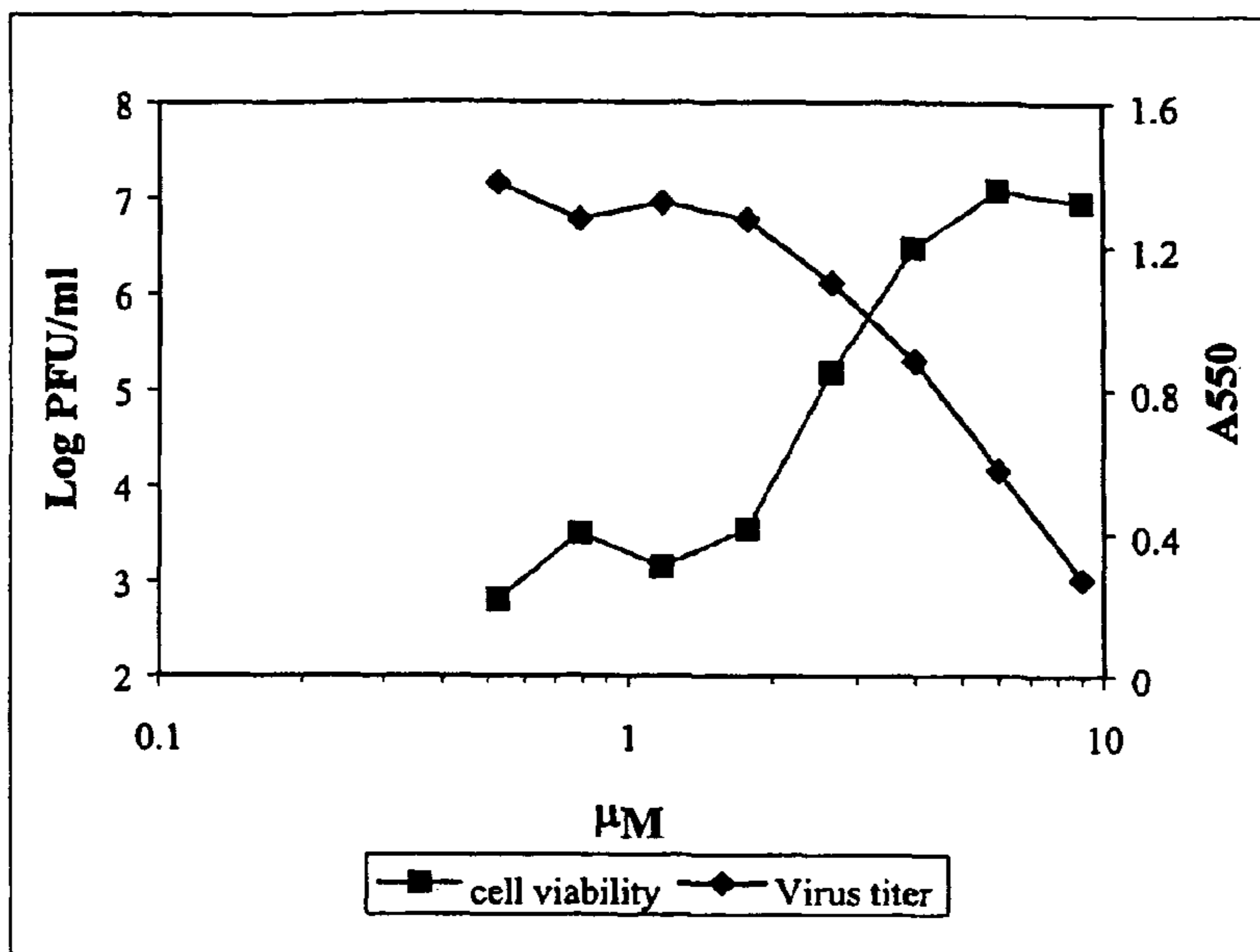
Figure 9: Yield Reduction Assay of \beta -D-2'-CH 3 -riboG
