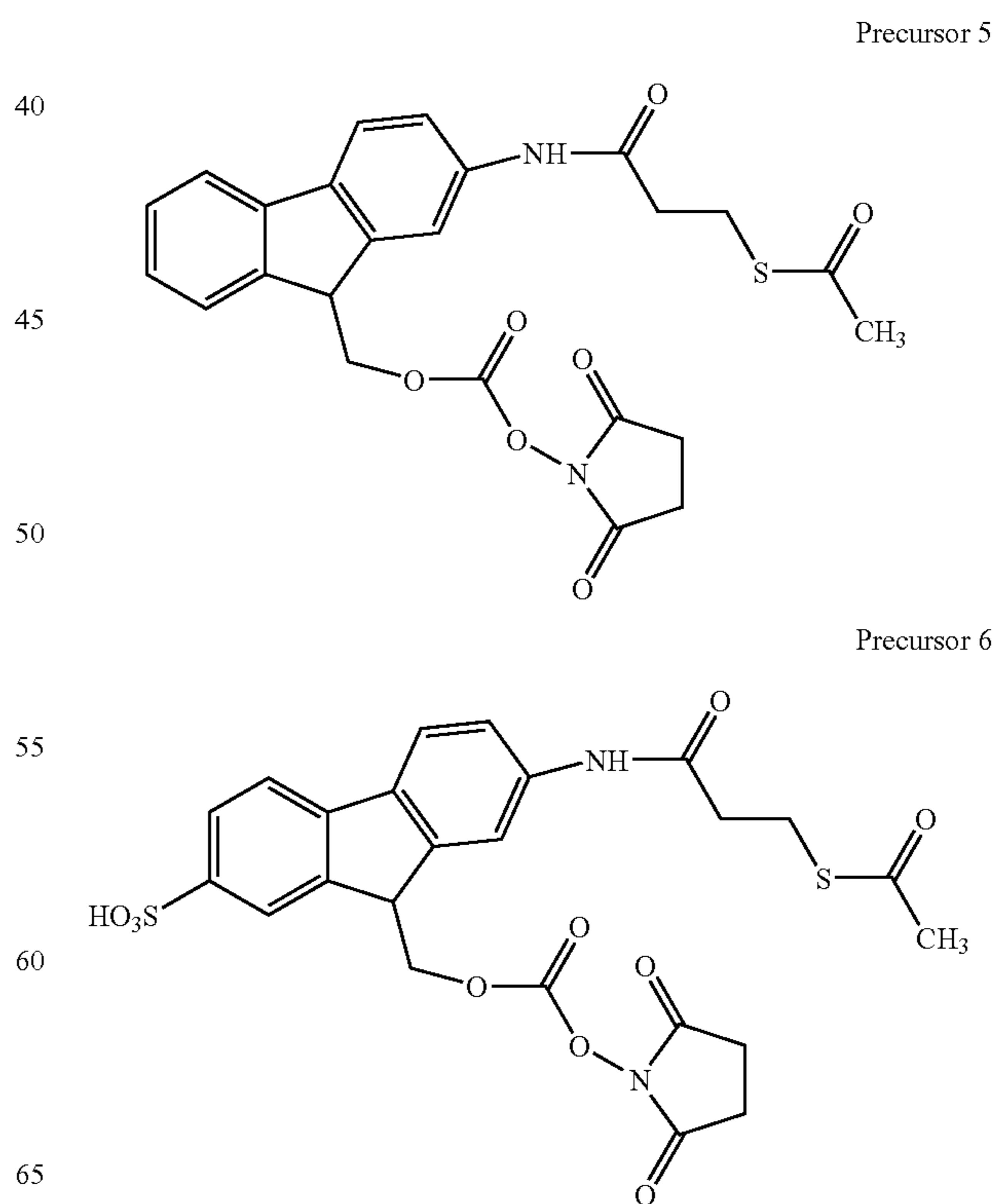
Scheme 3: Precursors 5-8
