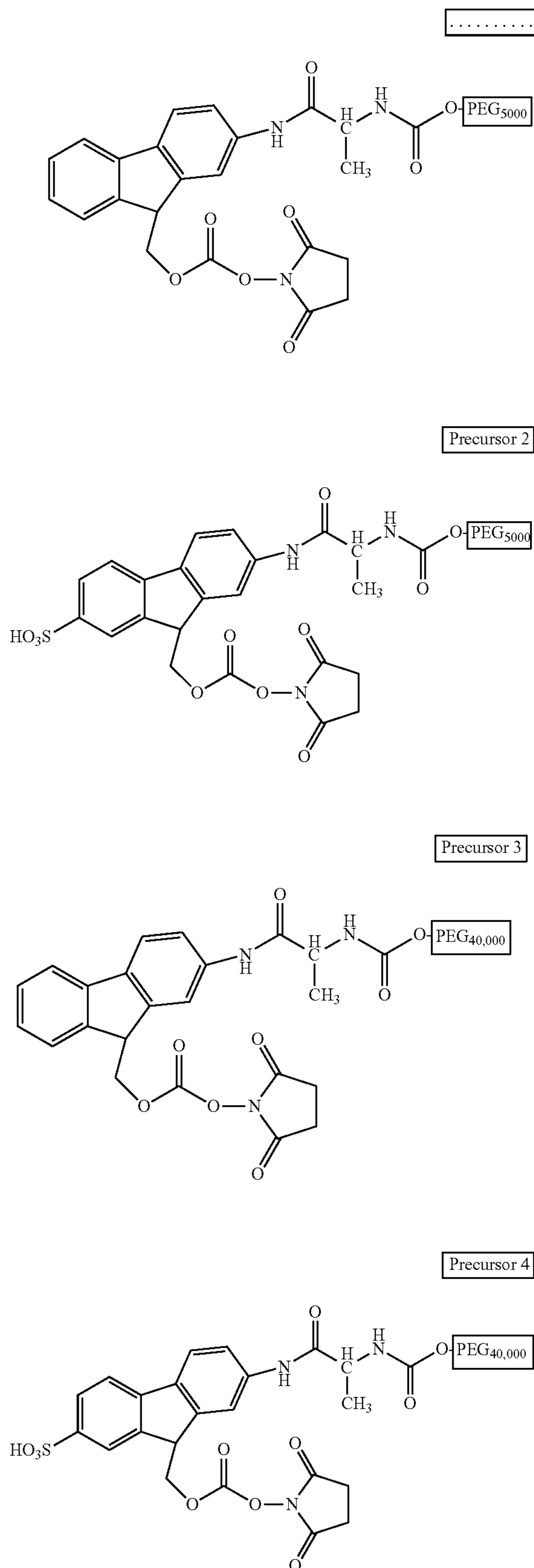
Scheme 1: Precursors 1-4
