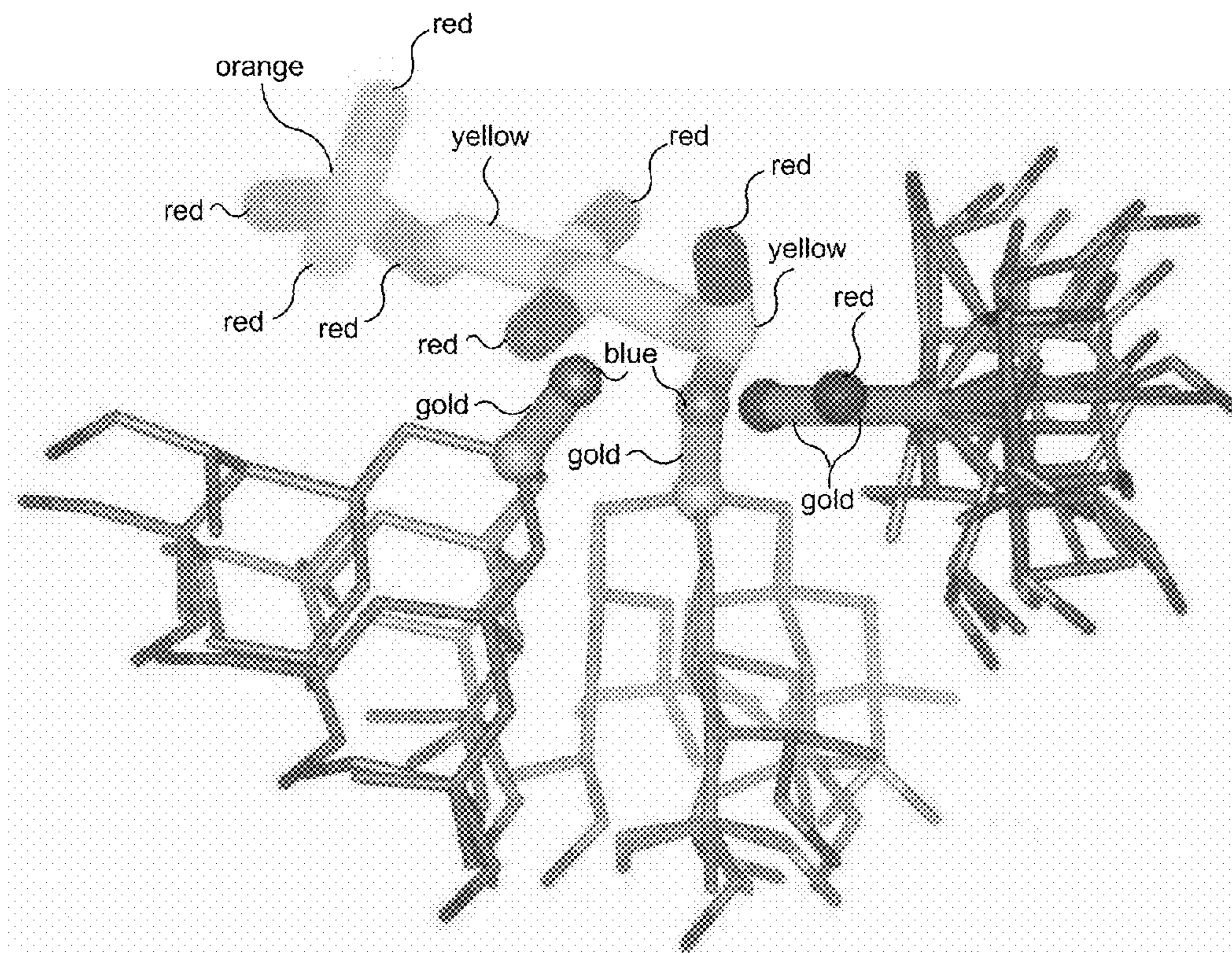
Inverse rotamer tree for deoxyribose-phosphate aldolase (DERA) active site. The transition state is colored in yellow, and the key functional groups of the catalytic residues are in gold. The remainder of the side chains in the rotamer trees are shown using thinner lines in CPK coloring.
