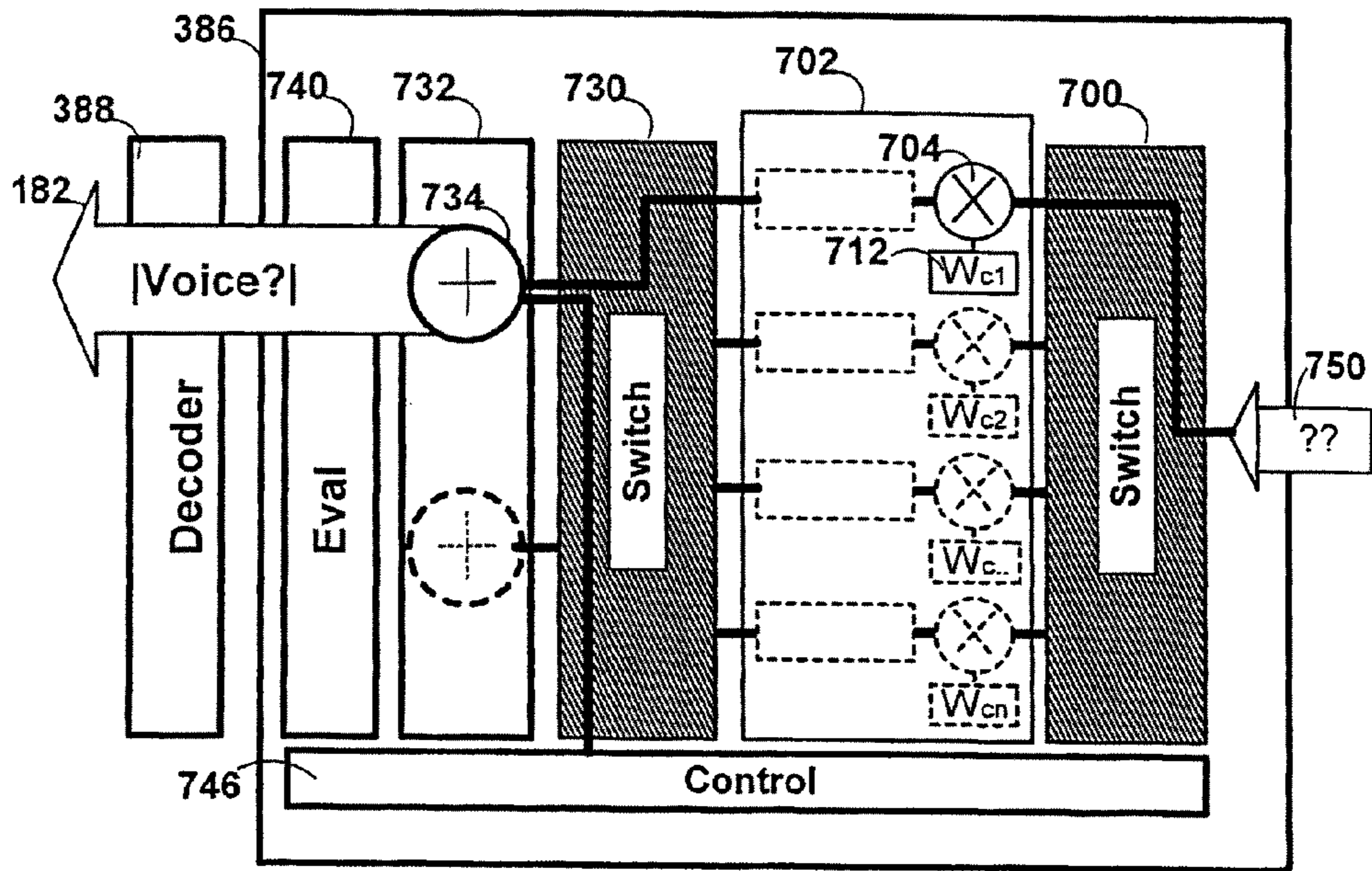
Spatial Processor
