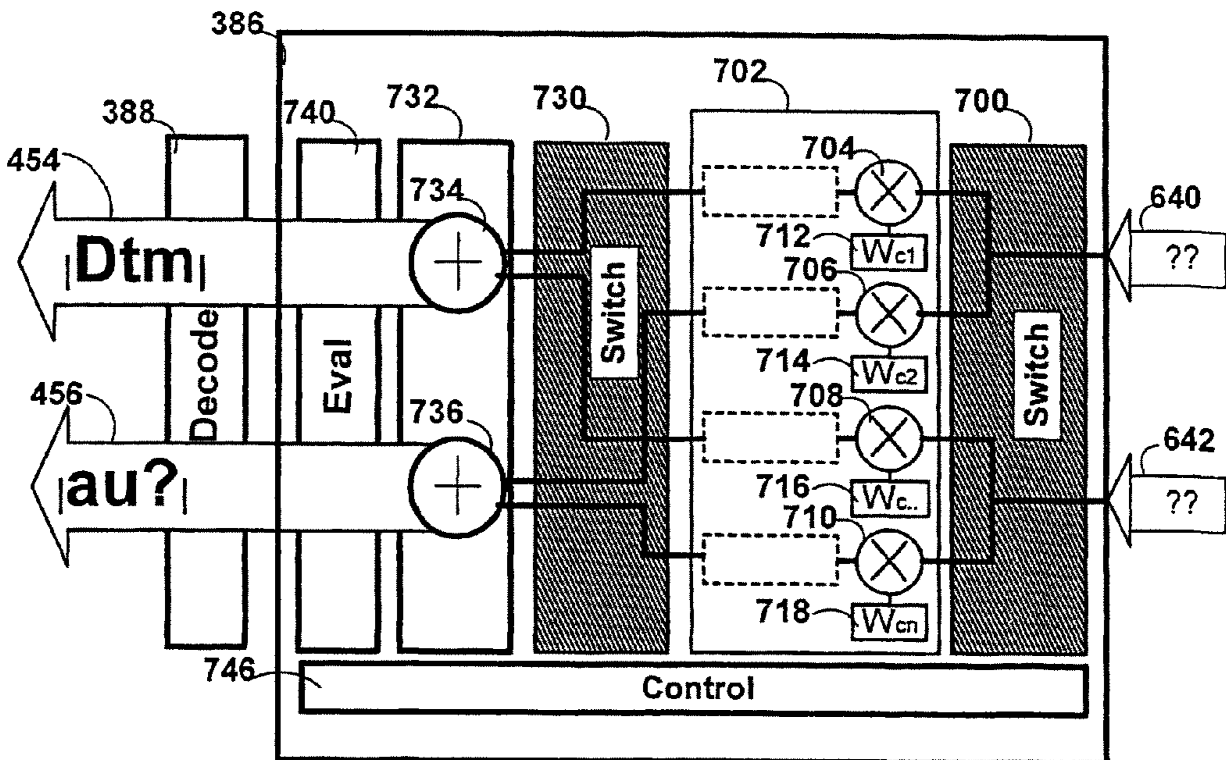
Spatial Processor
