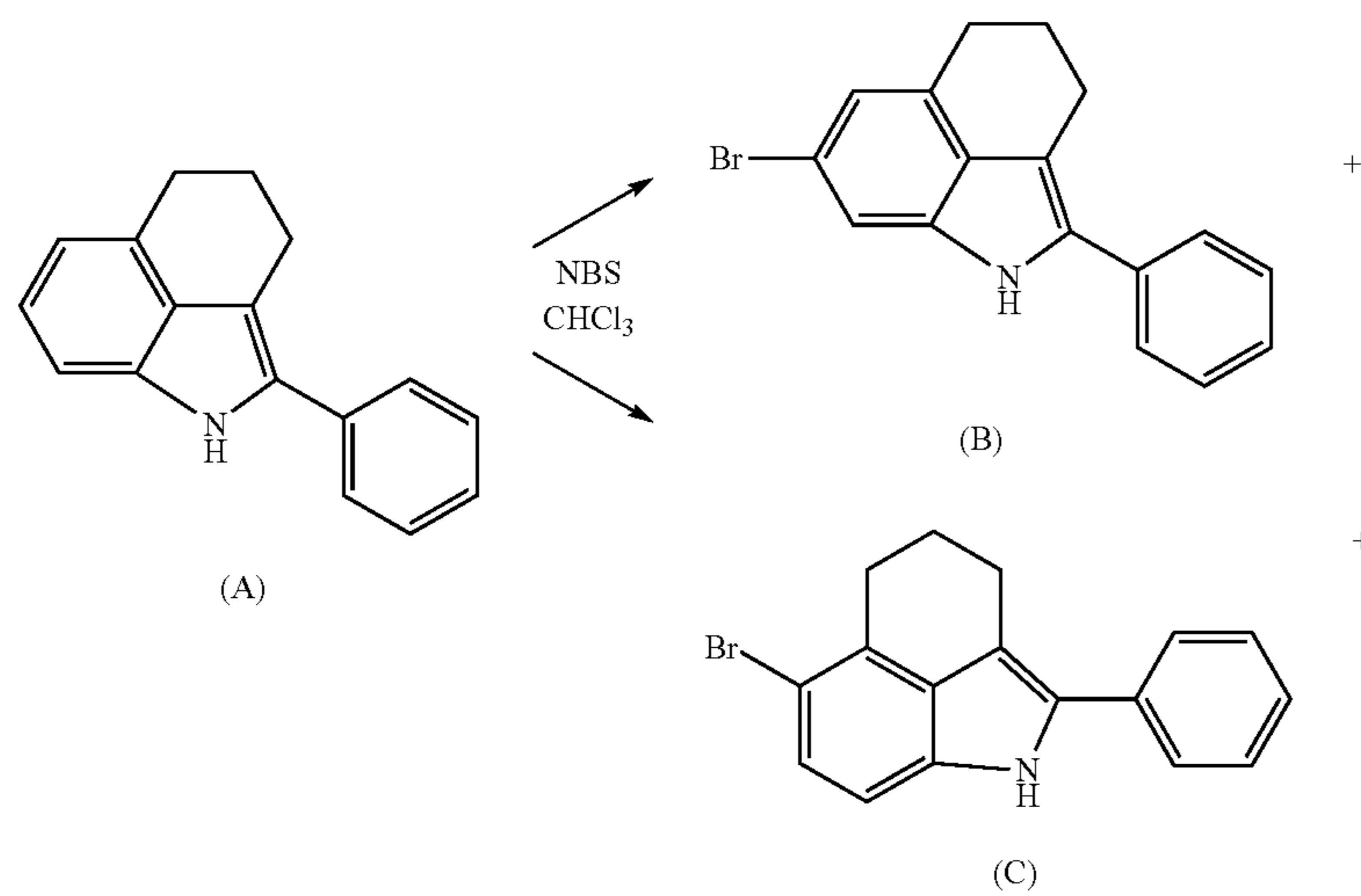
&lt;Reaction Scheme 2&gt;
