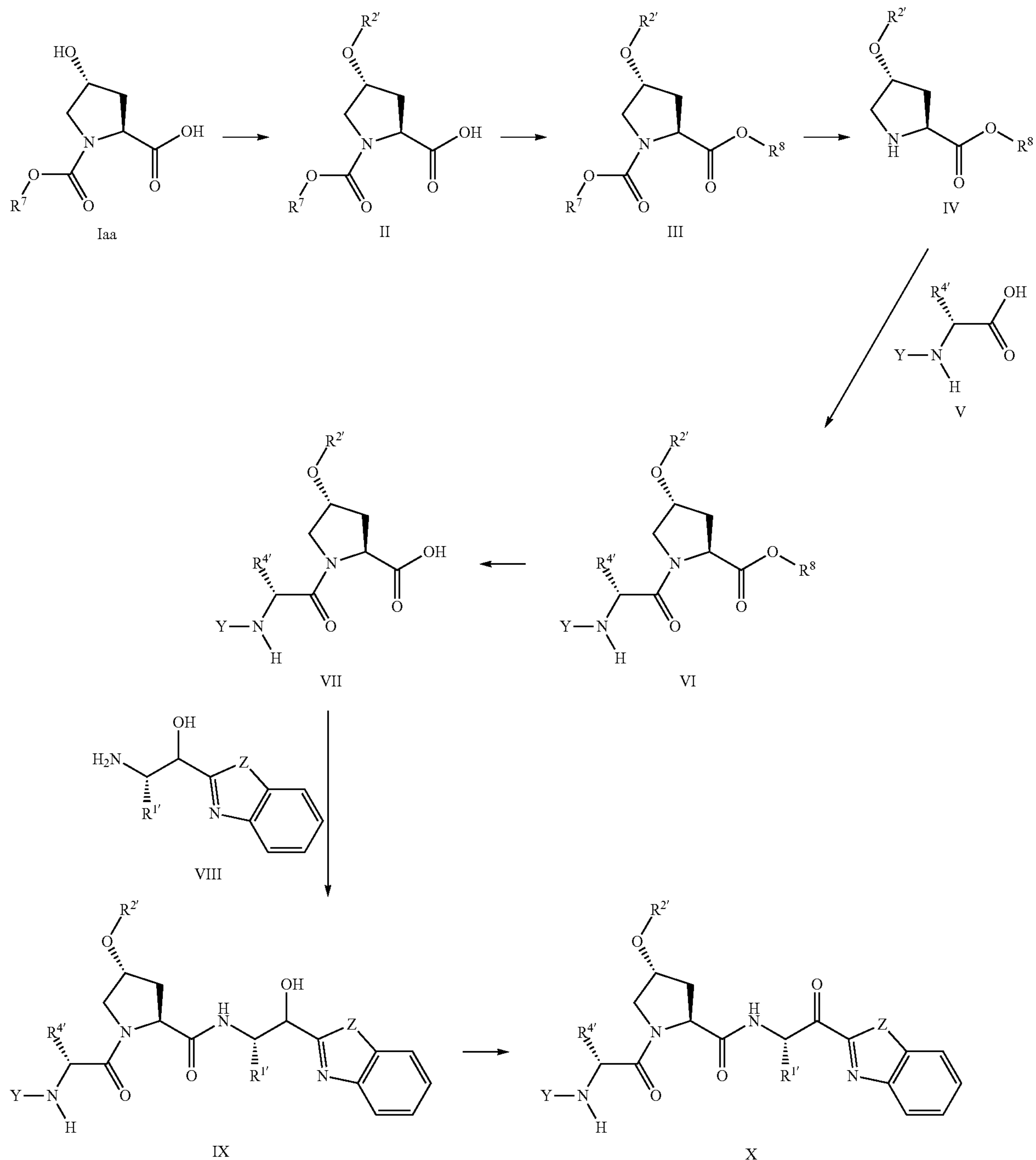
Reaction Scheme I
