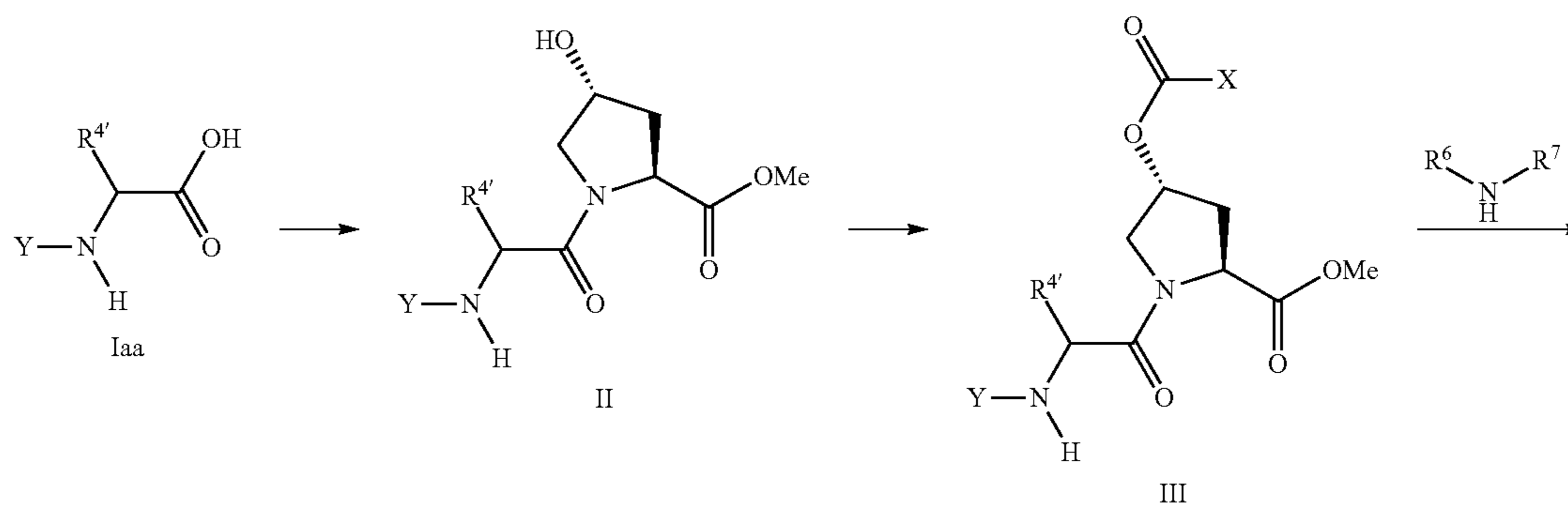
Reaction Scheme III
