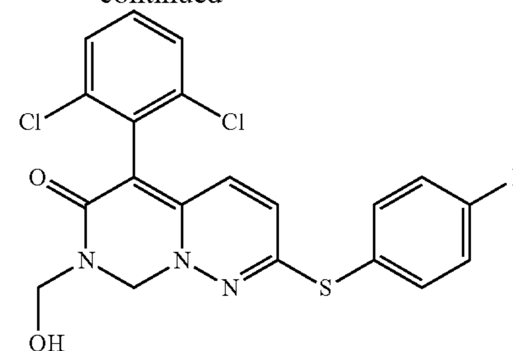
compound 138
