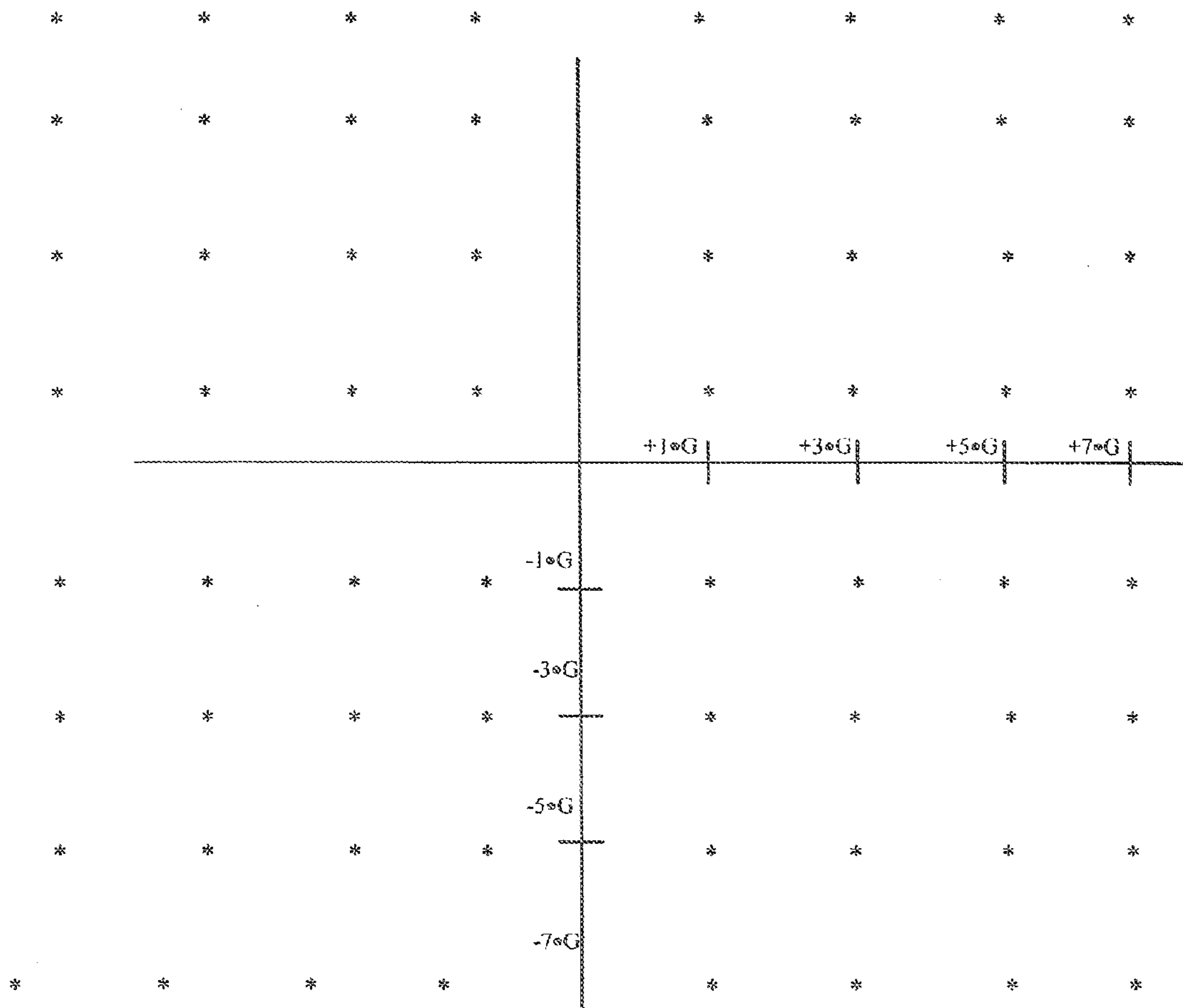
64-QAM Constellation Fig. 3
