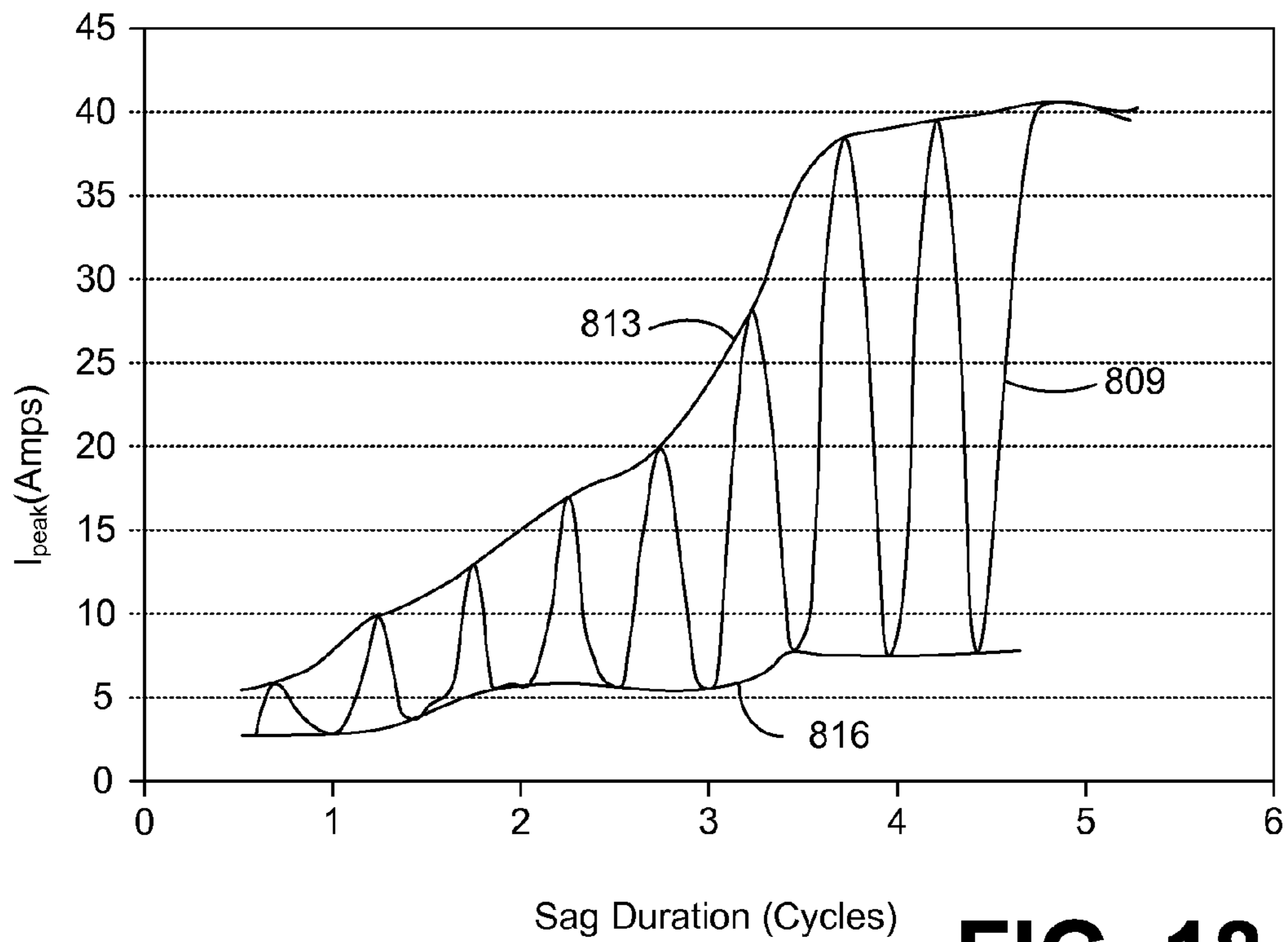
LCD Monitor Current—Inrush Surge
