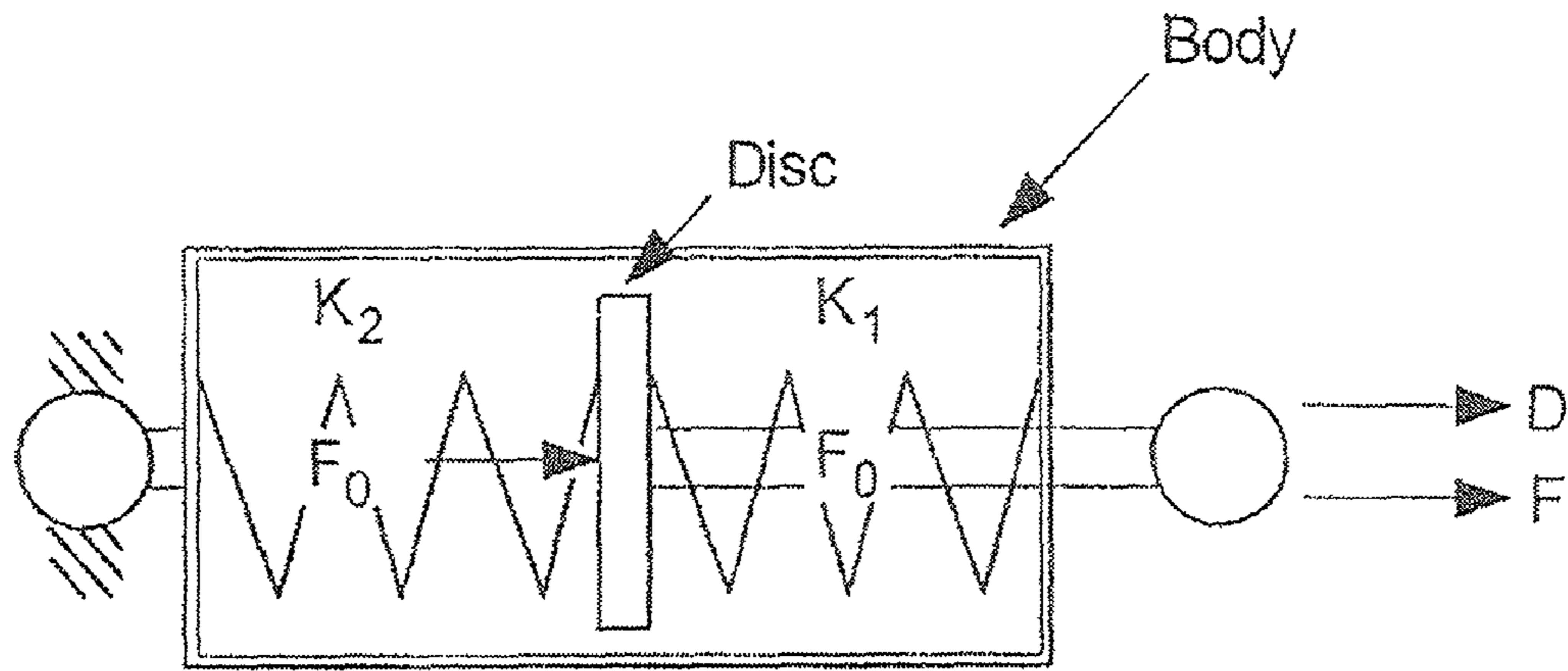
Free-body diagram
