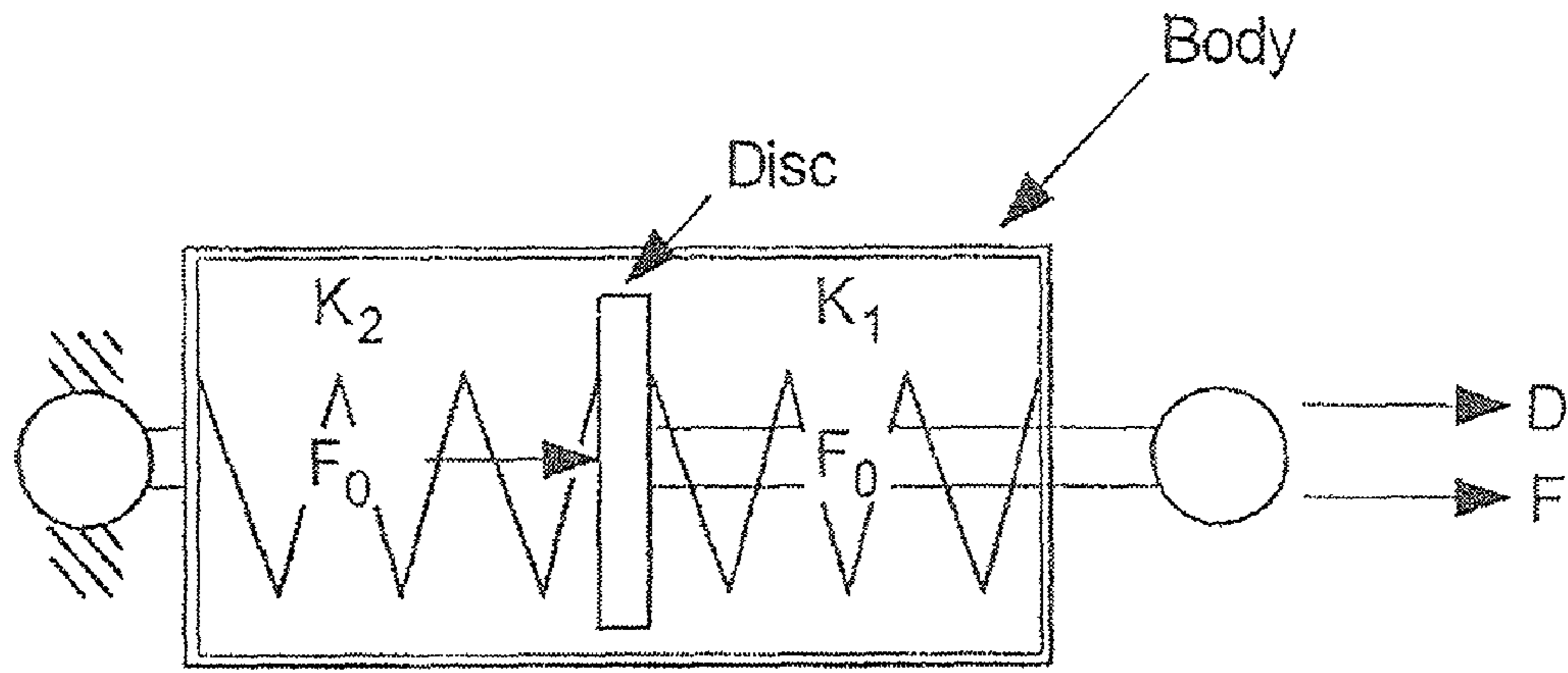
Free-body diagram
