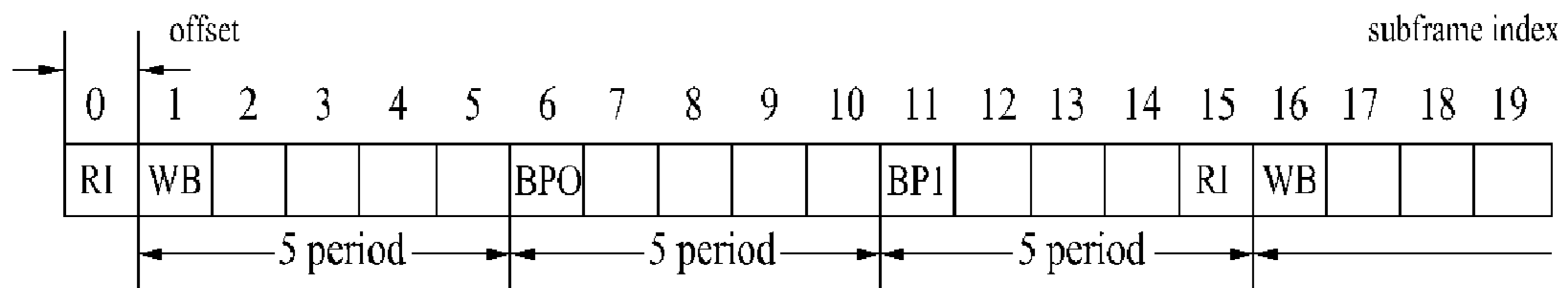
(b) CQI and Rank Indicator(RI)
