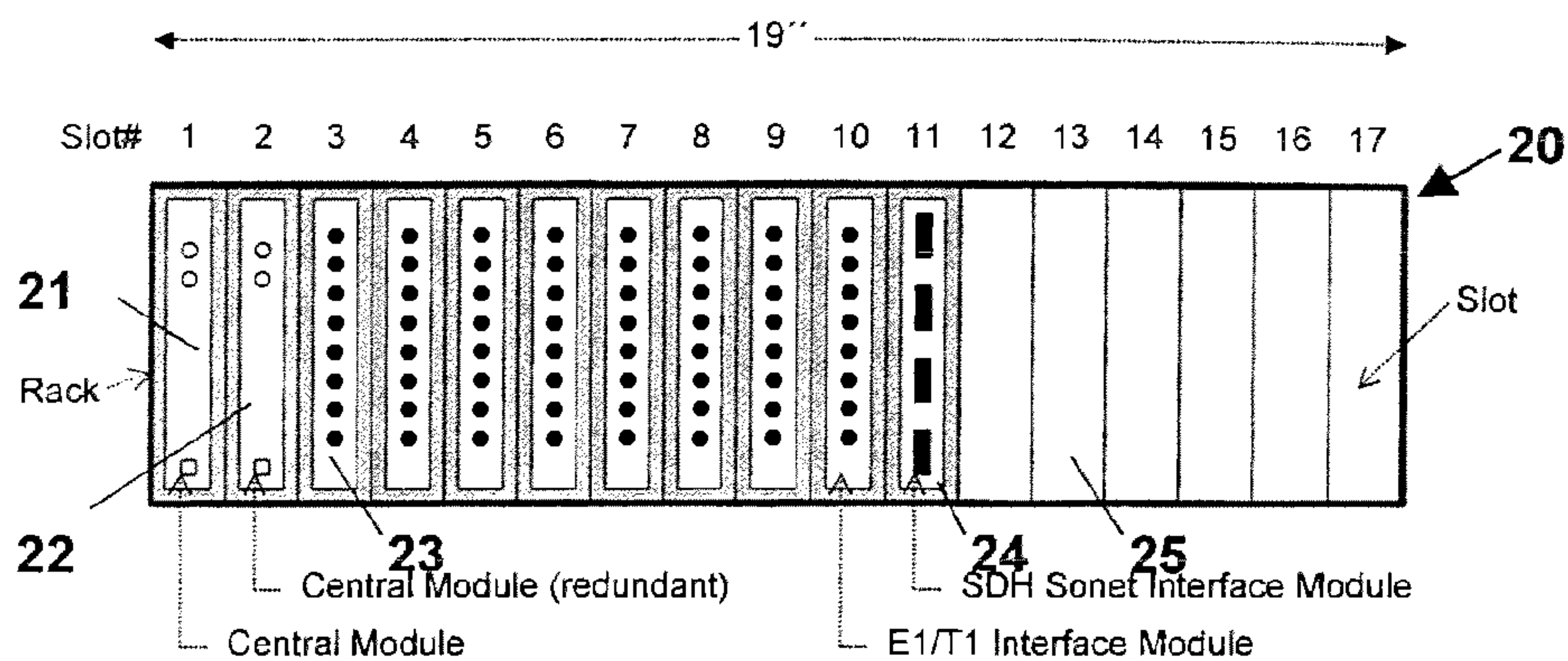
Fig. 1 Conventional rack-based telecommunication node
