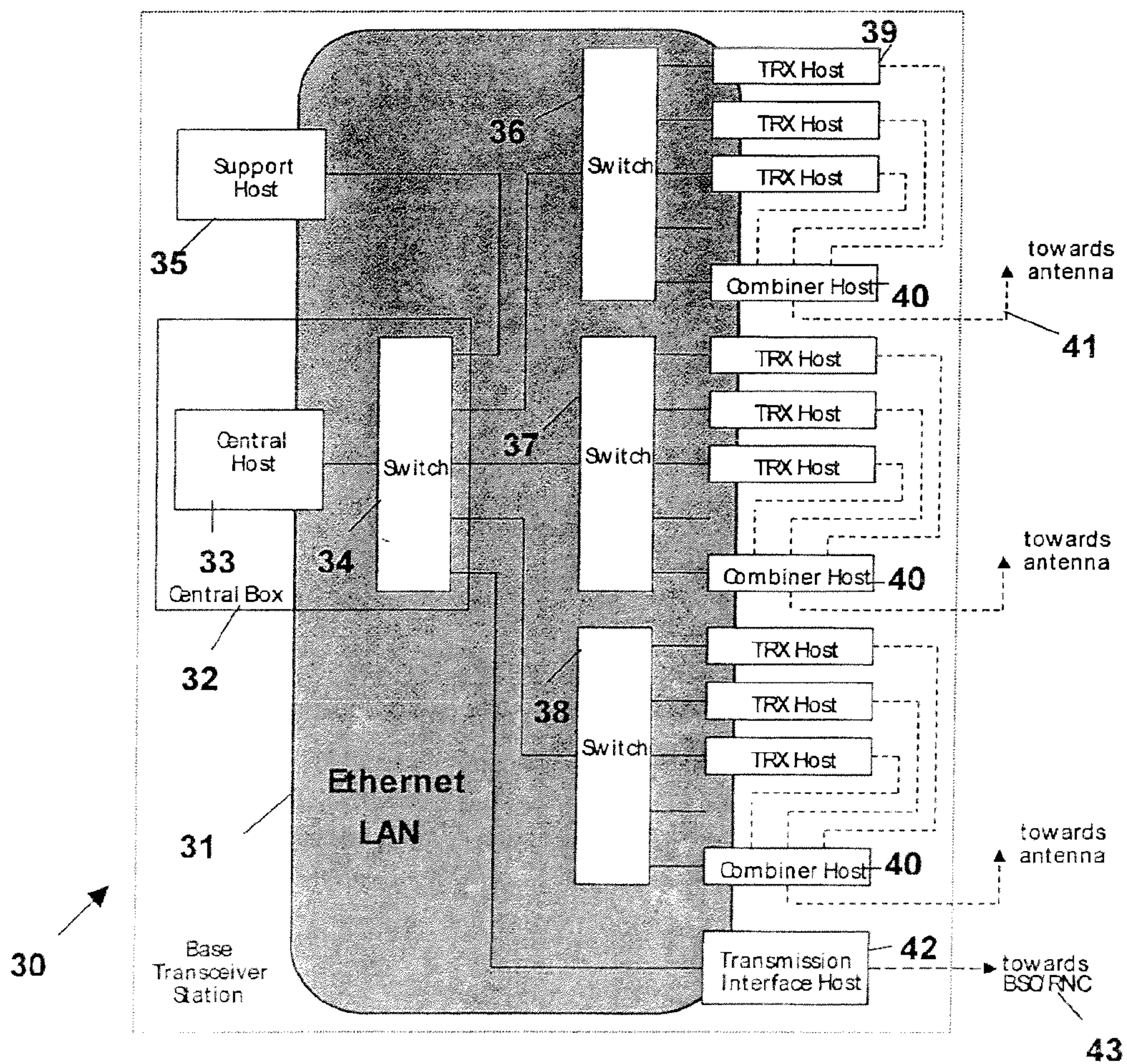
Fig. 2 LAN-based telecommunication node
