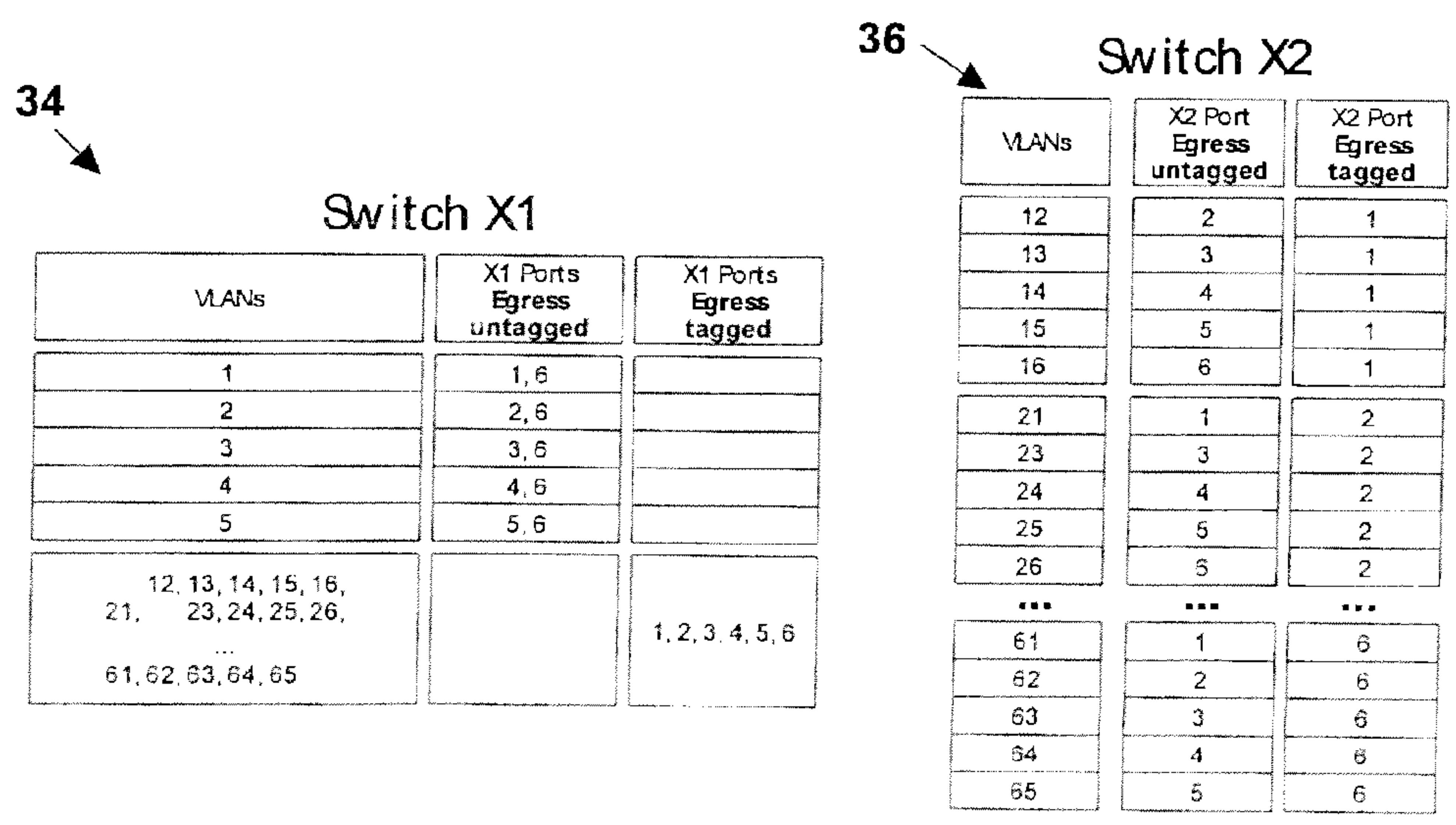
Fig. 6 Switch VLAN configuration
