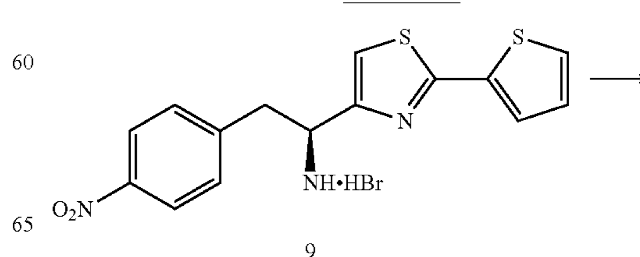
Scheme VIII
