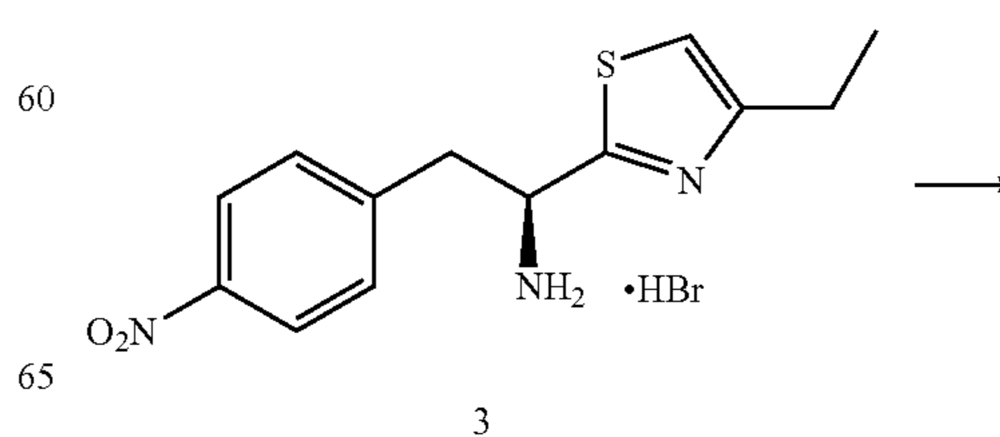
Scheme V
