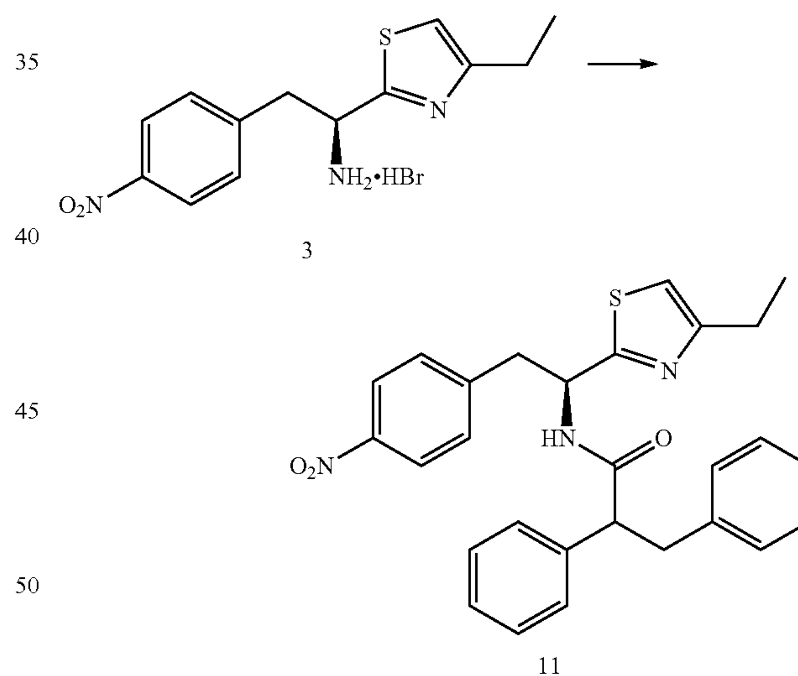
Scheme III
