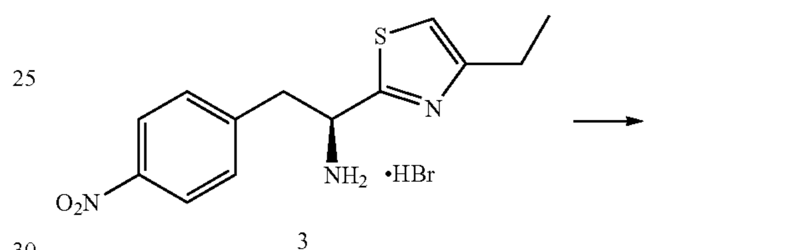
Scheme VII
