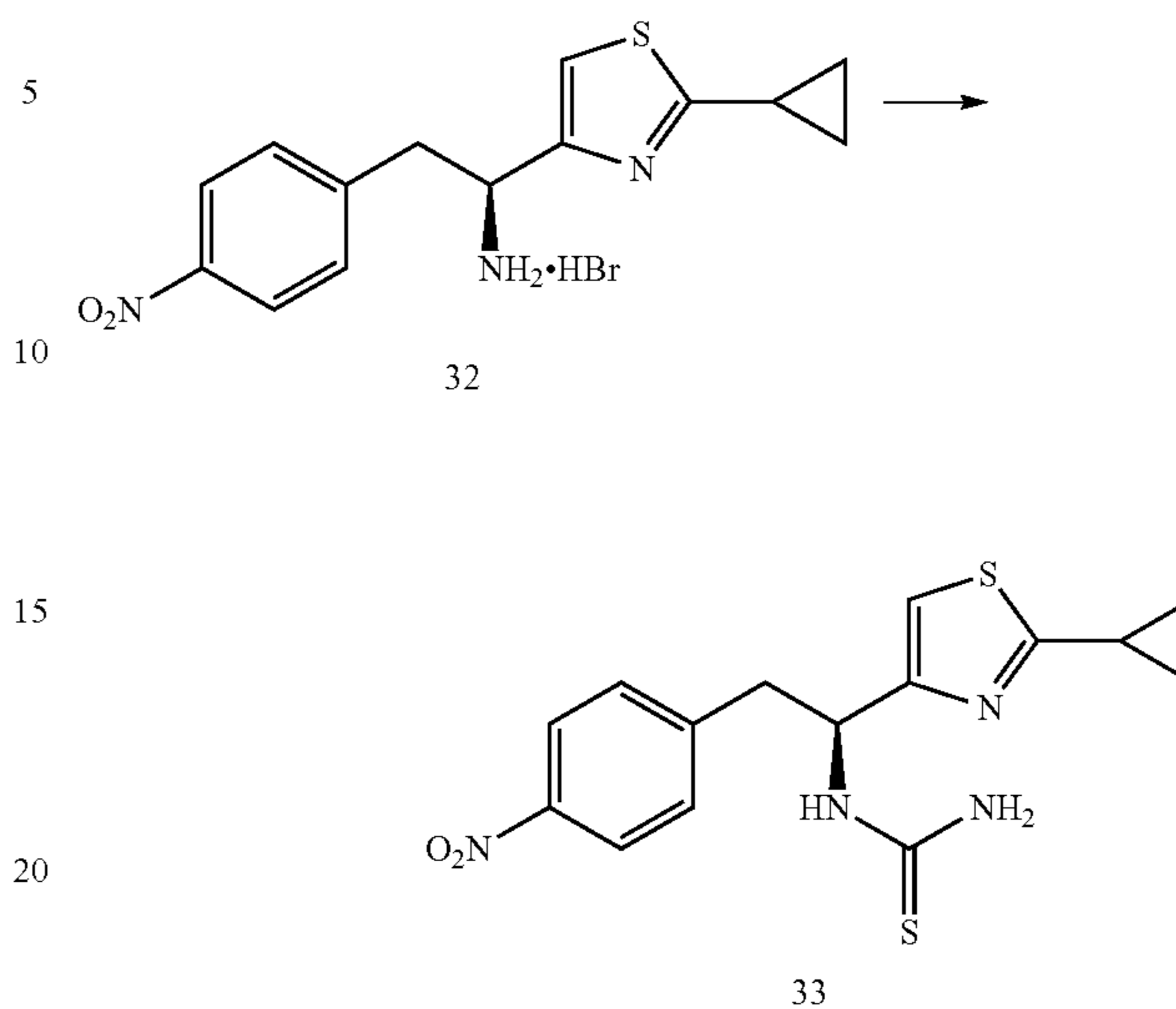
Scheme XII
