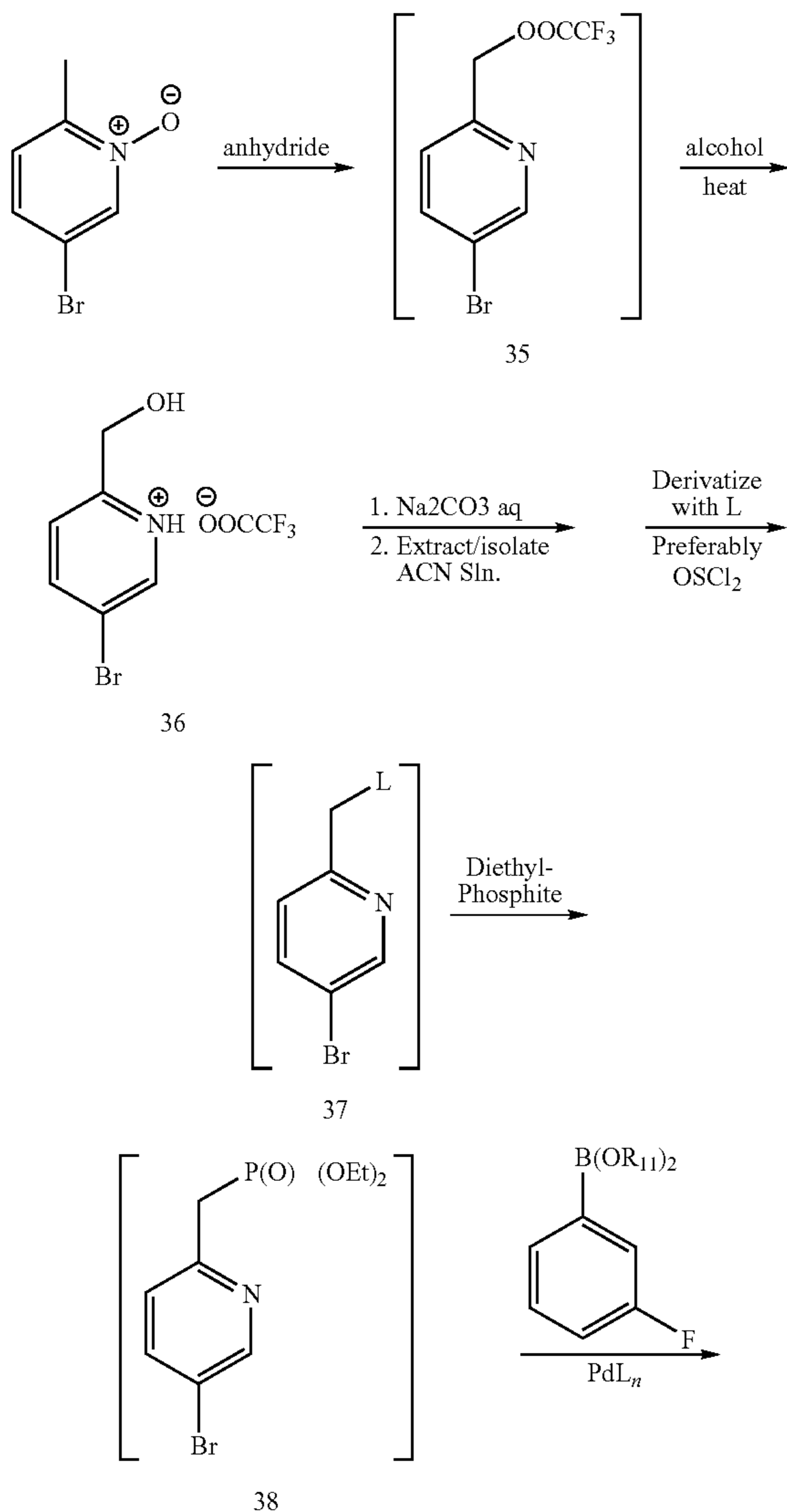
SCHEME II
