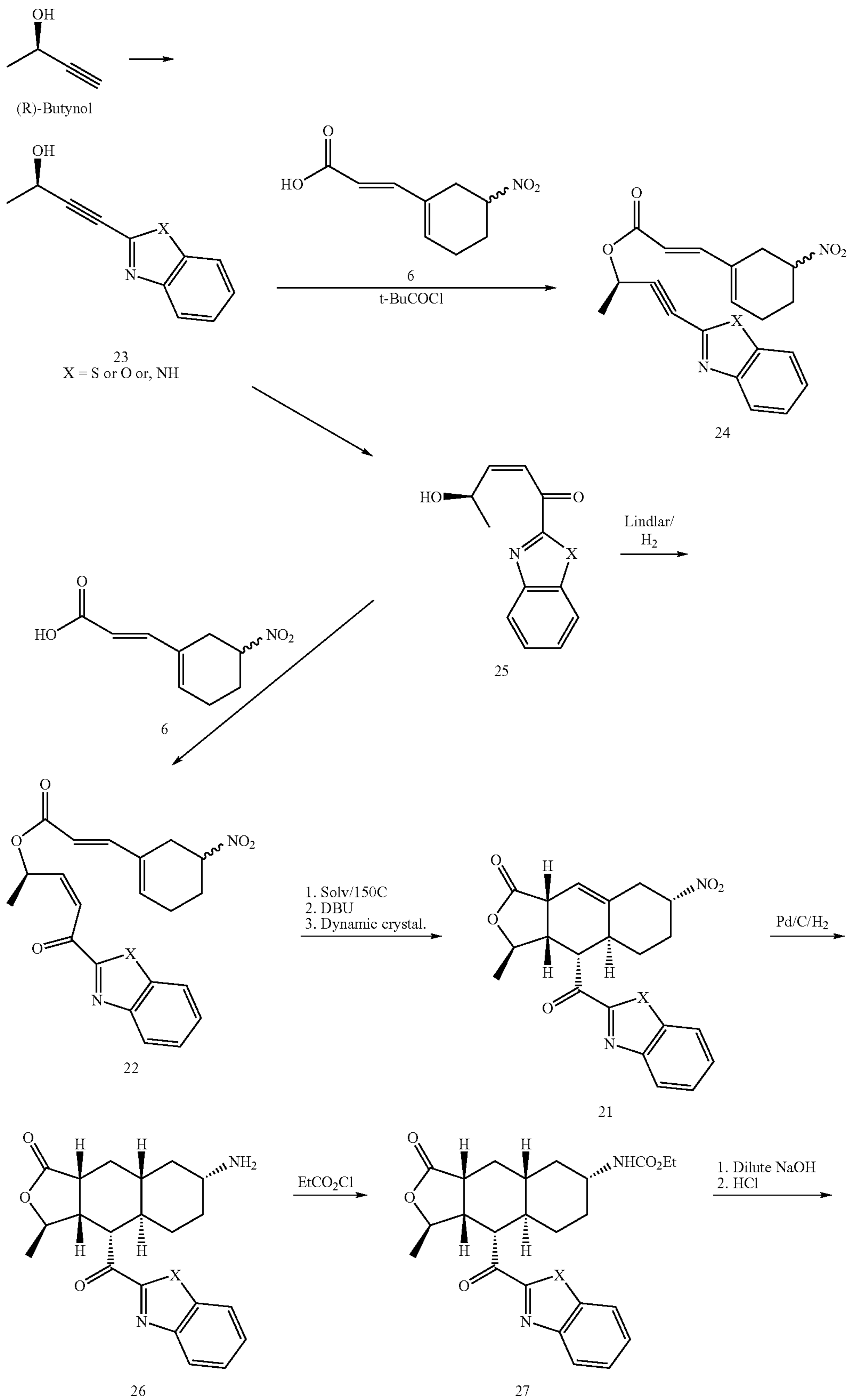
SCHEME V - Nitro-Oxazole Route:
