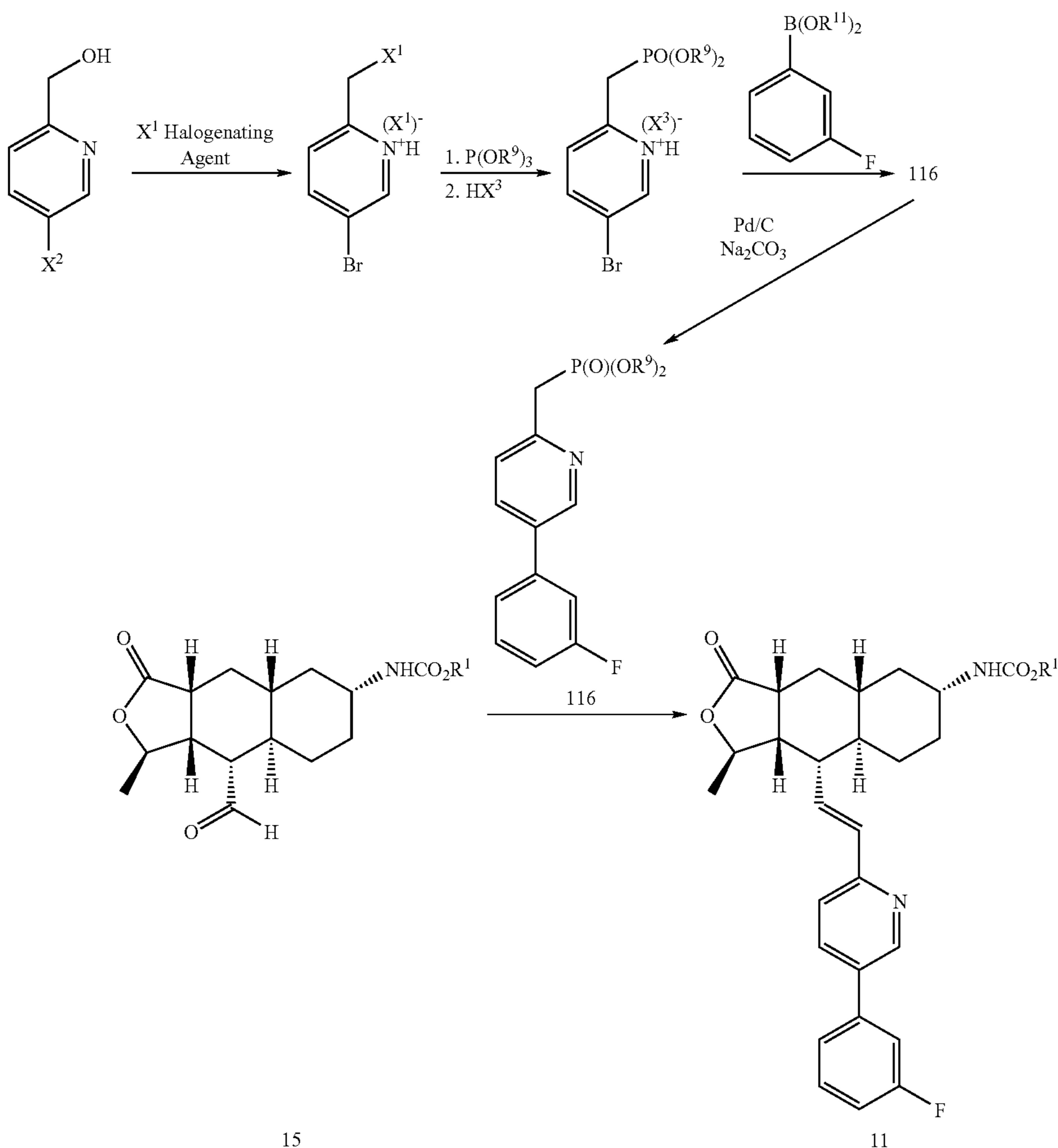
SCHEME III
