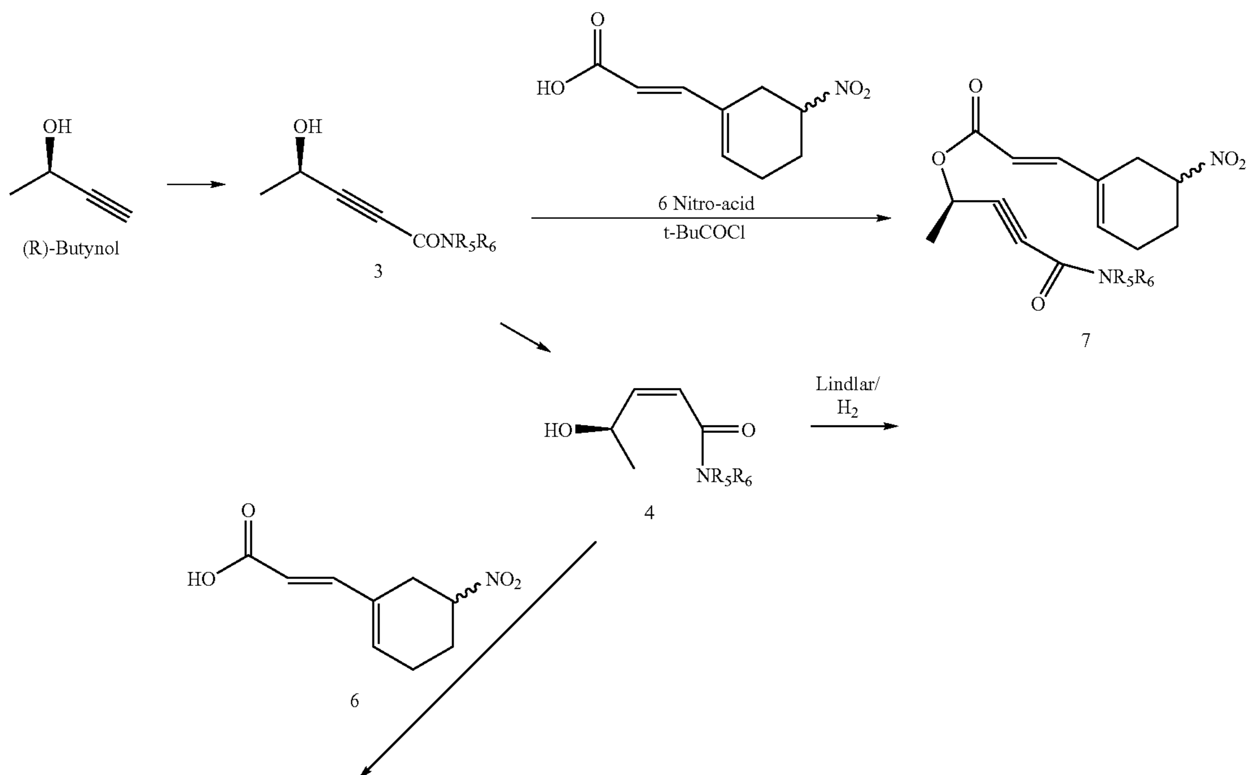
SCHEME IV - Nitro-Ester Route
