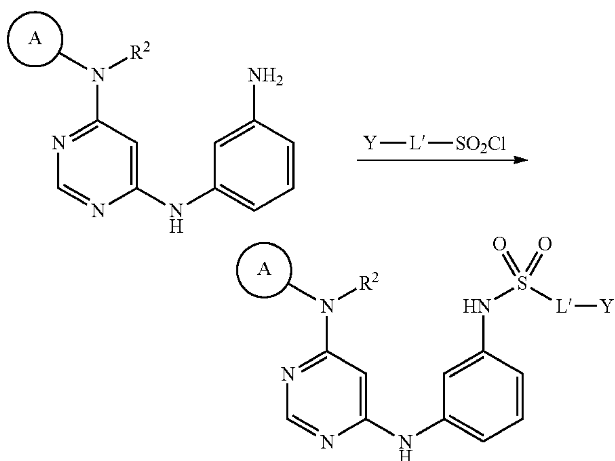
SCHEME 5a Synthesis of N-{3-(6-(arylamino-pyrimidin-4-ylamino)-phenyl)-ethenesulfonamides
