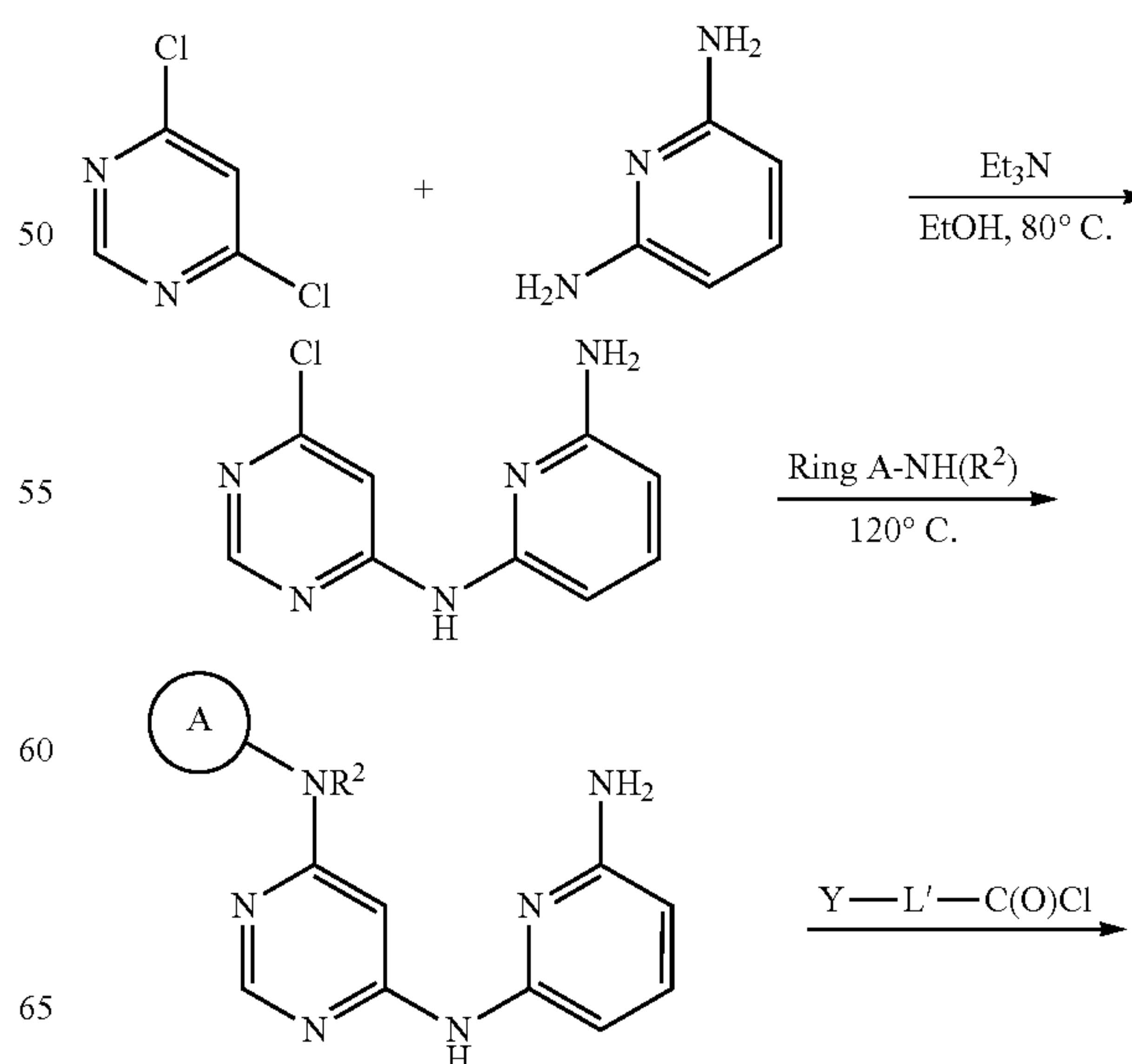
SCHEME 6a Synthesis of N^2 -acylated 6-(6-mono or disubstituted-aminopyrimidin-4-yl)amino-2-aminopyridines
