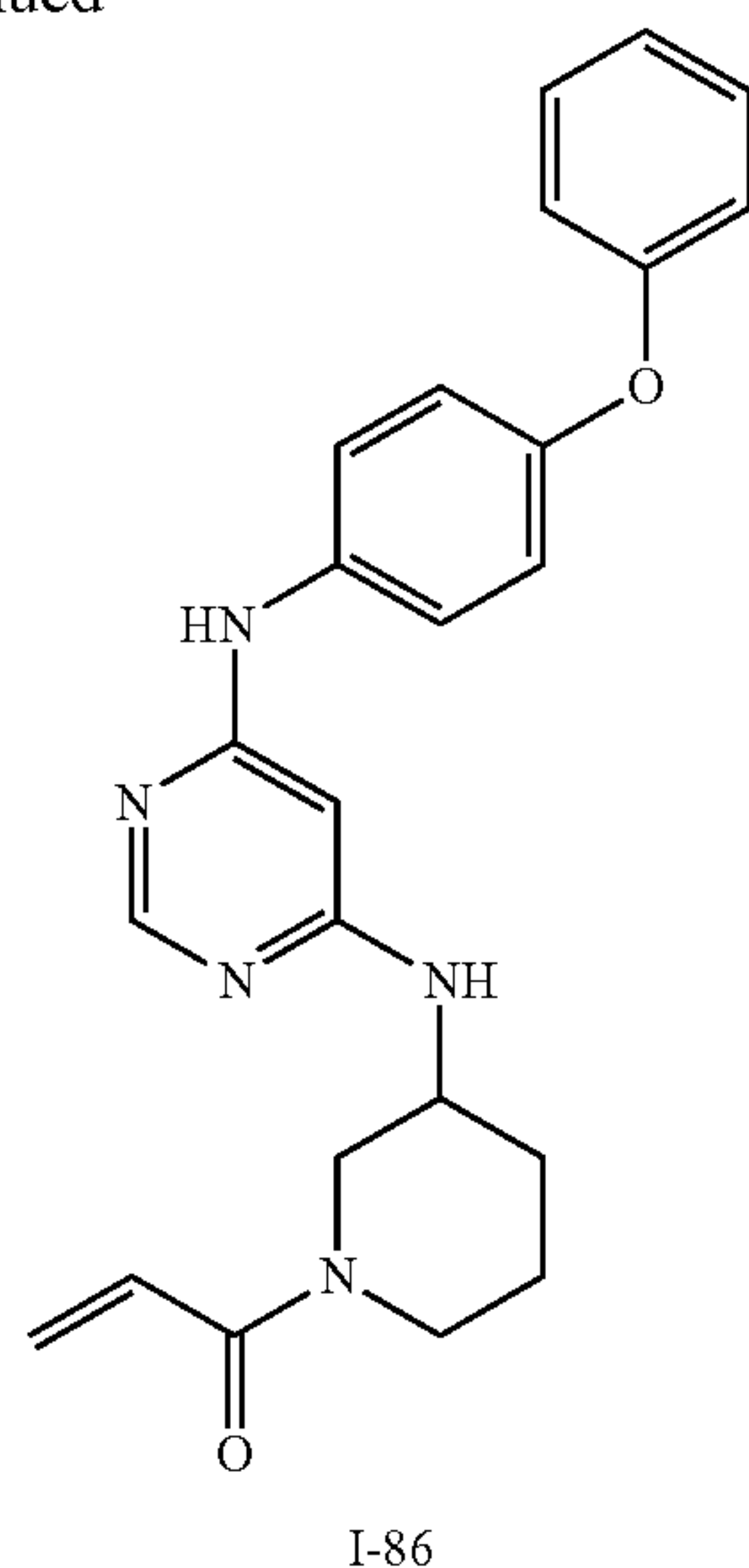
Synthesis of 1-(3-(6-(4-phenoxyphenylamino)pyrimidin-4-ylamino)piperidin-1-yl)prop-2-en-1-one (I-86)
