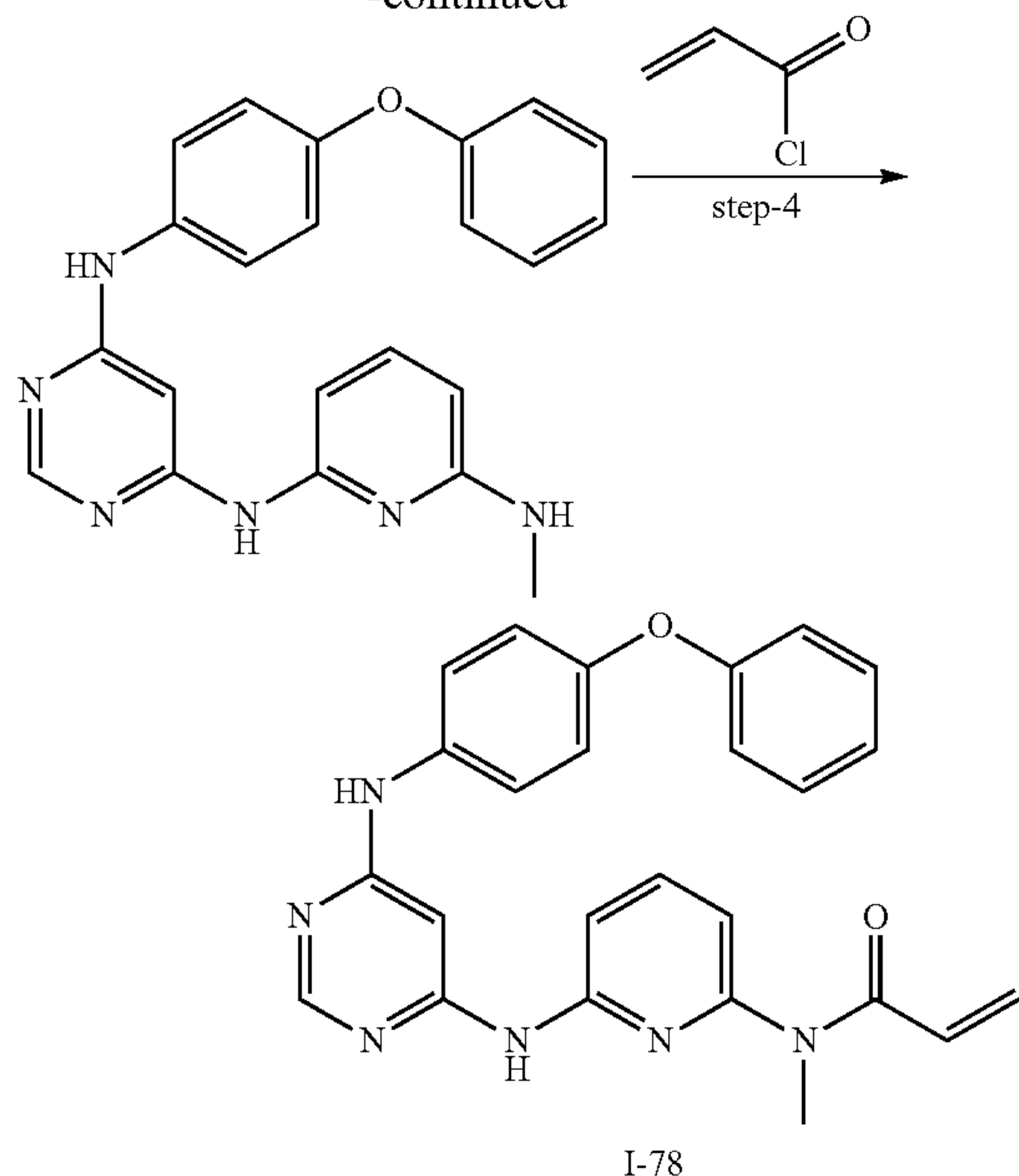
Synthesis of N-methyl-N-(6-(6-(4-phenoxyphenylamino)pyrimidin-4-ylamino)pyridin-2-yl)acrylamide (I-78)
