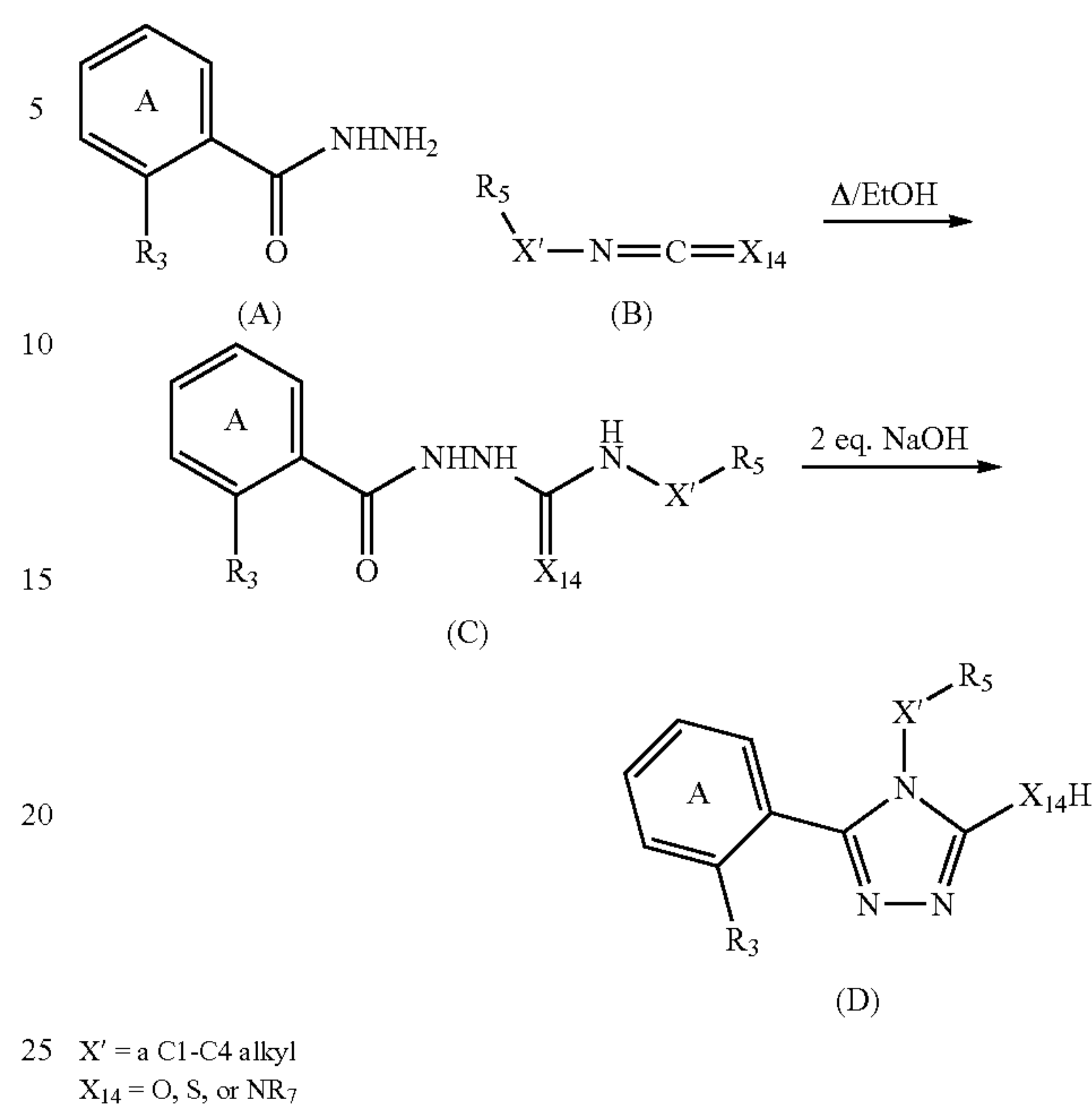
Scheme I: Synthesis of triazole compounds of the invention
