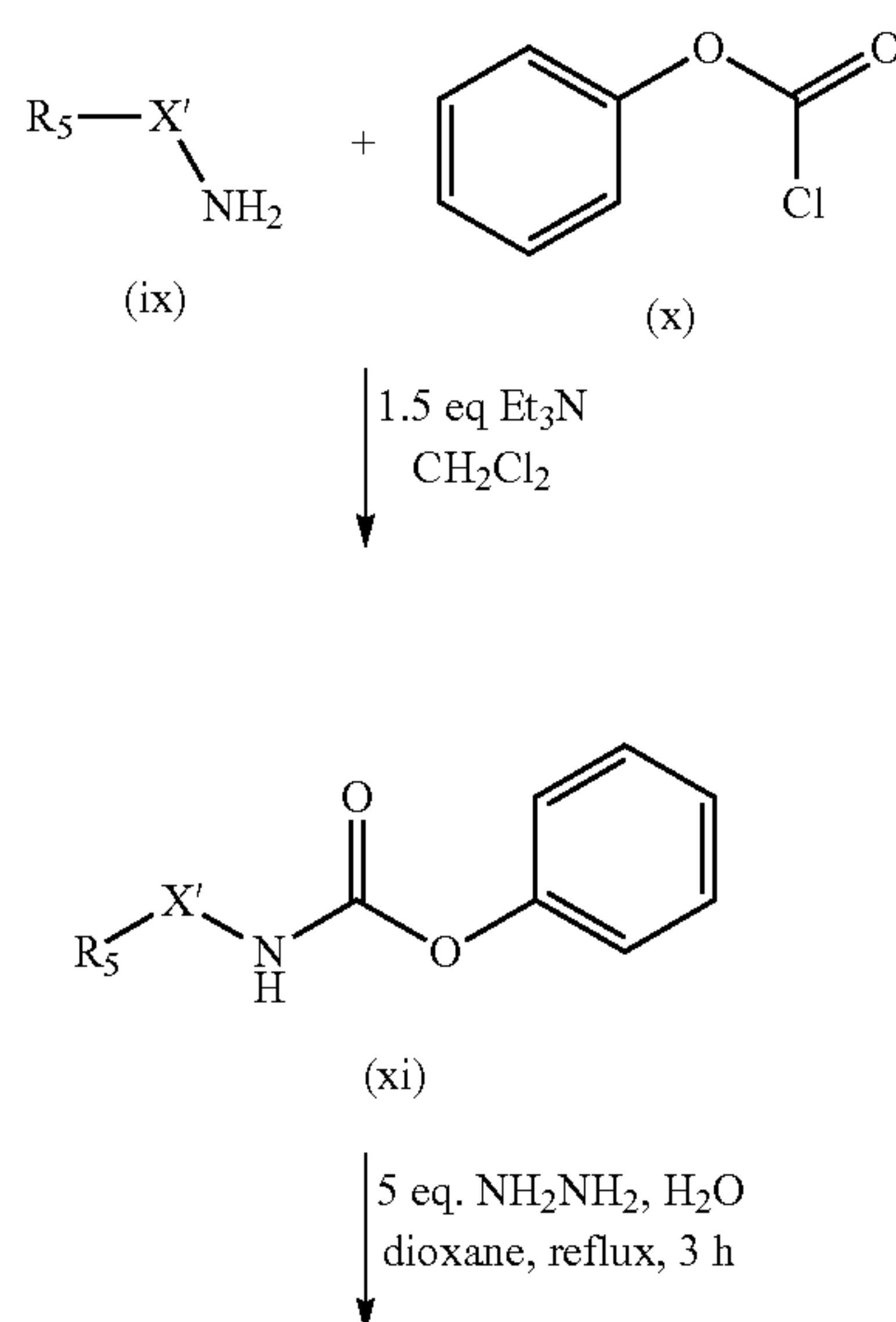
Scheme III: Alternative synthesis of triazole compounds of the invention
