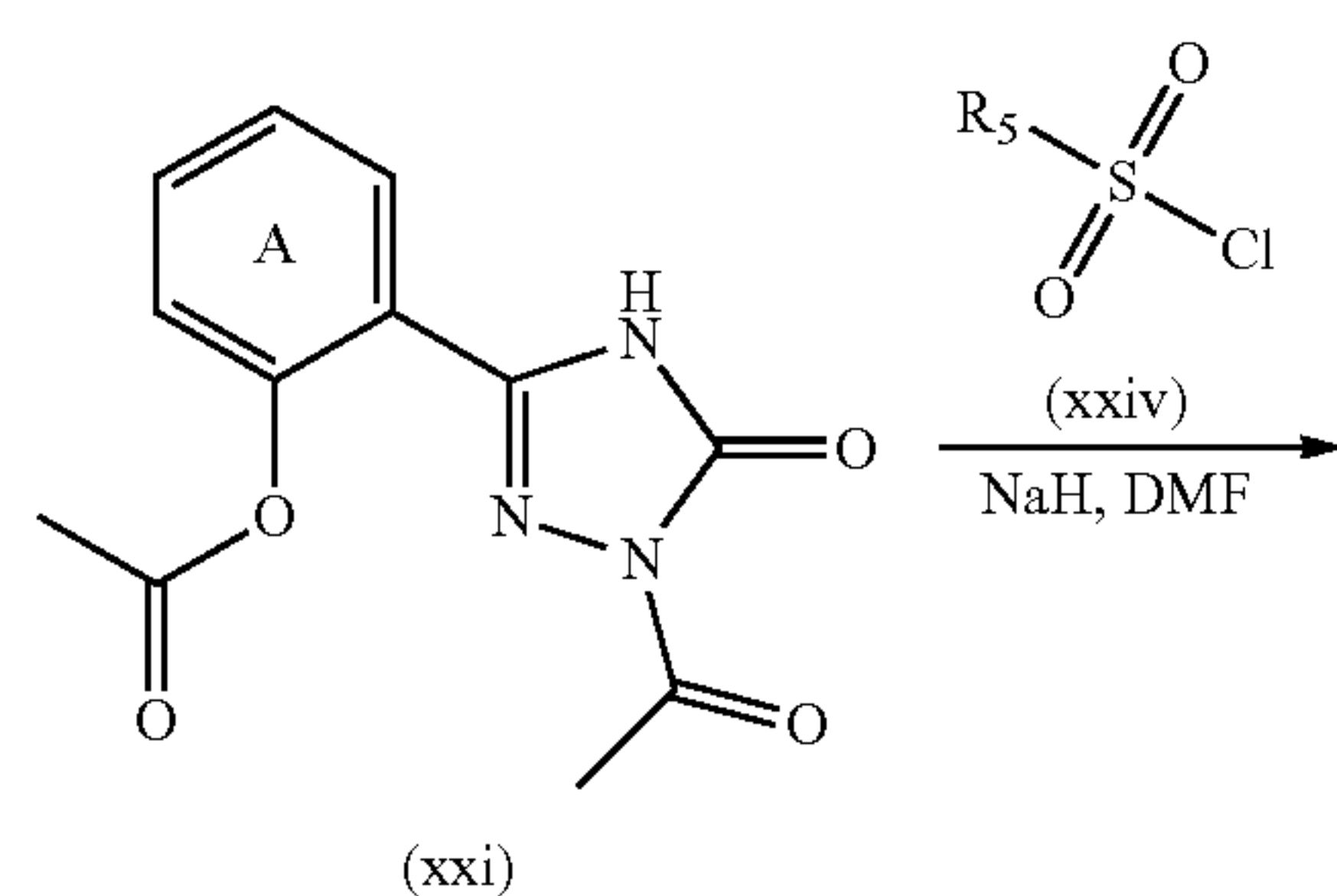
Scheme V: Synthesis of triazole compounds of the invention wherein X is S(O) 2
