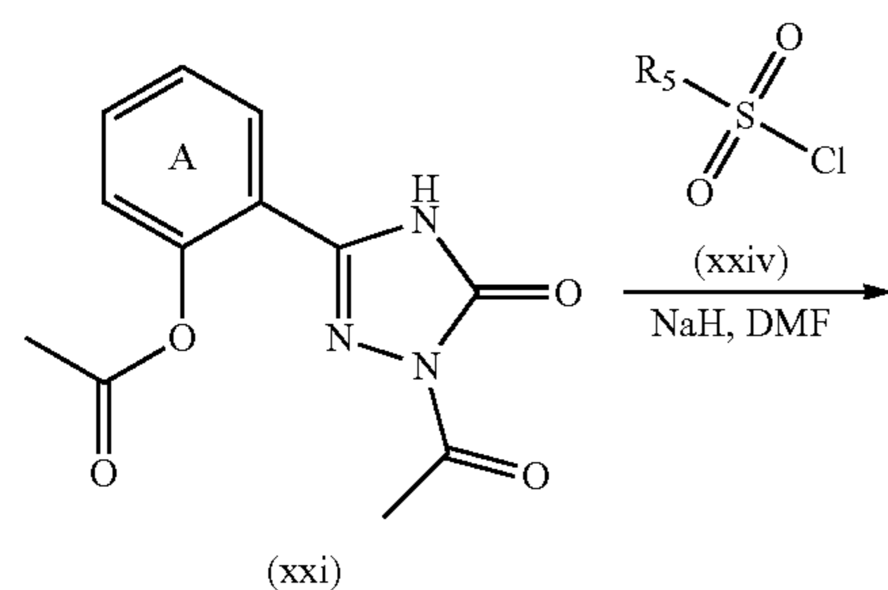
Scheme V: Synthesis of triazole compounds of the invention wherein X is \text{S}(\text{O})_2
