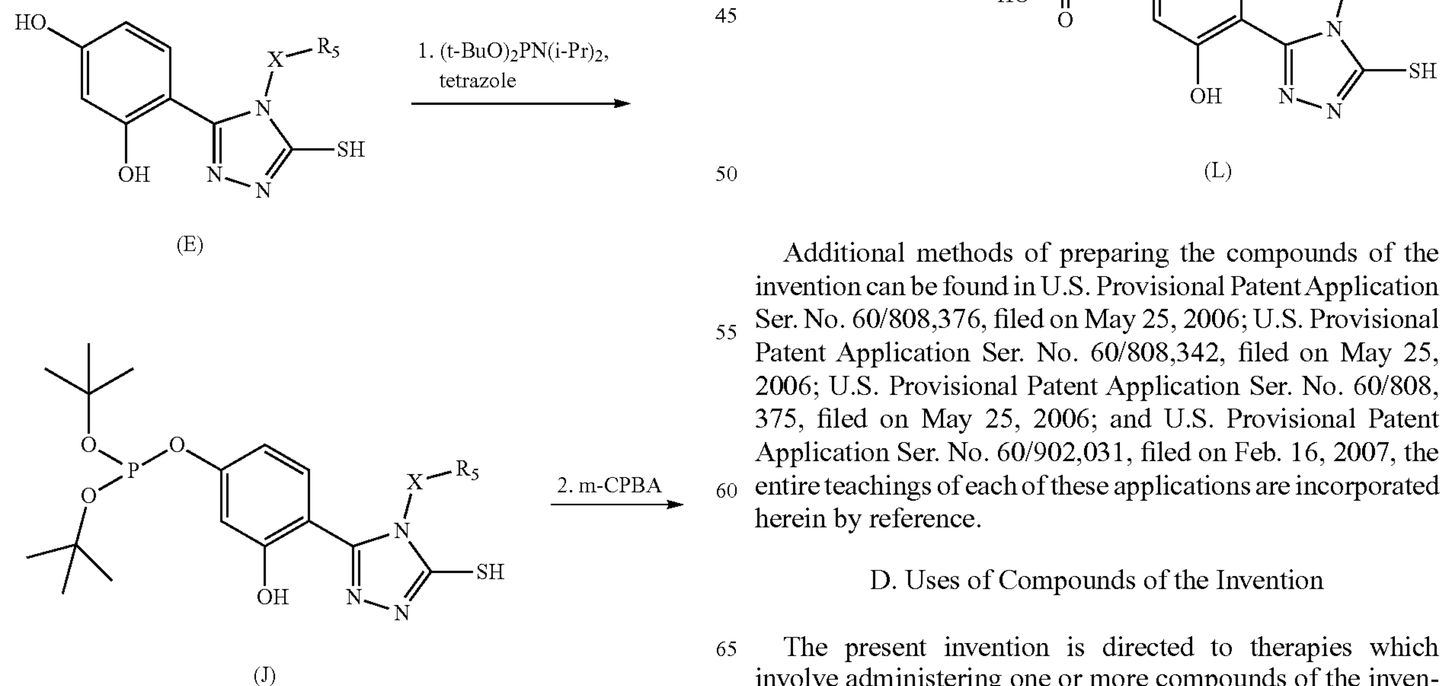
Scheme IX: Preparation of prodrugs in which the 4-hydroxy group of compounds of the invention is protected with a phosphate group.
