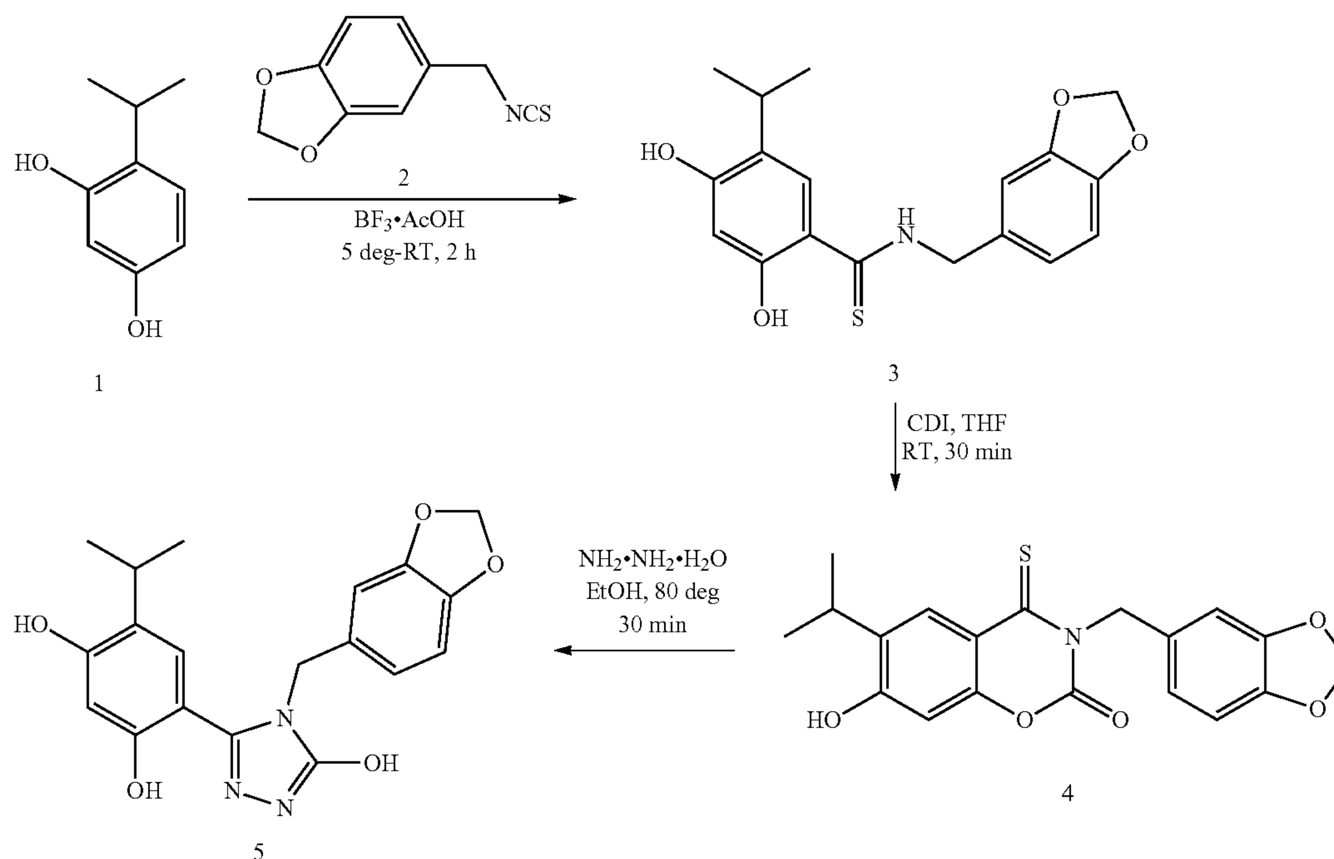
Scheme VII: Alternate Synthesis of Triazole Compounds of the Invention
