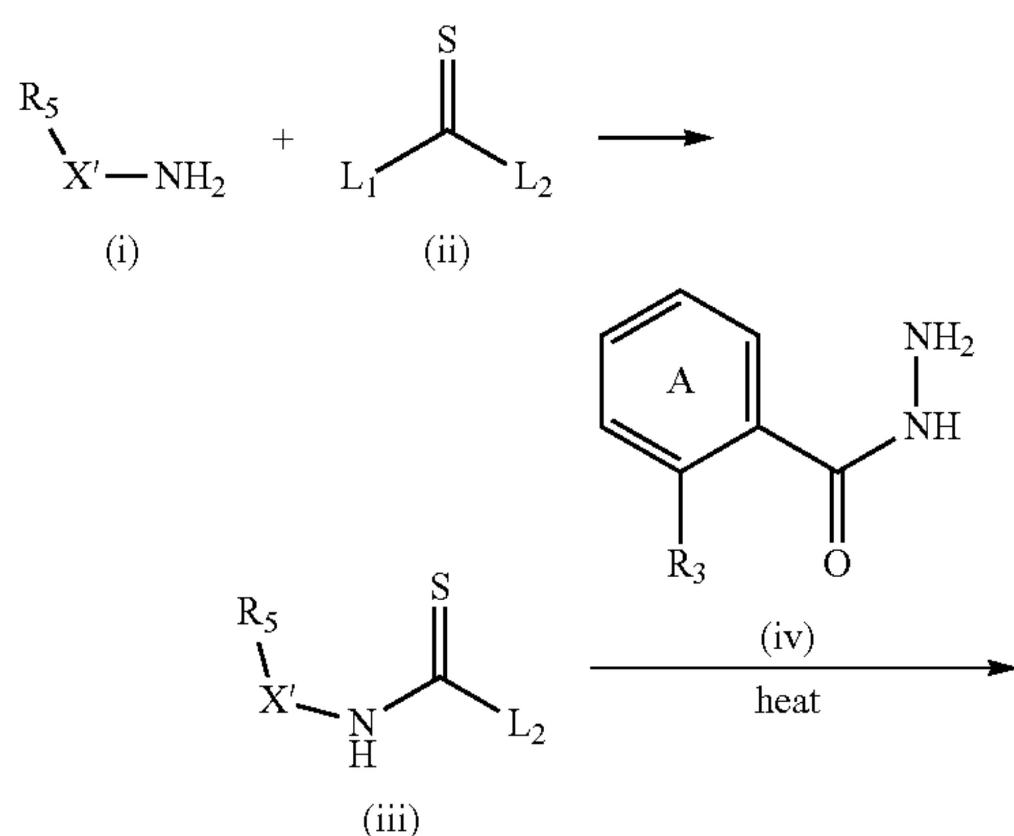
Scheme II: Alternative synthesis of triazole compounds of the invention
