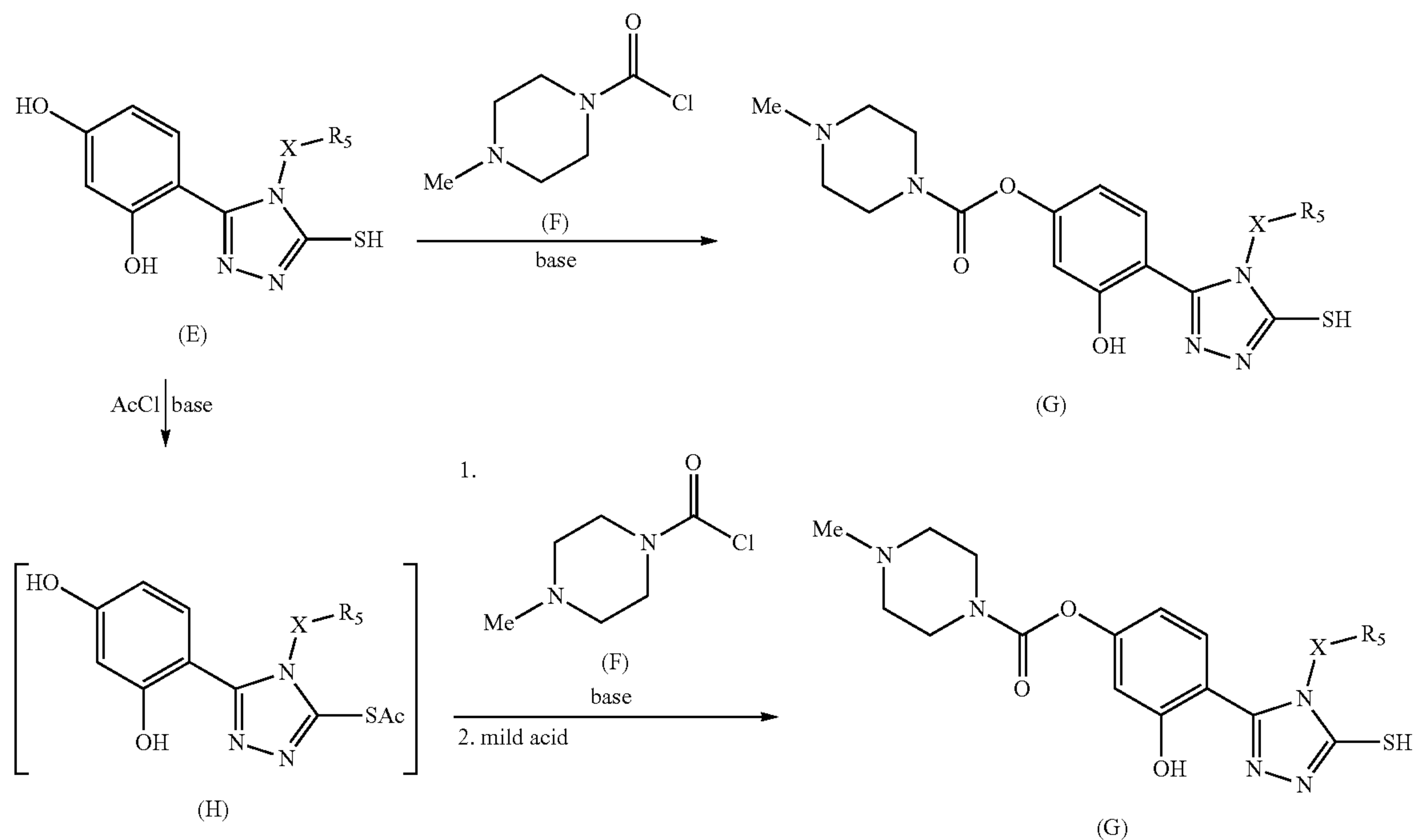
Scheme VIII: Preparation of prodrugs in which the 4-hydroxy group of compounds of the invention is protected with 4-methyl-piperazine-1-carbamoyl.
