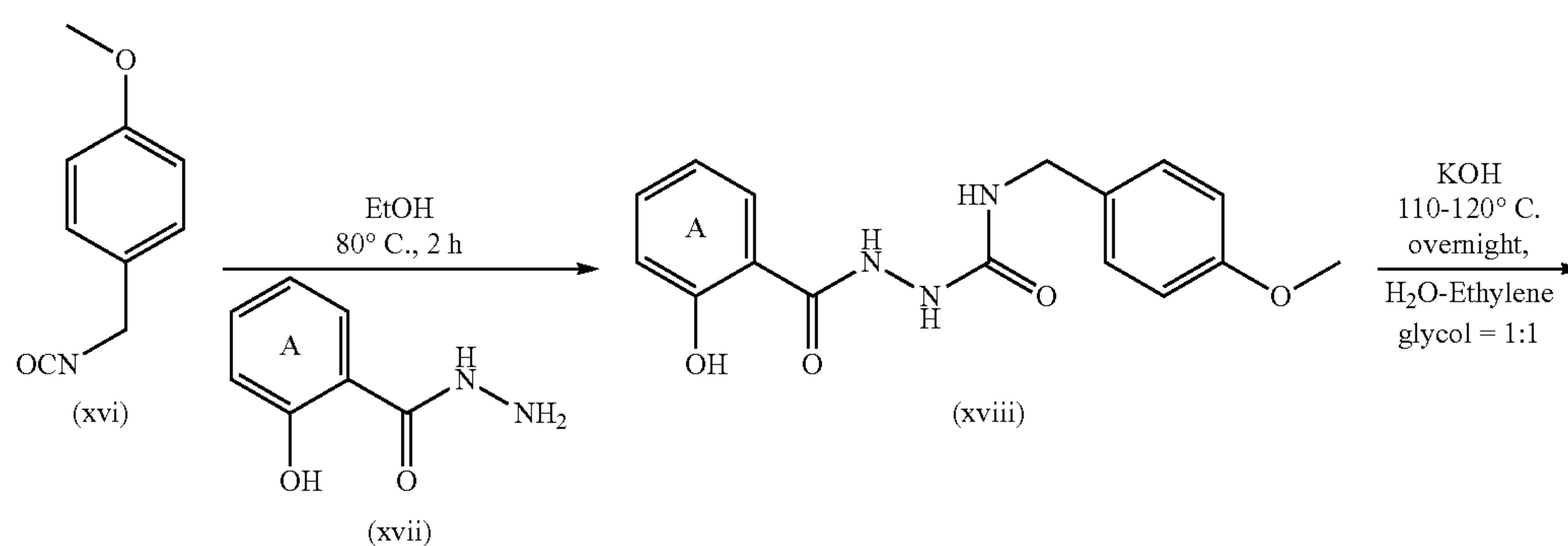
Scheme IV: Synthesis of triazole compounds of the invention wherein X is C(O)
