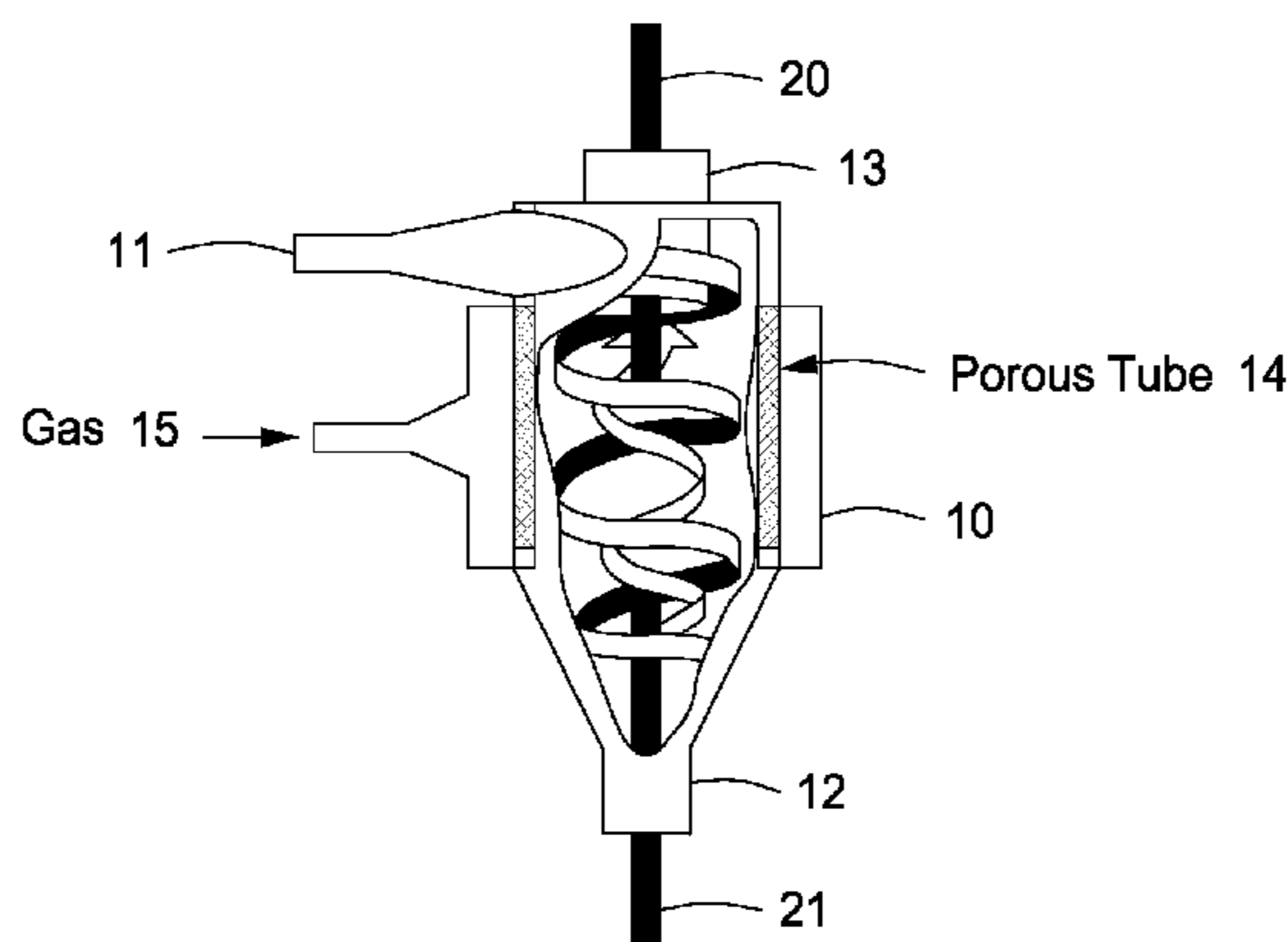
Carbon Arc in Gas-Sparged Hydrocyclone
