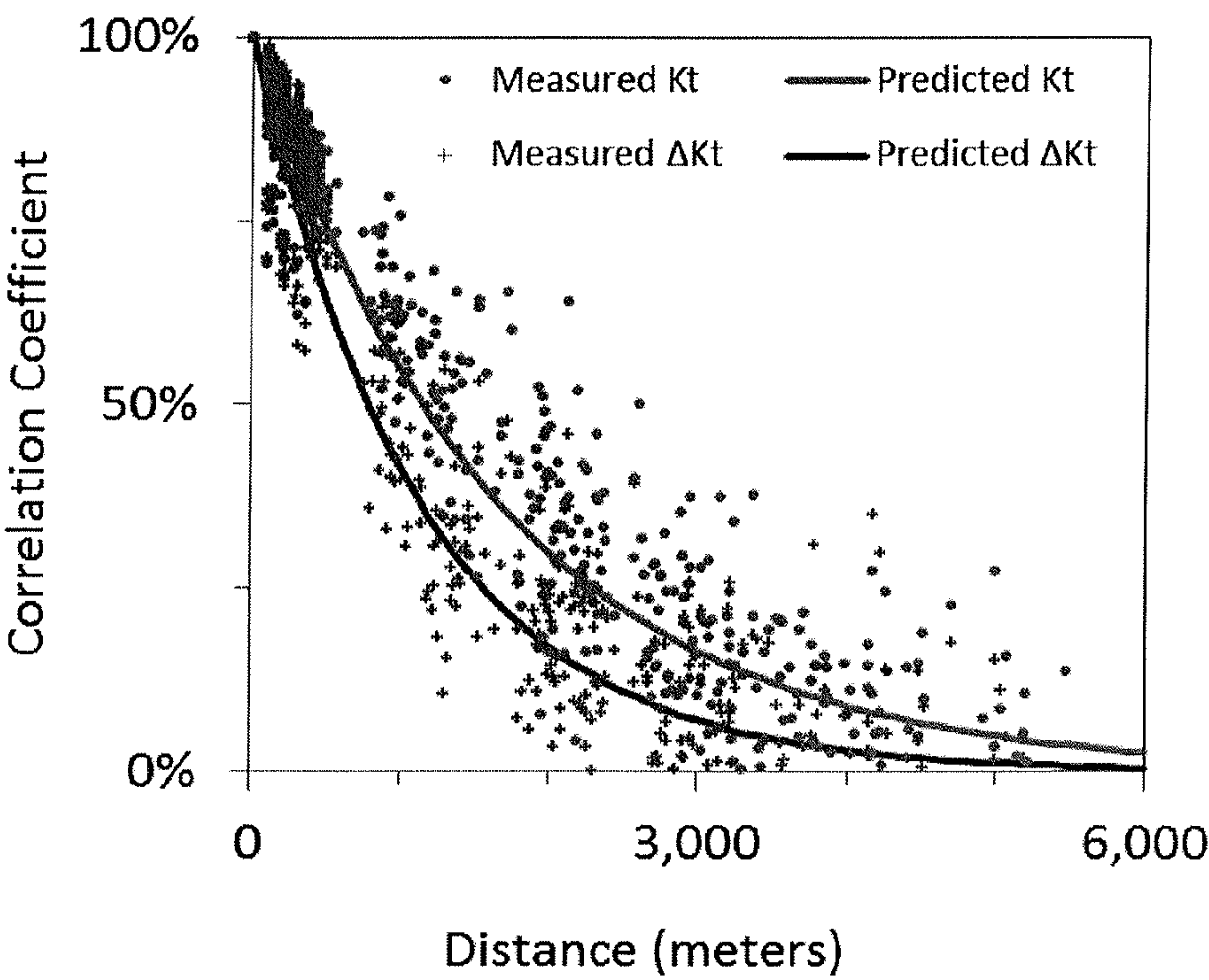
Correlation vs. Distance ( \Delta t=300 )
