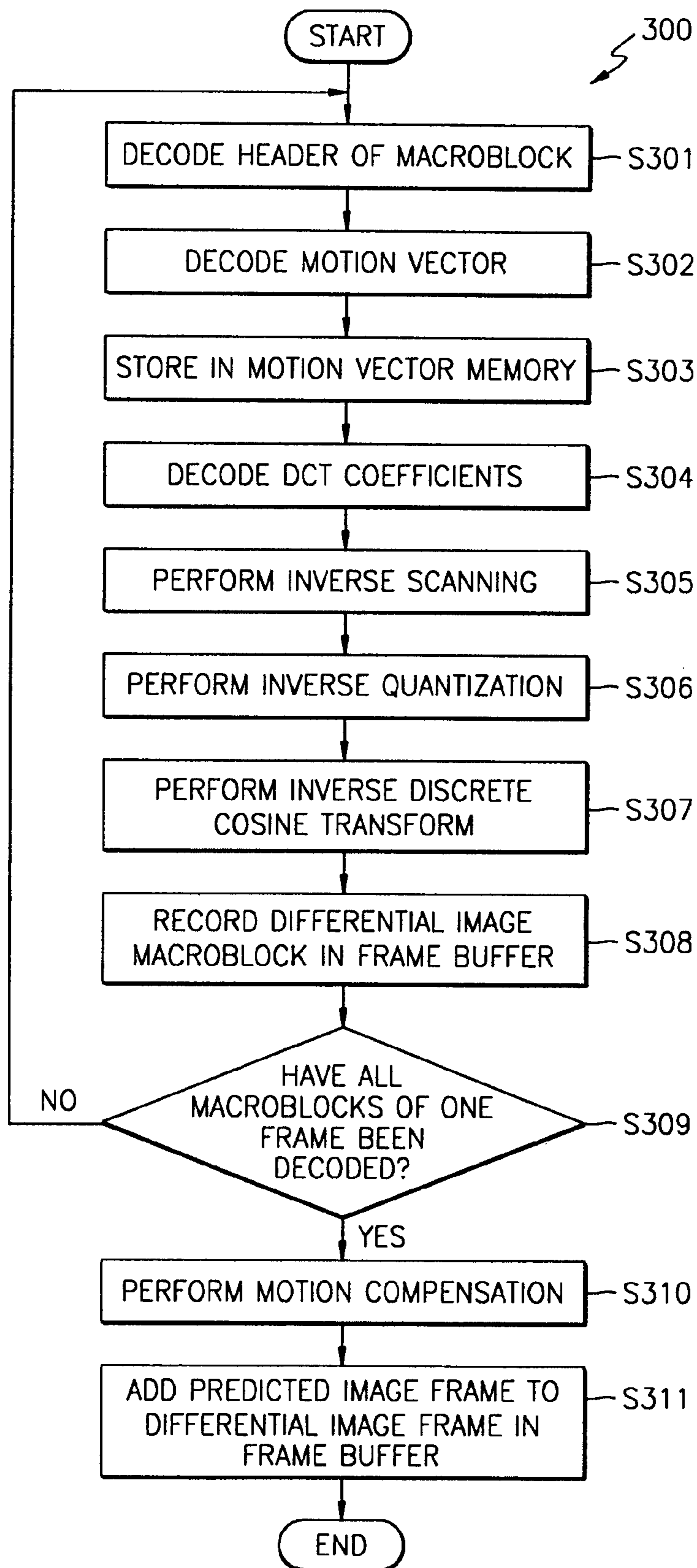
FIG. 3 (PRIOR ART)
