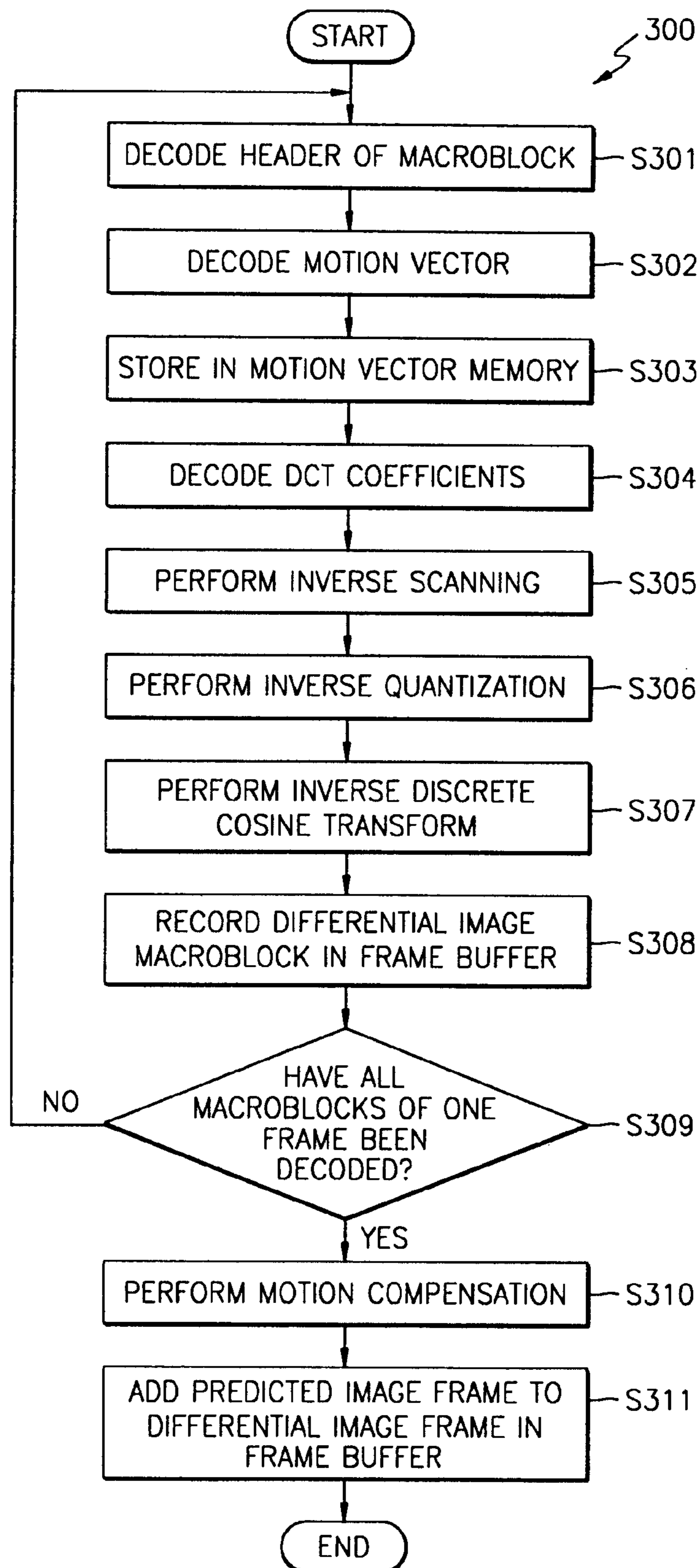
FIG. 3 (PRIOR ART)
