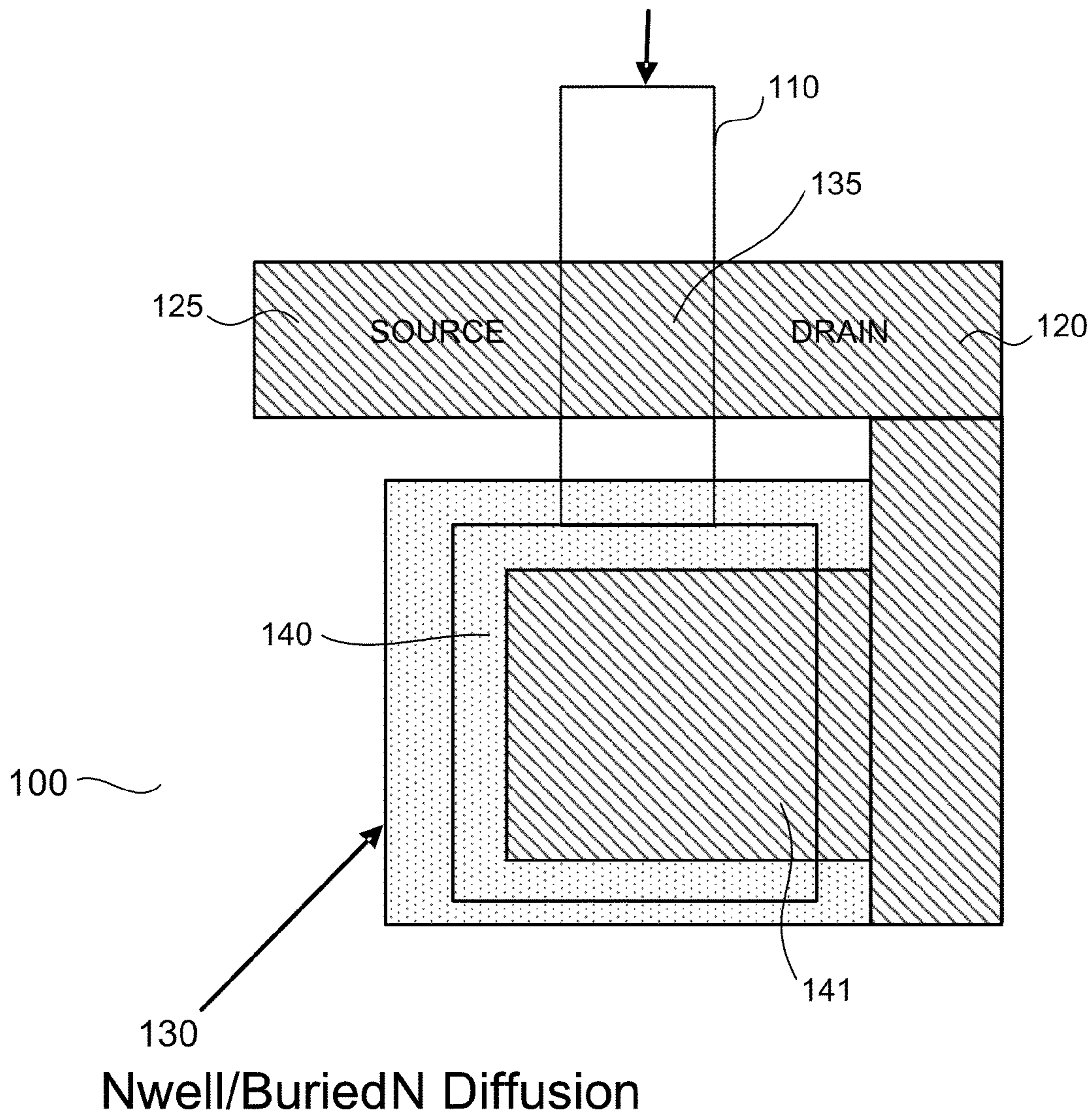
FIG. 1 Floating Gate
