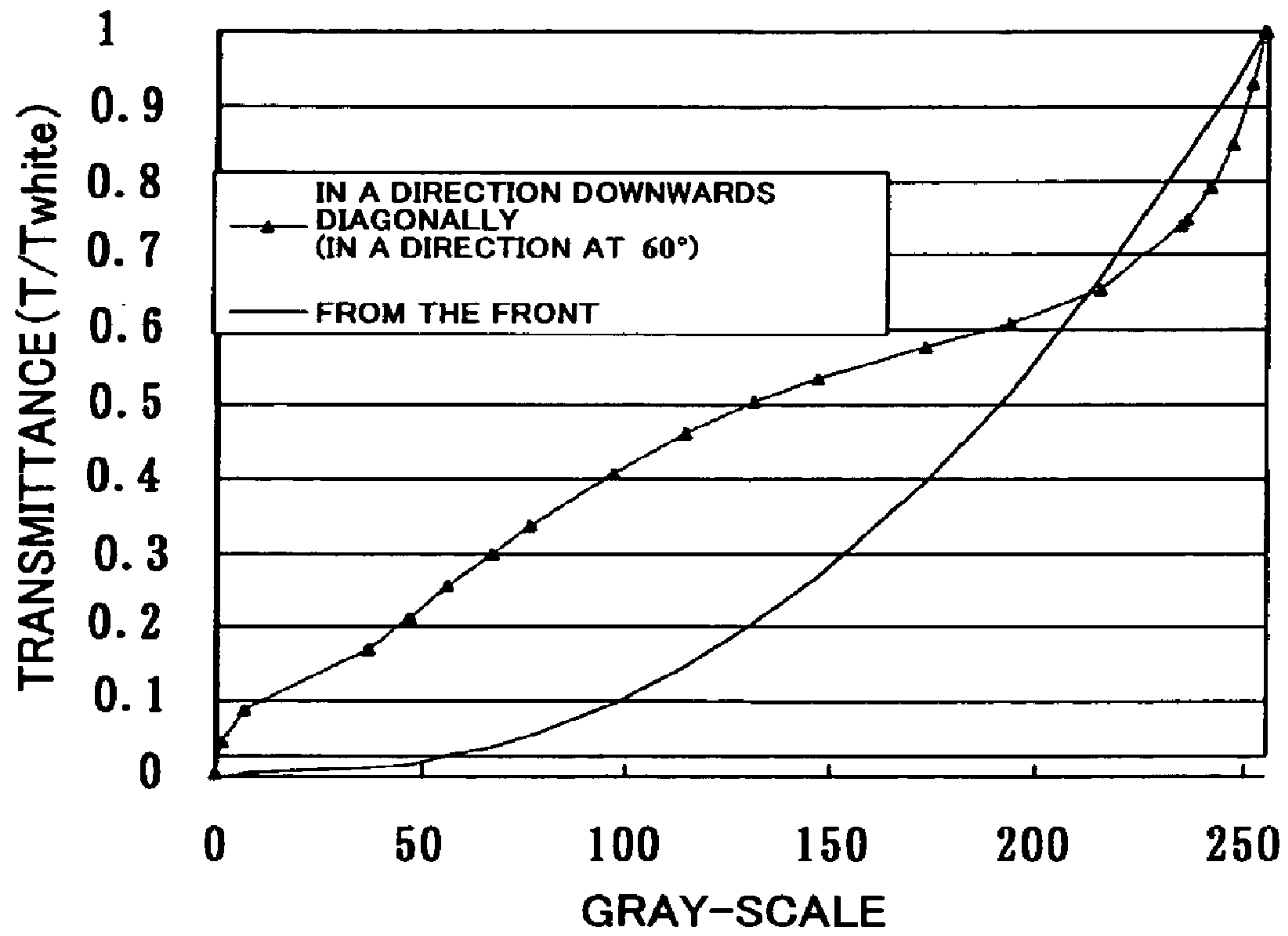
FIG. 2 (PRIOR ART)
