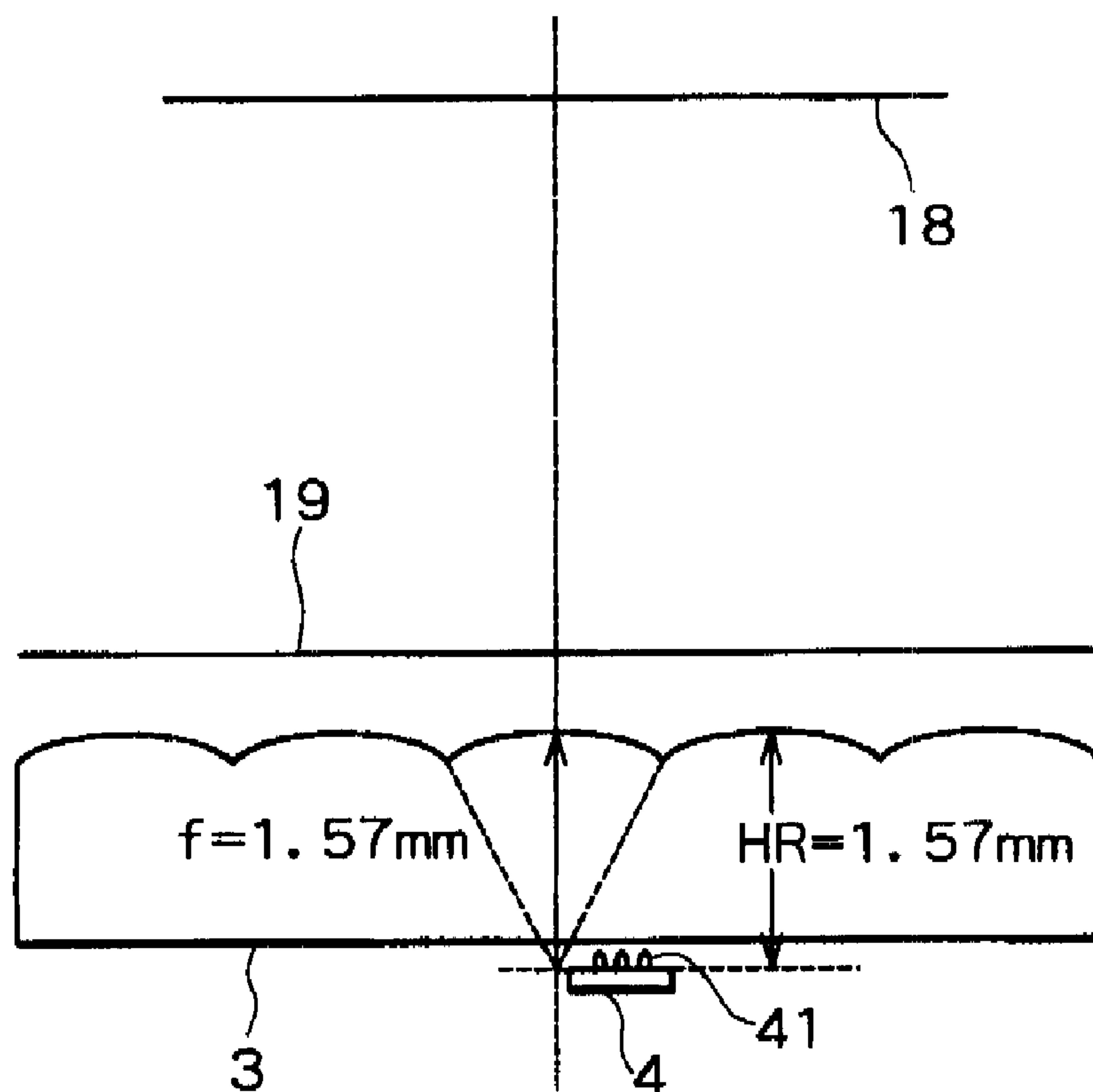
FIG. 10 (PRIOR ART)
