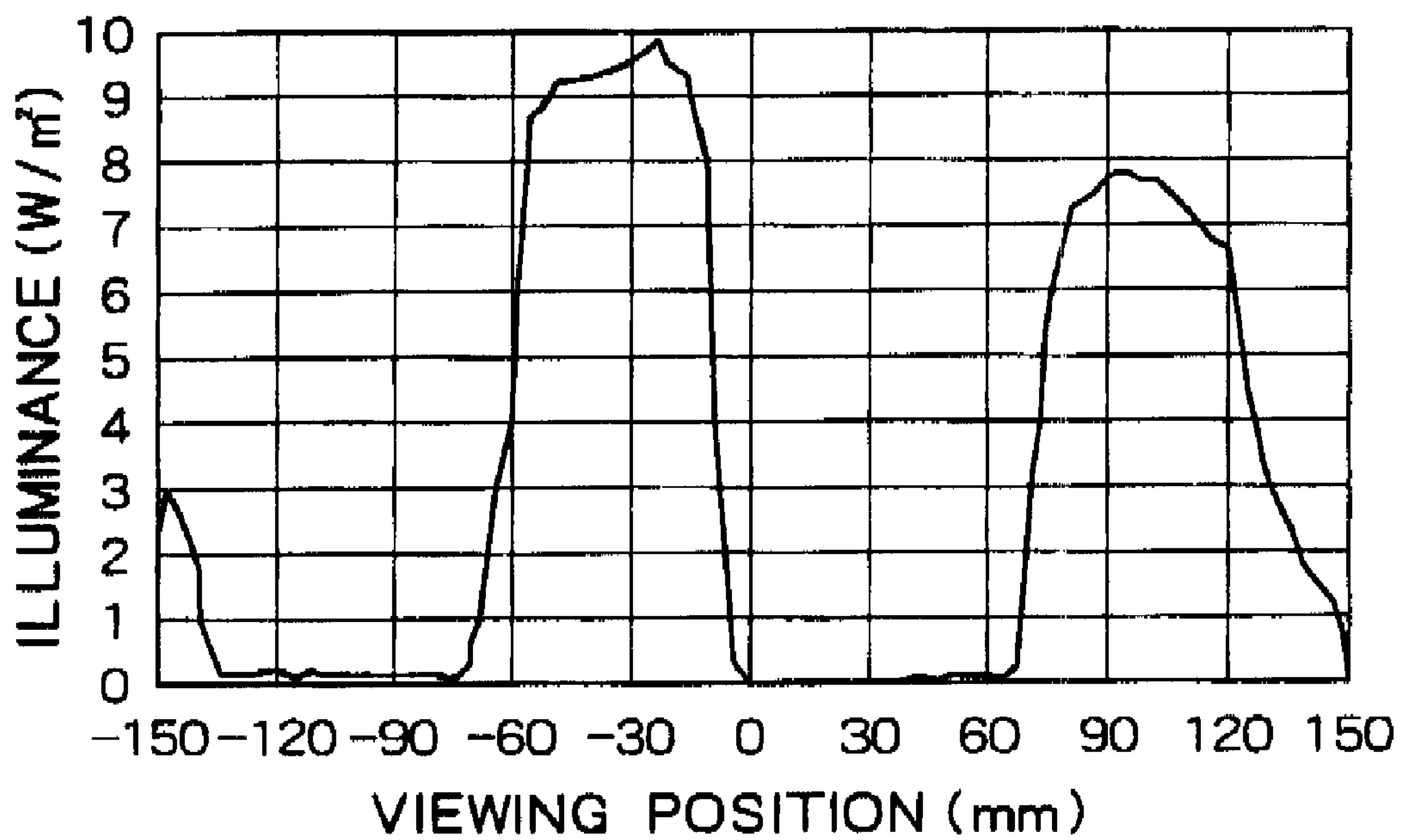
FIG. 9 (PRIOR ART)
