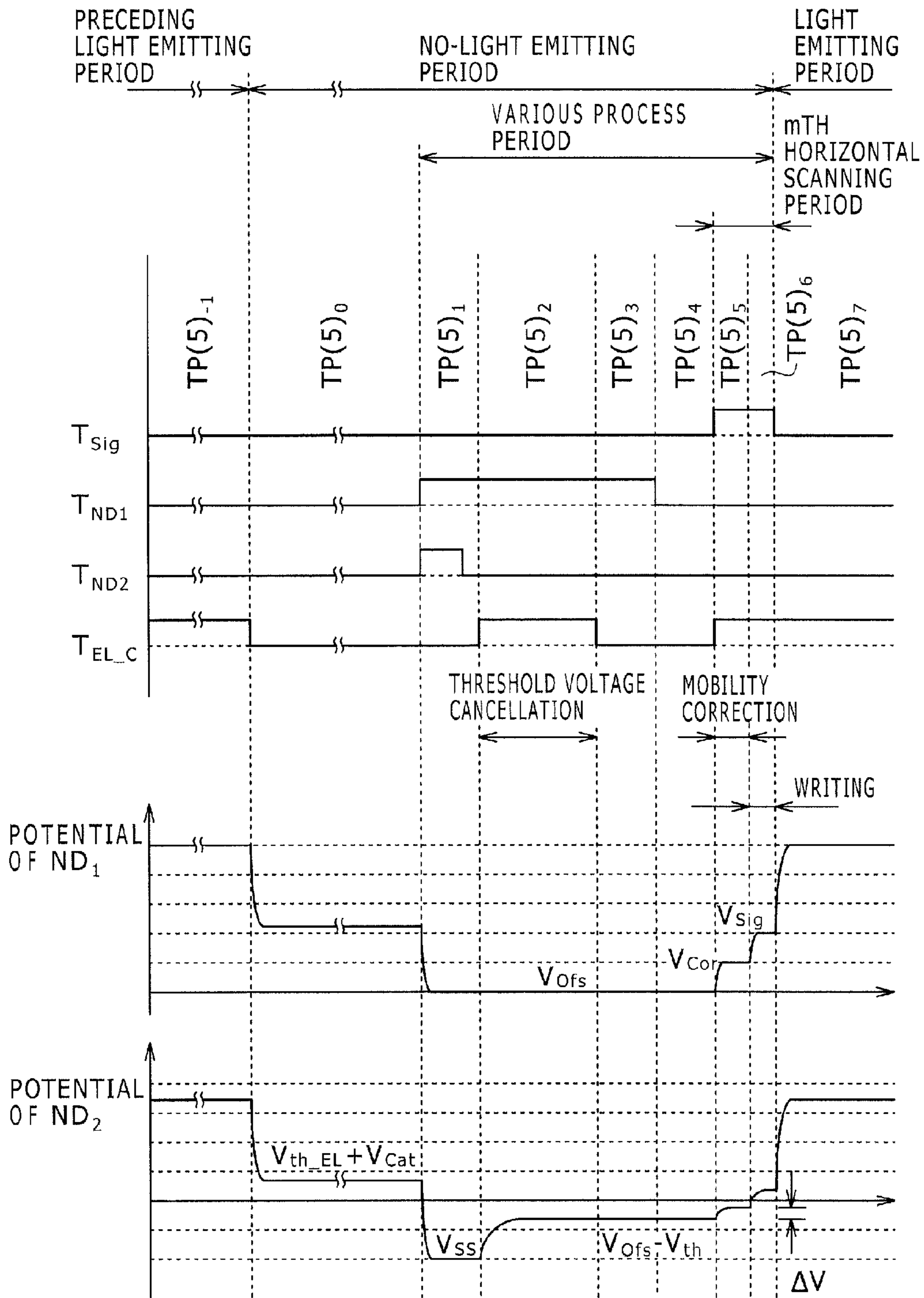
FIG. 3 [5Tr/1C DRIVING CIRCUIT]
