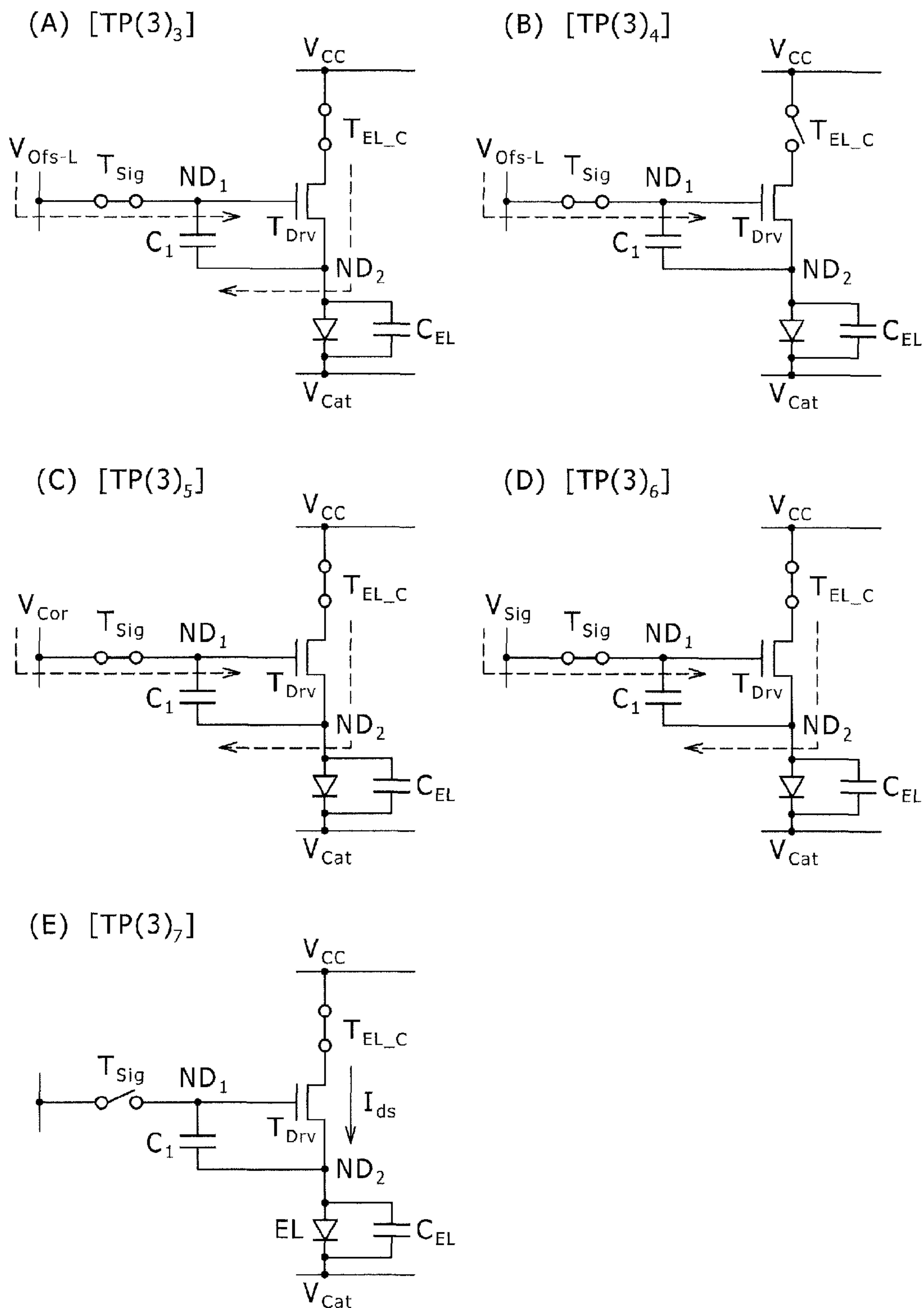
FIG. 16 [3Tr/1C DRIVING CIRCUIT]
