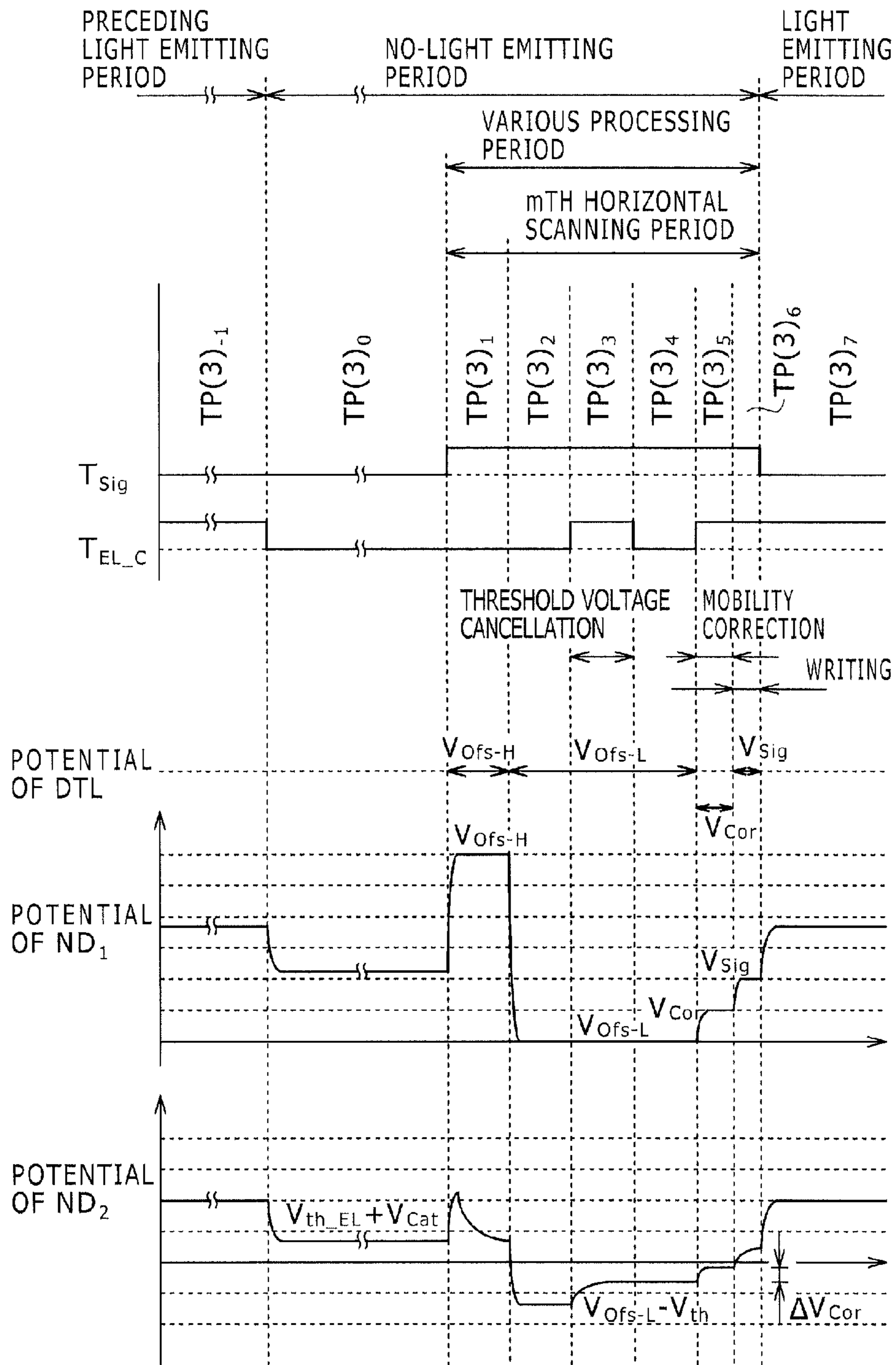
FIG. 14 [3Tr/1C DRIVING CIRCUIT]
