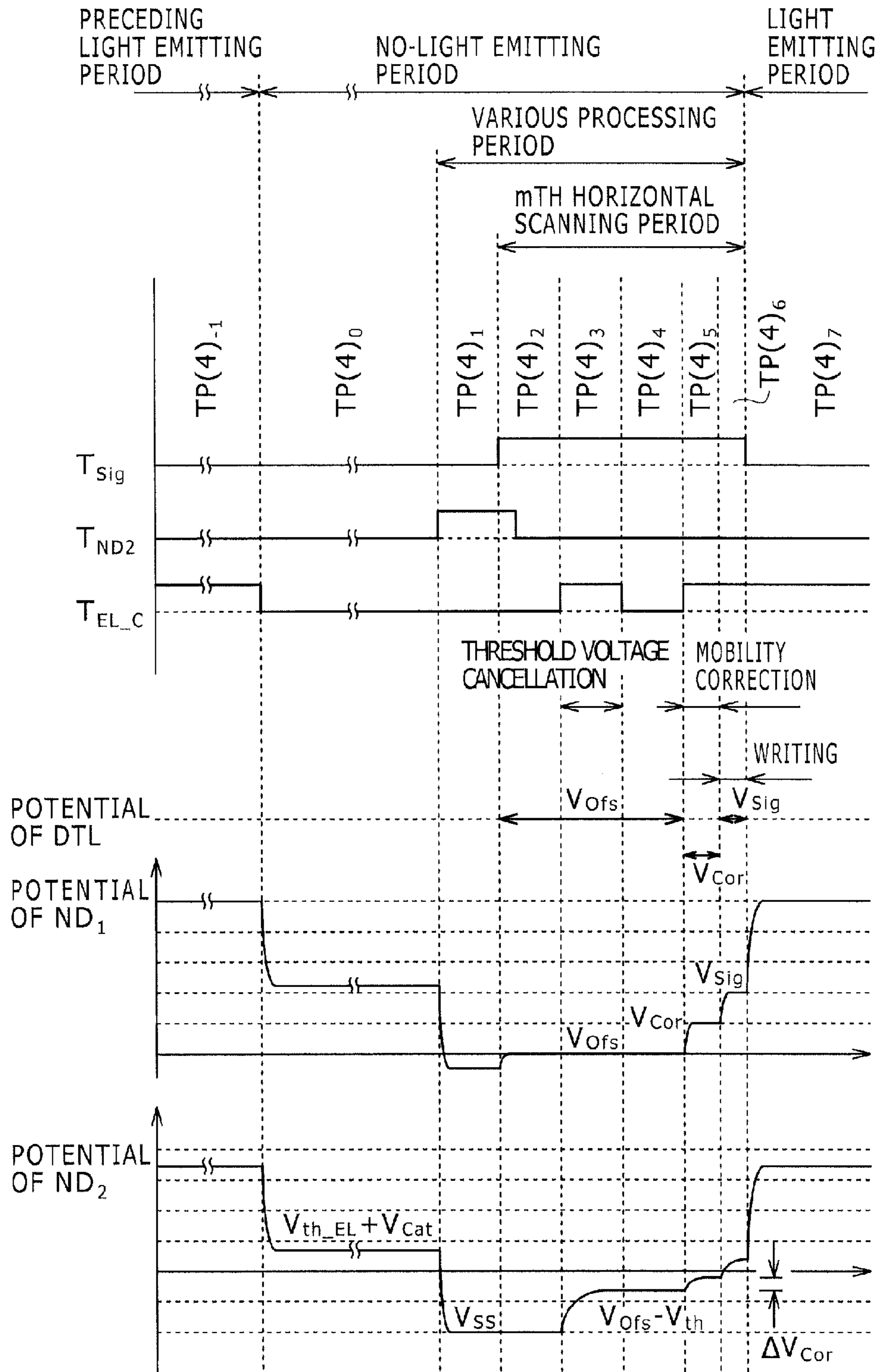
FIG. 9 [4Tr/1C DRIVING CIRCUIT]
